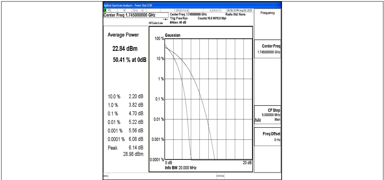
Band4-20MHz-QPSK-20300-100RB#0-PASS
