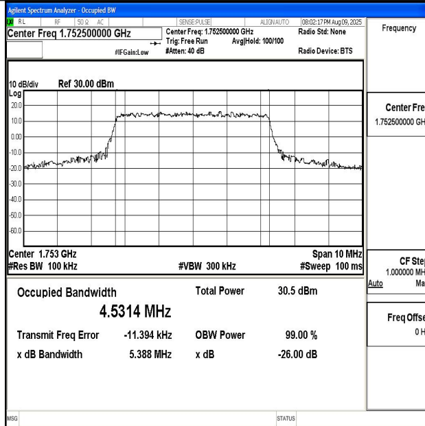
Band4-5MHz-QPSK-20375-25RB#0-PASS
