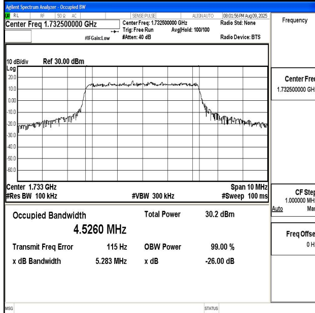
Band4-5MHz-16QAM-20175-25RB#0-PASS
