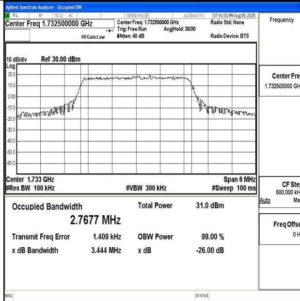
Band4-3MHz-QPSK-20175-15RB#0-PASS
