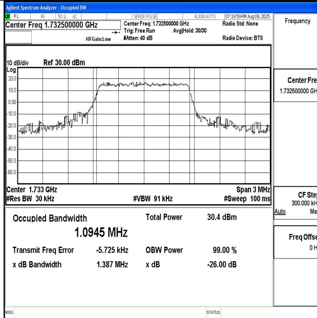
Band4-1.4MHz-QPSK-20175-6RB#0-PASS
