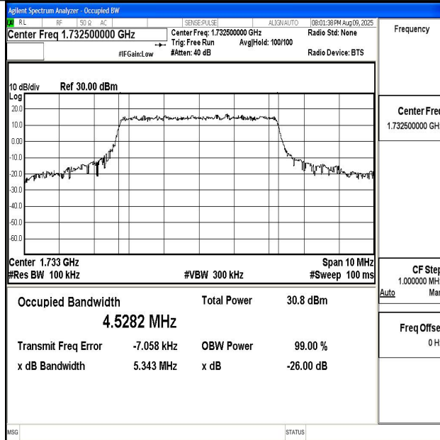
Band4-5MHz-QPSK-20175-25RB#0-PASS
