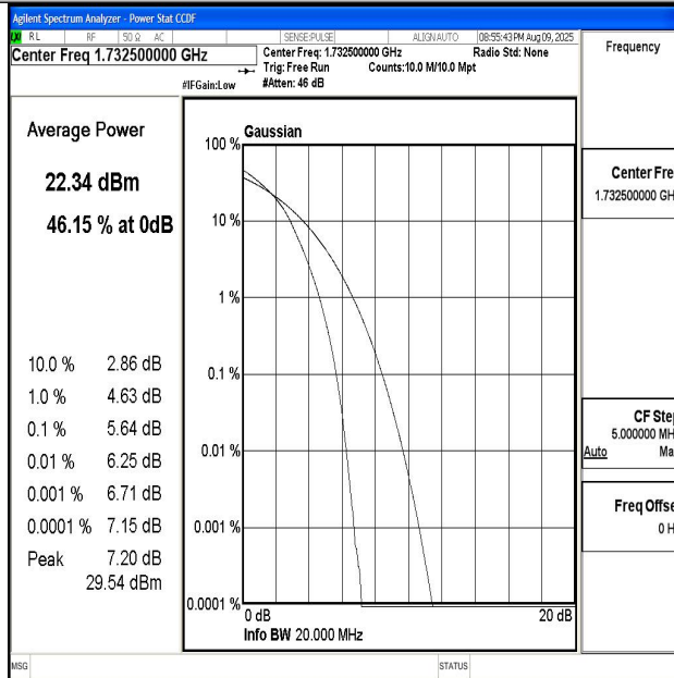
Band4-20MHz-16QAM-20175-100RB#0-PASS
