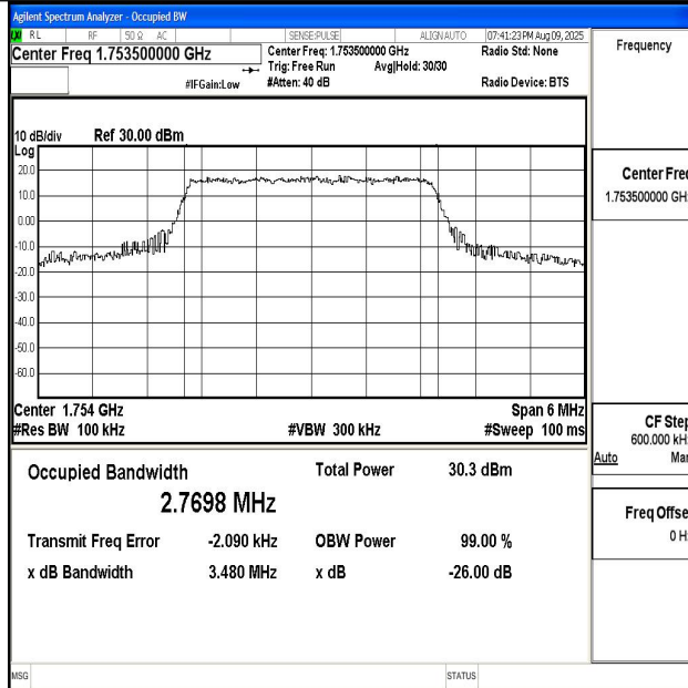
Band4-3MHz-QPSK-20385-15RB#0-PASS
