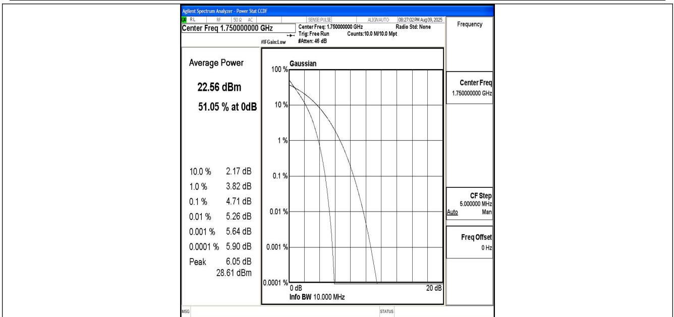
Band4-10MHz-QPSK-20350-50RB#0-PASS
