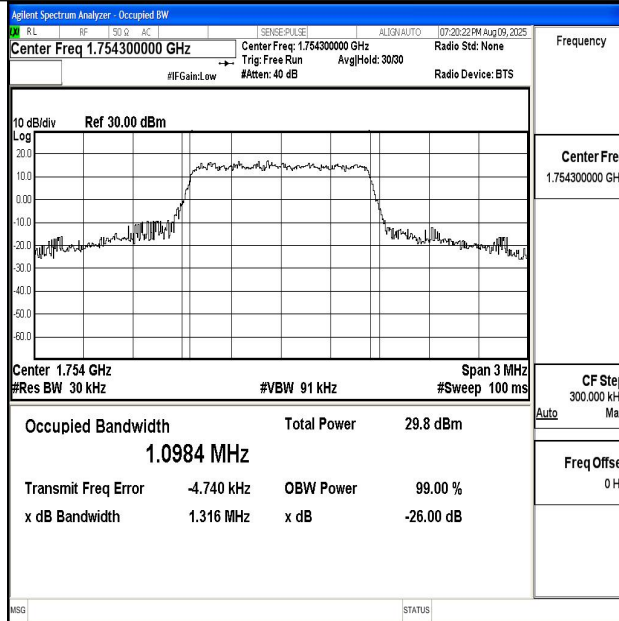
Band4-1.4MHz-QPSK-20393-6RB#0-PASS
