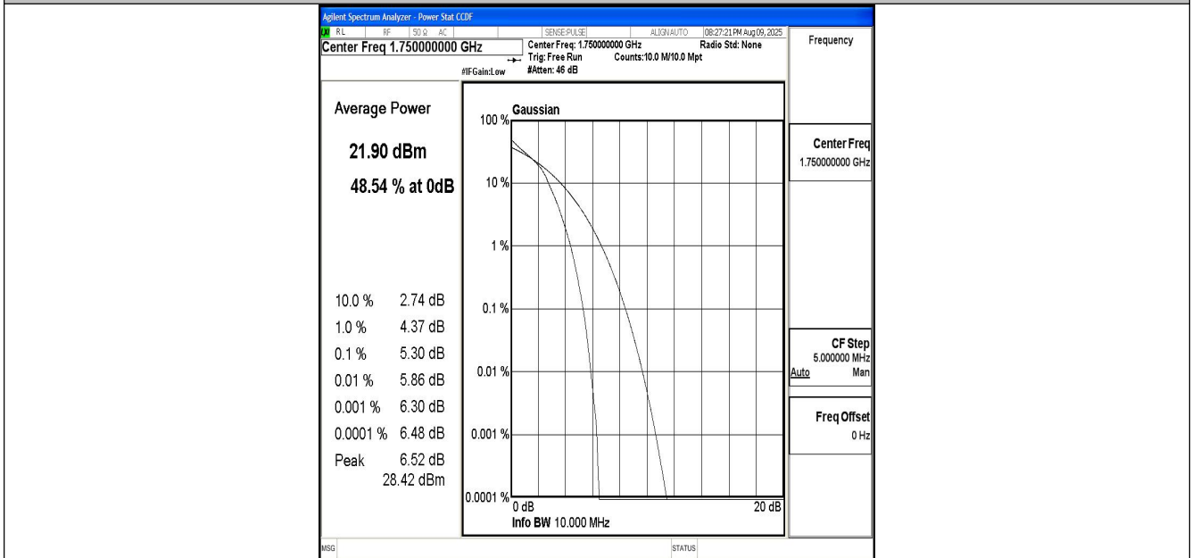
Band4-10MHz-16QAM-20350-50RB#0-PASS
