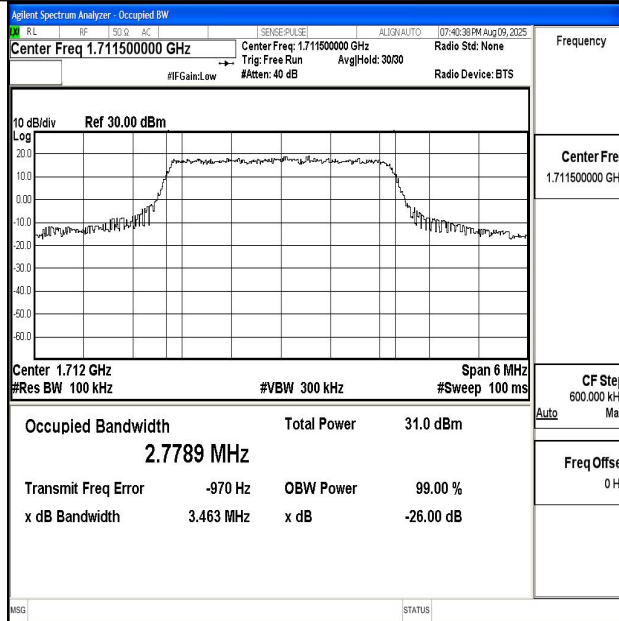
Band4-3MHz-QPSK-19965-15RB#0-PASS
