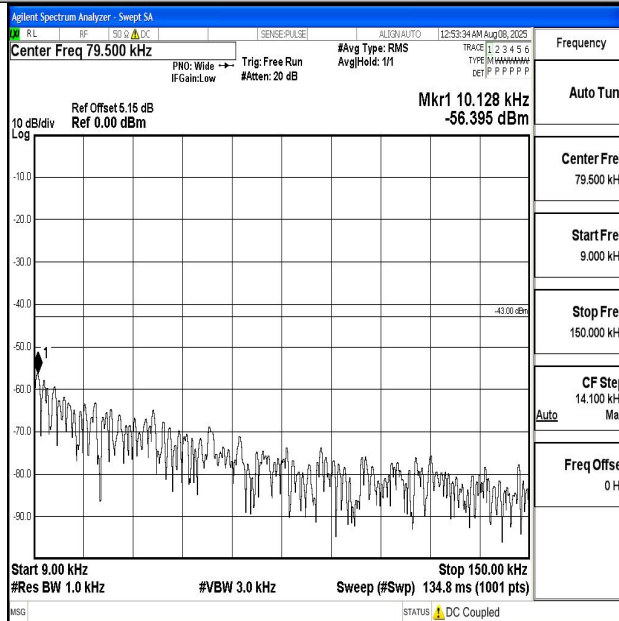
Band2_10MHz_16QAM_18900_1RB#0_0.009~0.15_0.009~0.15
