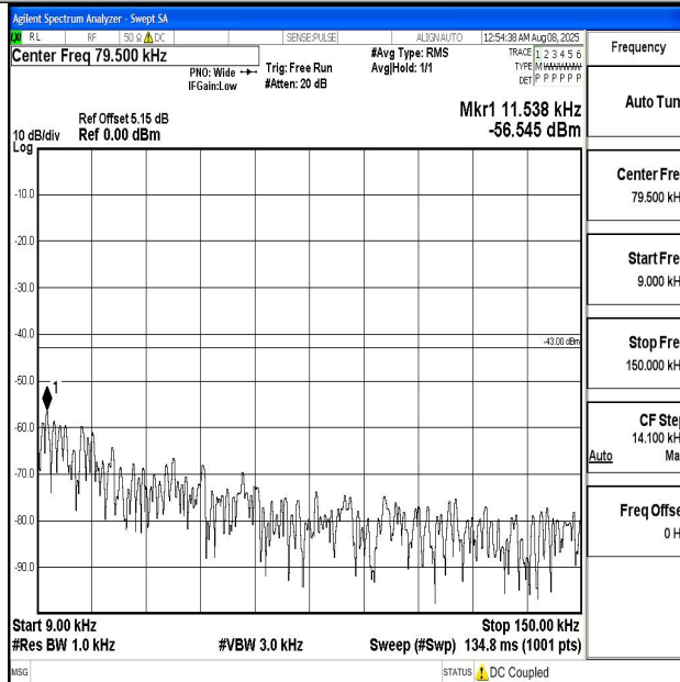
Band2_10MHz_16QAM_19150_1RB#0_0.009~0.15_0.009~0.15
