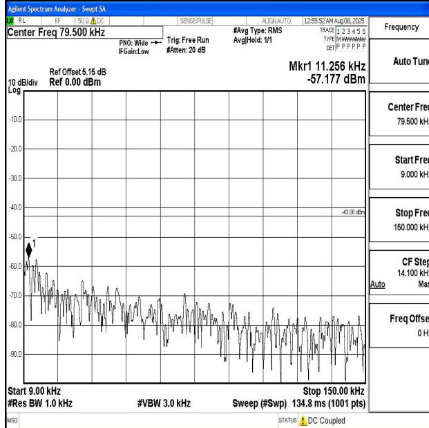
Band2_15MHz_QPSK_18675_1RB#0_0.009~0.15_0.009~0.15
