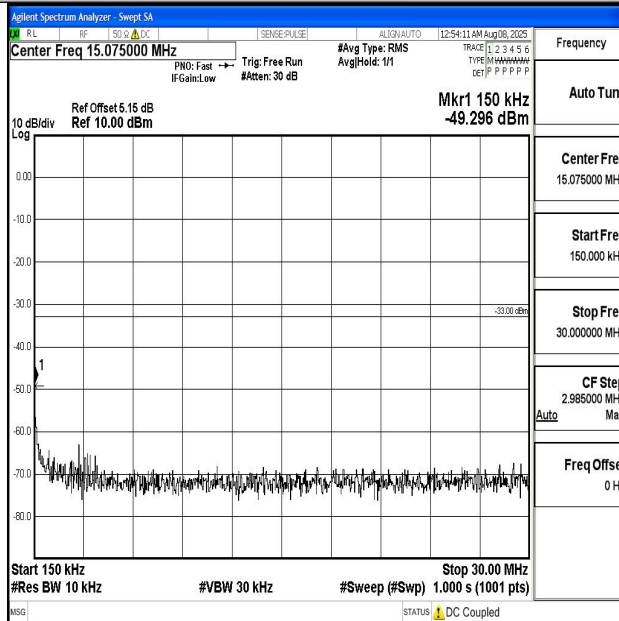
Band2_10MHz_QPSK_19150_1RB#0_0.15~30_0.15~30
