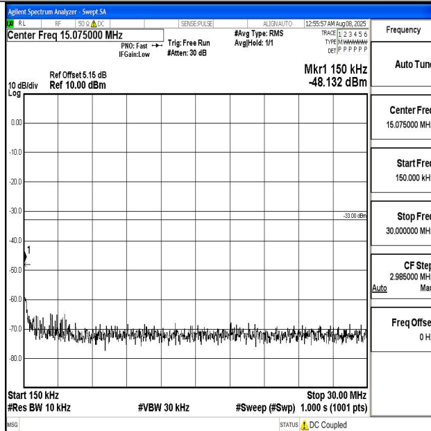
Band2_15MHz_QPSK_18675_1RB#0_0.15~30_0.15~30
