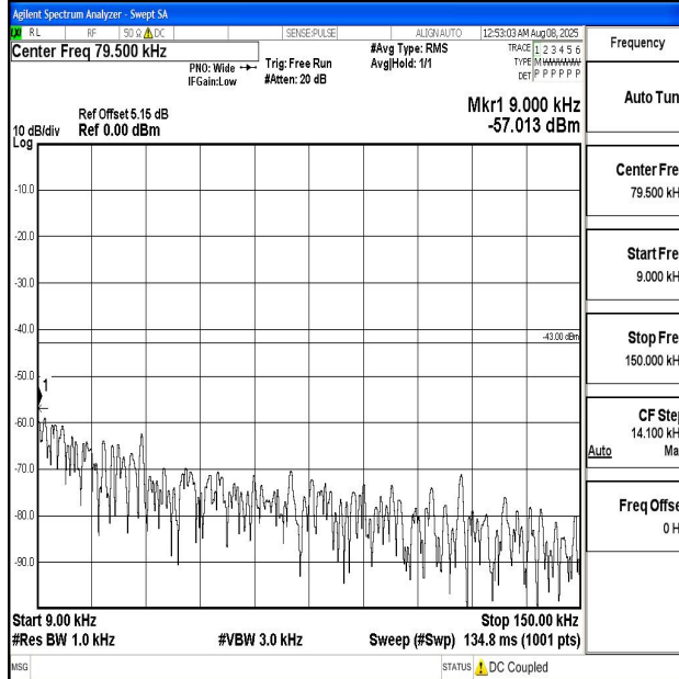
Band2_10MHz_QPSK_18900_1RB#0_0.009~0.15_0.009~0.15
