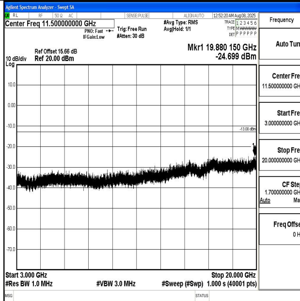
Band2_10MHz_QPSK_18650_1RB#0_3000~20000_3000~20000
