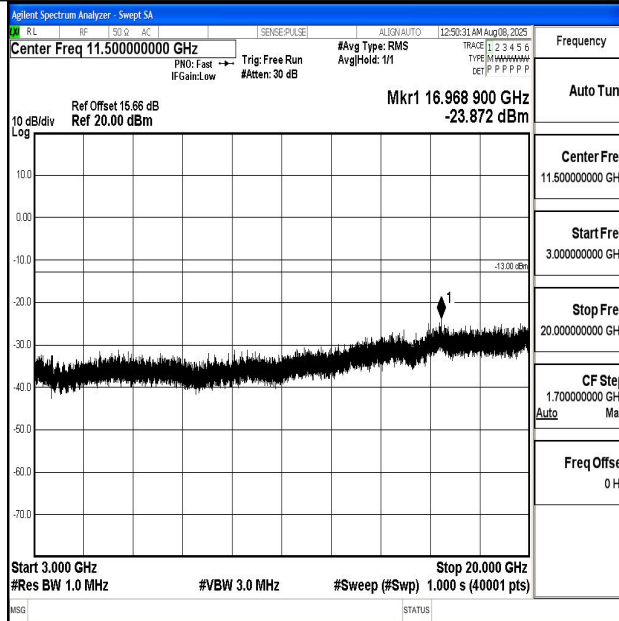
Band2_5MHz_QPSK_19175_1RB#0_3000~20000_3000~20000
