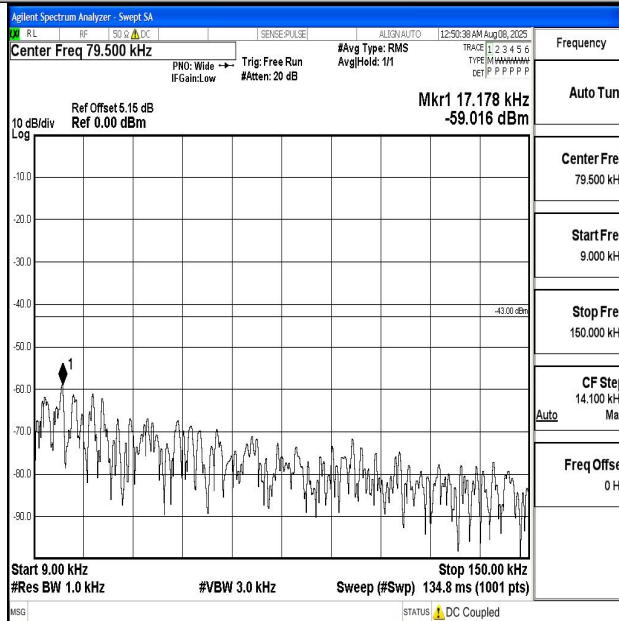
Band2_5MHz_16QAM_19175_1RB#0_0.009~0.15_0.009~0.15
