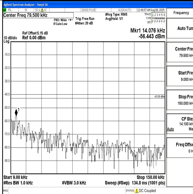
Band2_5MHz_QPSK_18900_1RB#0_0.009~0.15_0.009~0.15
