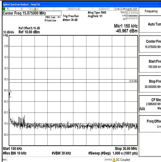
Band2_3MHz_QPSK_19185_1RB#0_0.15~30_0.15~30
