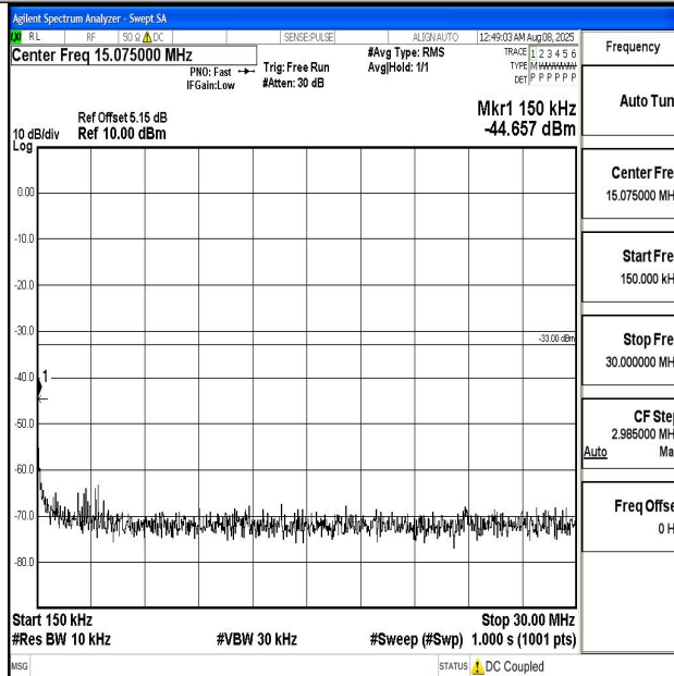
Band2_5MHz_QPSK_18900_1RB#0_0.15~30_0.15~30
