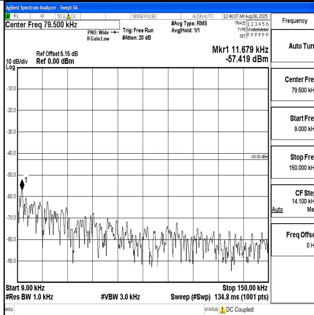
Band2_3MHz_QPSK_19185_1RB#0_0.009~0.15_0.009~0.15
