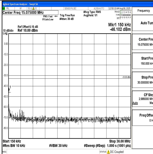
Band2_5MHz_QPSK_19175_1RB#0_0.15~30_0.15~30
