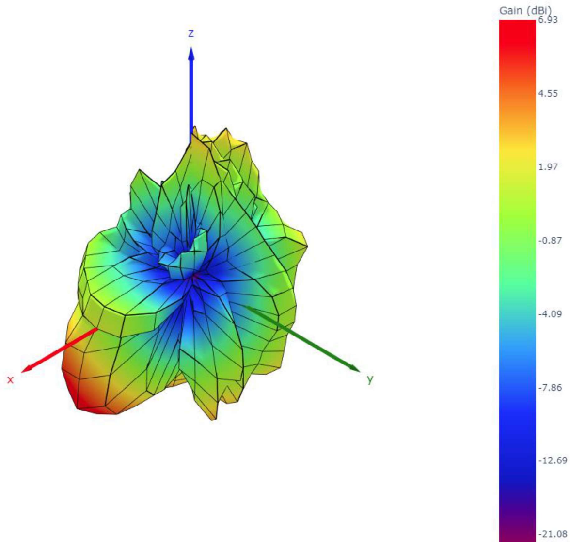
UWB1-6.5GHz-Horizontal-3D
