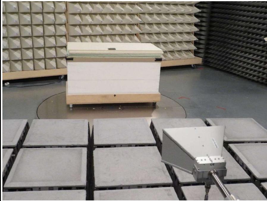
EUT SETUP 1 GHz to 17 GHZ CONFIGURATION 1
