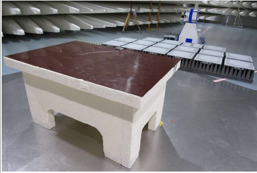
EUT SETUP 26.5 GHz to 40 GHZ CONFIGURATION 2
