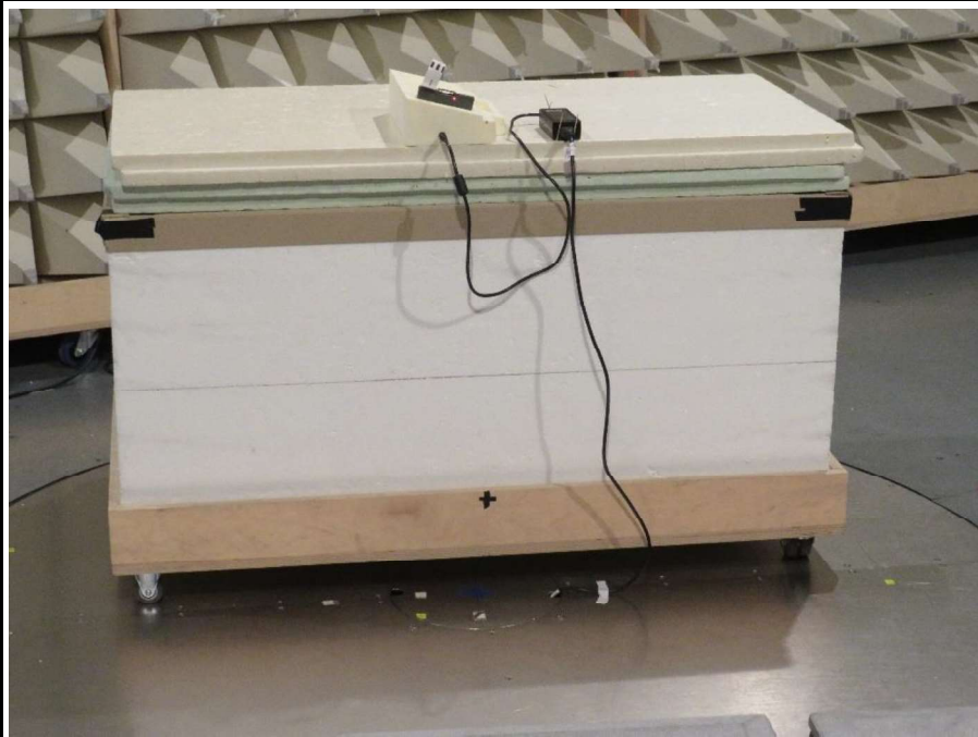
EUT SETUP 1 GHz to 17 GHZ CONFIGURATION 2
