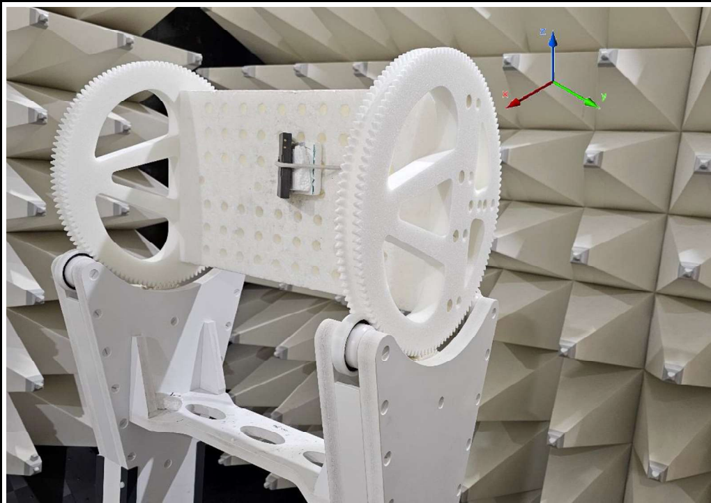
Test setup - Antenna position to the axis - Measuring antenna vertical
