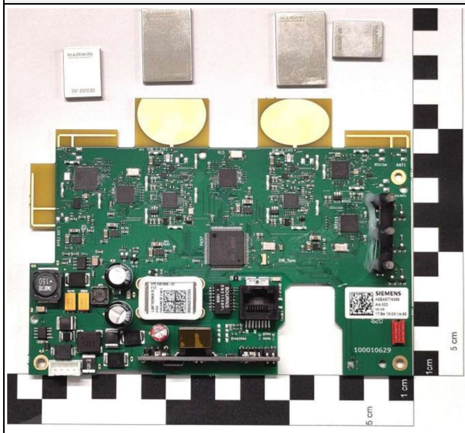
PCB Top without shielding
