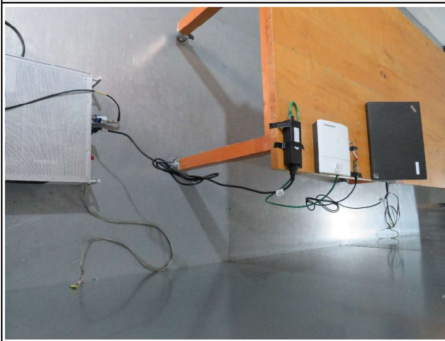
Setup for measurements with PoE
