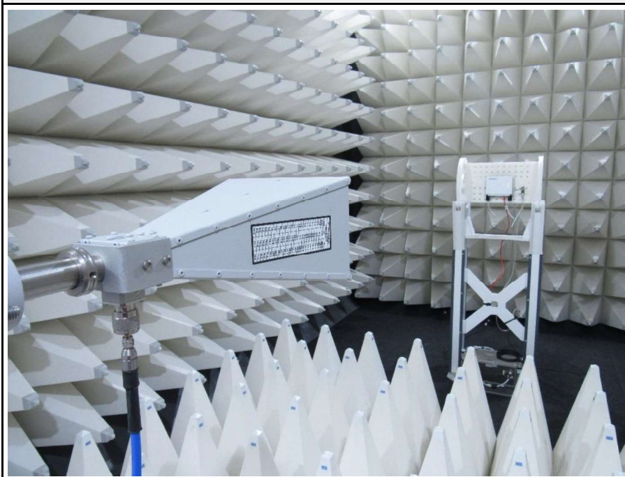
Setup 4.8 to 40 GHz
