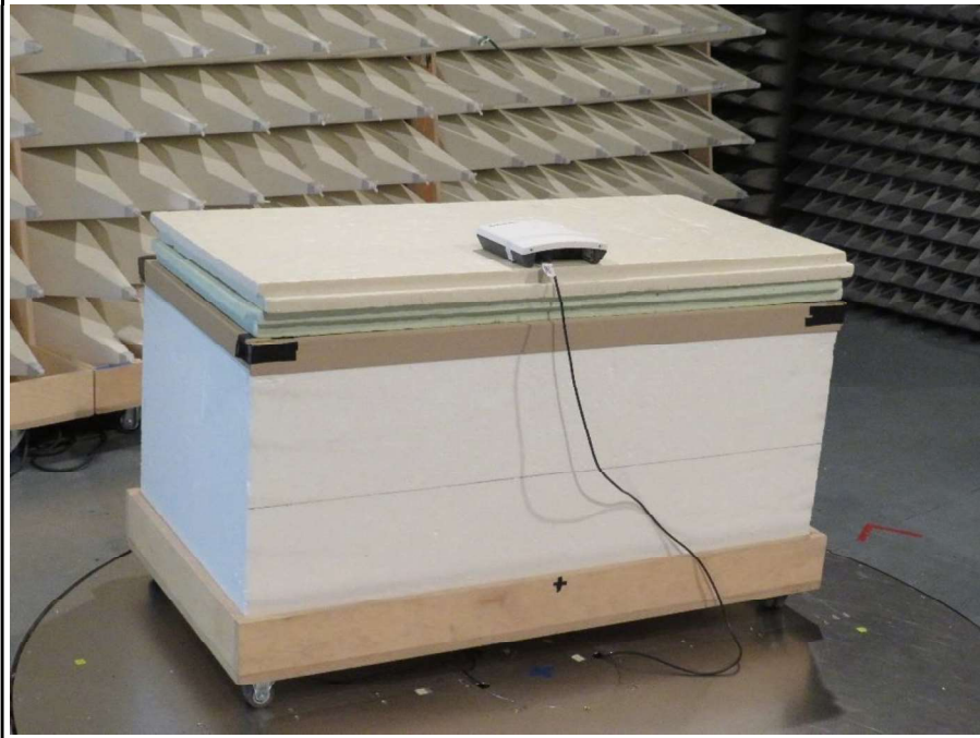
EUT SETUP FOCUS CONFIGURATION 1 AC1
