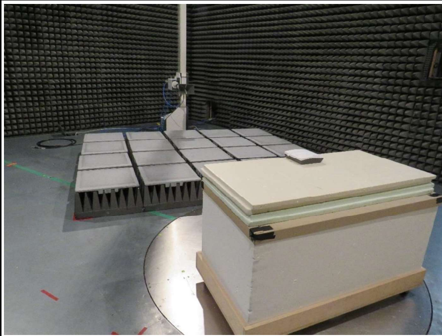
EUT SETUP 1 GHz to 17 GHZ
