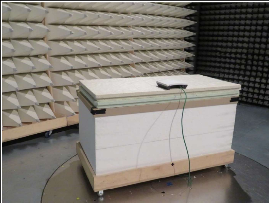
EUT SETUP FOCUS CONFIGURATION 2 AC1
