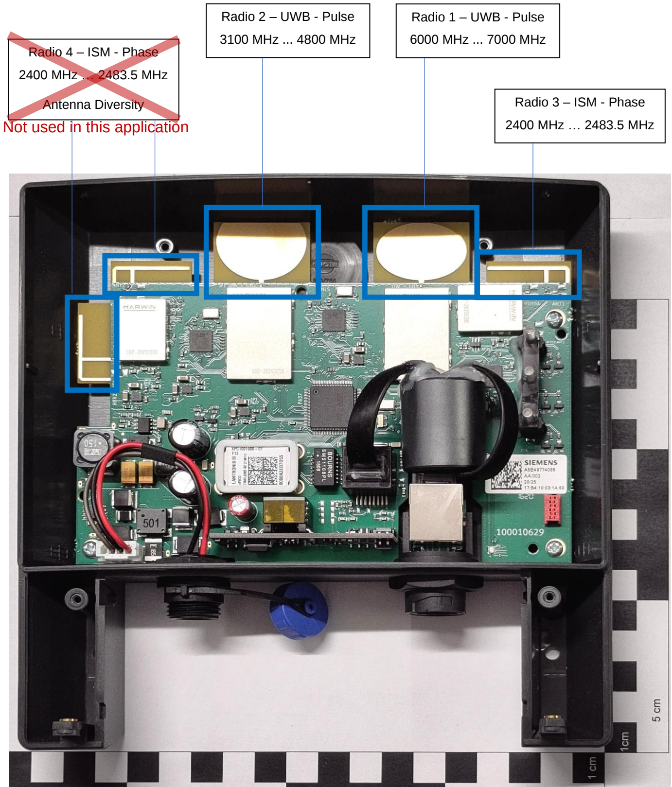
Internal View with Antenna
