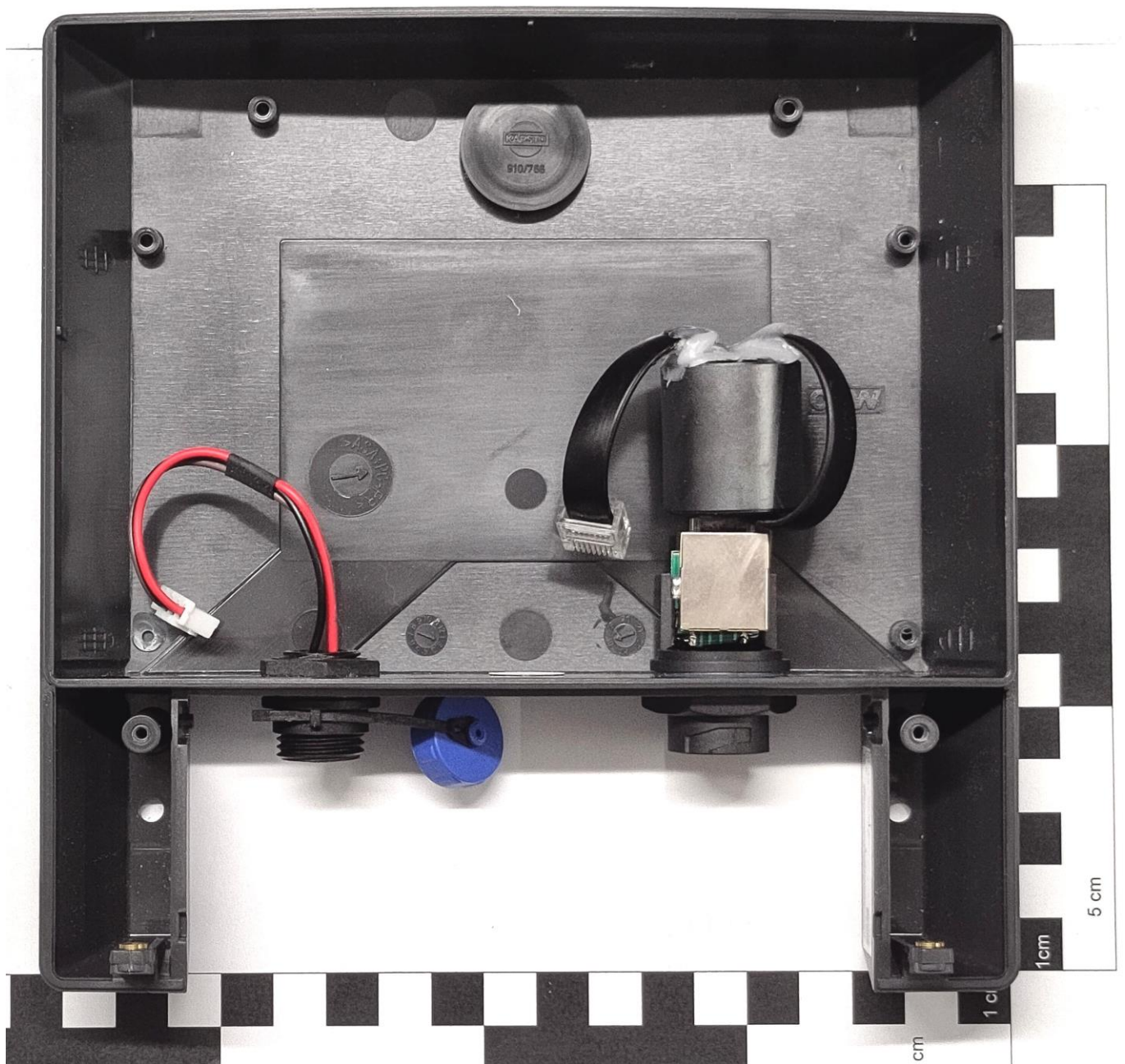
Case with connections
