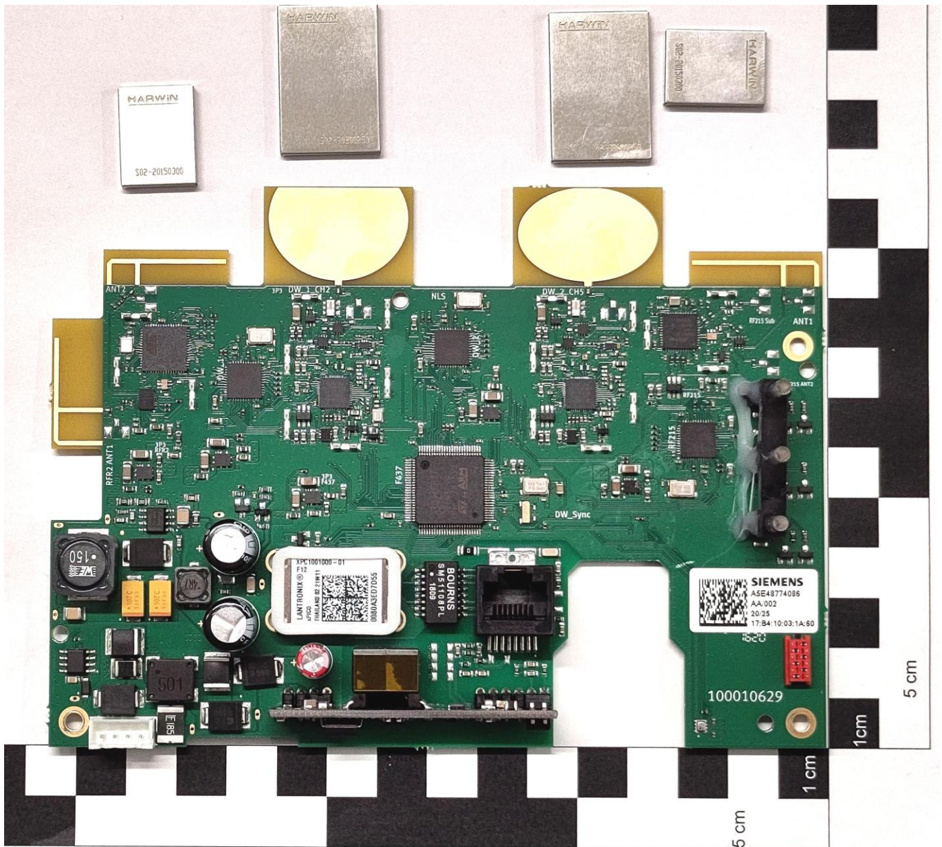
PCB w/o shielding
