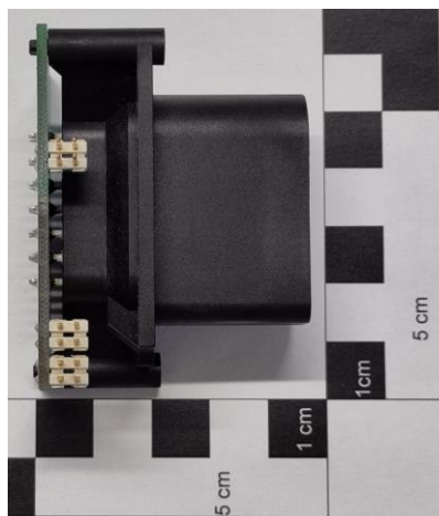
Plug PCB Side
