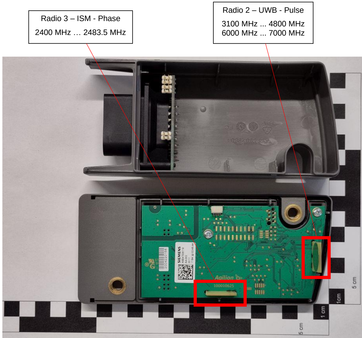
Assembly of PCBs and Housing
