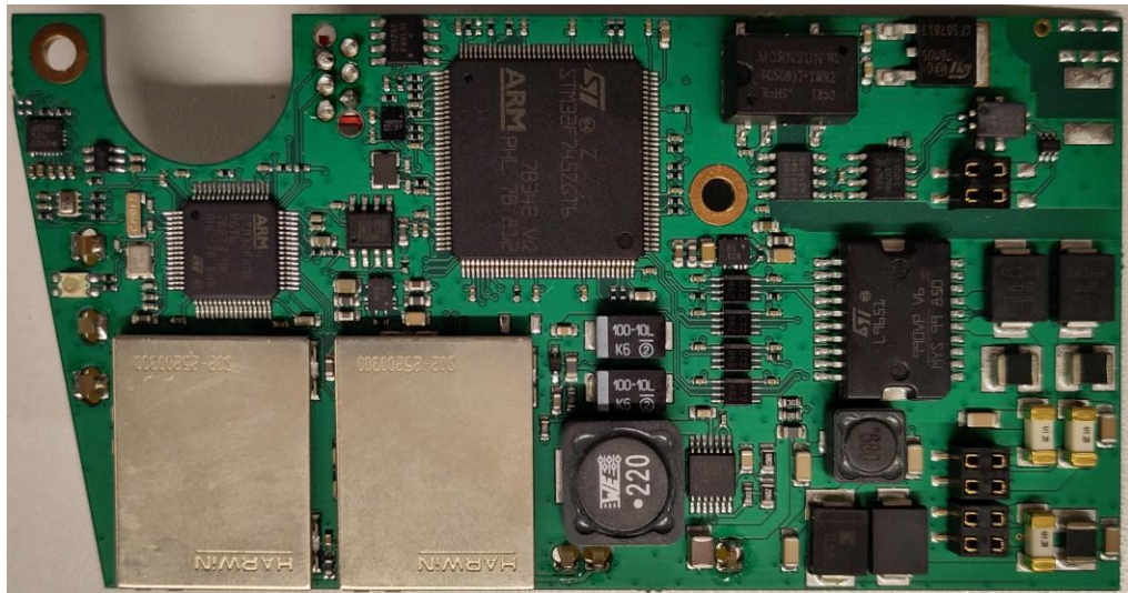
PCB Top View
