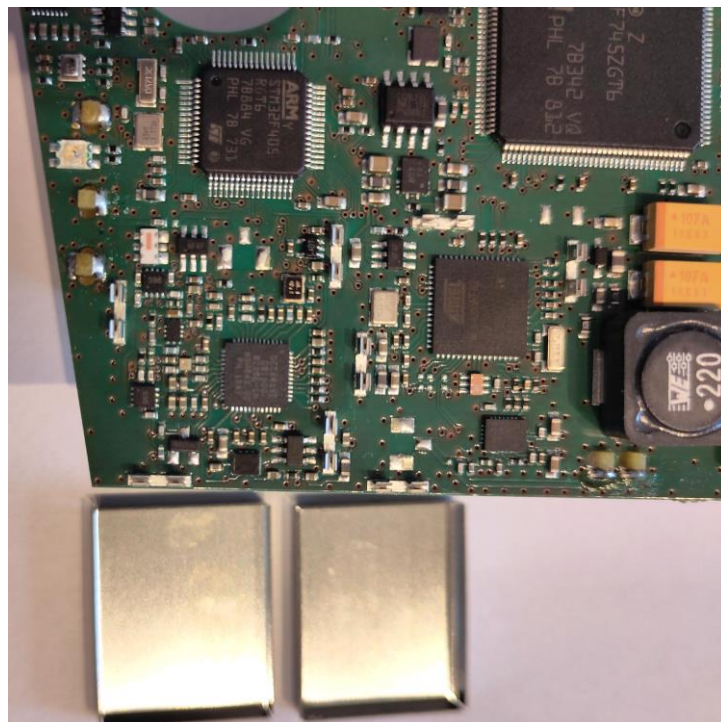
PCB w/o shielding
