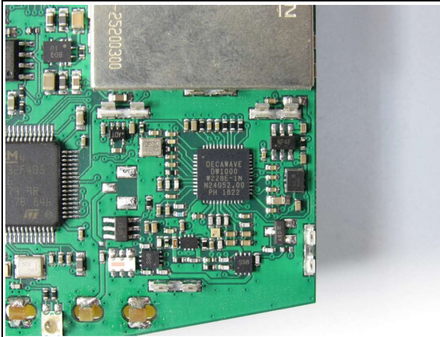
Radio part
