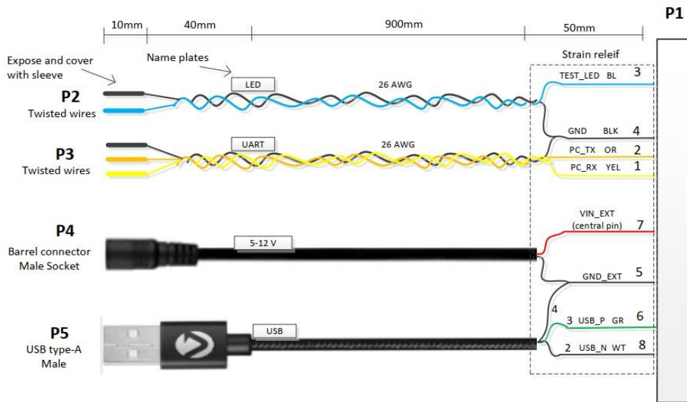
Figure 2-2: UNO-MINI Cable
