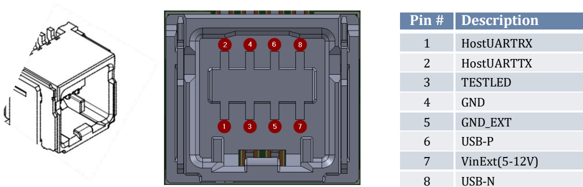
Figure 2-1: UNO-MINI Connector
