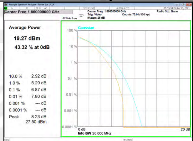
Band 2_100_QPSK_Middle
