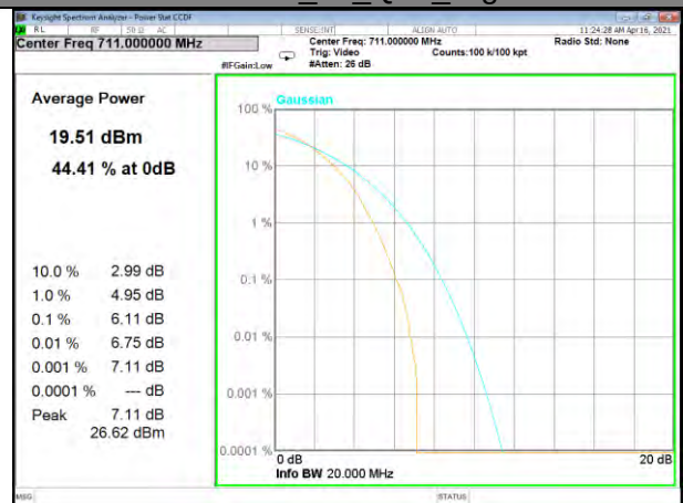
Band 17_50_Q16_High
