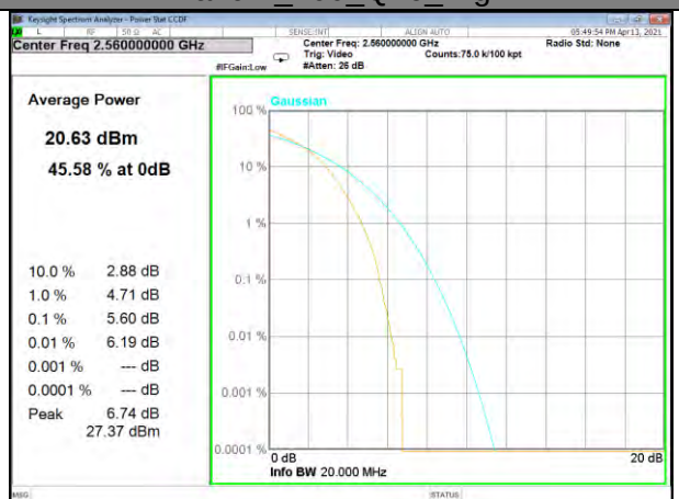
Band 7_100_Q16_High
