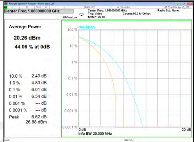
Band 2_100_Q16_Low
