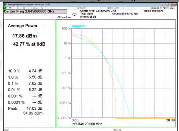
Band 41_100_Q16_High
