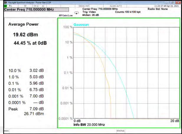
Band 17_50_QPSK_High
