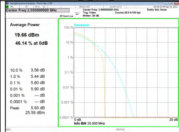
Band 38_1_QPSK_High
