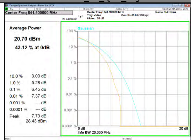
Band 26_75_Q16_High
