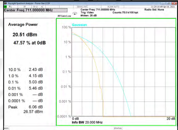
Band 17_50_Q16_High
