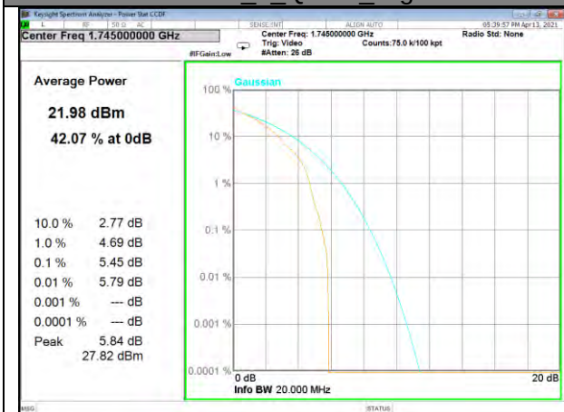
Band 4_1_Q16_High
