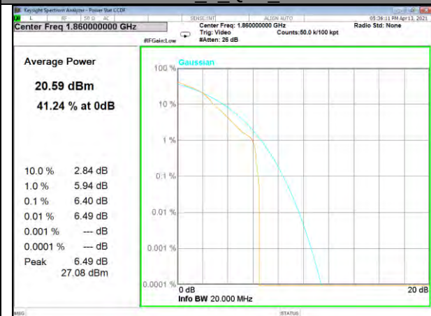
Band 2_1_QPSK_Middle
