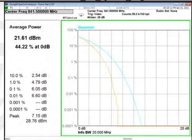
Band 26_75_Q16_High
