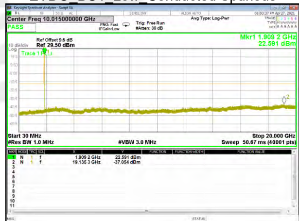
EVDO_BC1_High_Conducted Spurious
