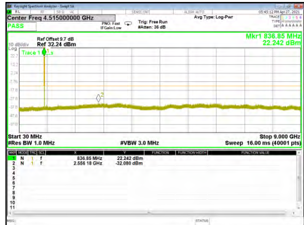
CDMA BC0 Middle Conducted Spurious
