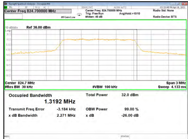
EVDO_CDMA_Lower6BW and 99%
