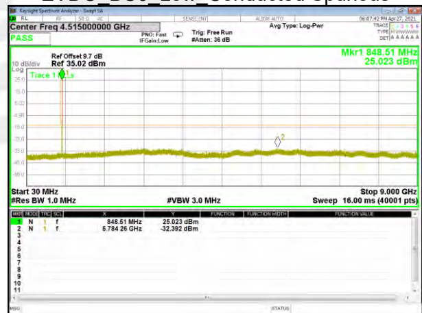
EVDO_BC0_High_Conducted Spurious
