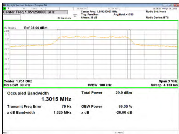
BC1_CDMA_Lower6BW and 99%
