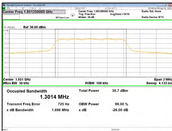
EVDO_CDMA_Lower6BW and 99%
