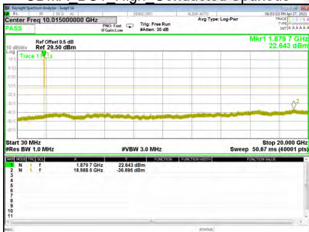
EVDO_BC1_Middle_Conducted Spurious
