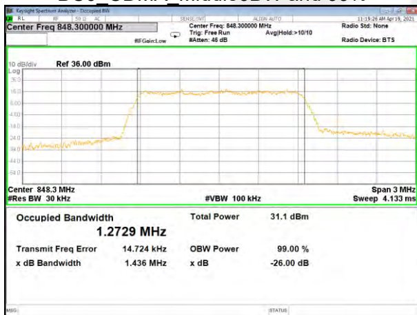
BC0_CDMA_Higher6BW and 99%
