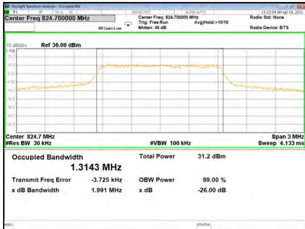
BC0_CDMA_Lower6BW and 99%
