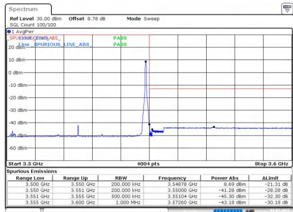
n78(3450-3550) SCS=30kHz DFT_64QAM BW=50MHz HighChannel=635000 RB=1@132
