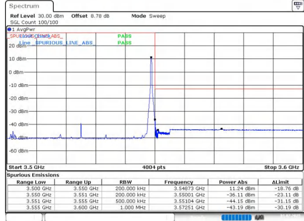
n78(3450-3550) SCS=30kHz DFT_16QAM BW=50MHz HighChannel=635000 RB=1@132
