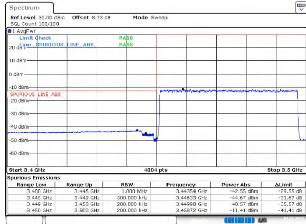
n78(3450-3550) SCS=30kHz DFT_256QAM BW=50MHz LowChannel=631668 RB=128@0
