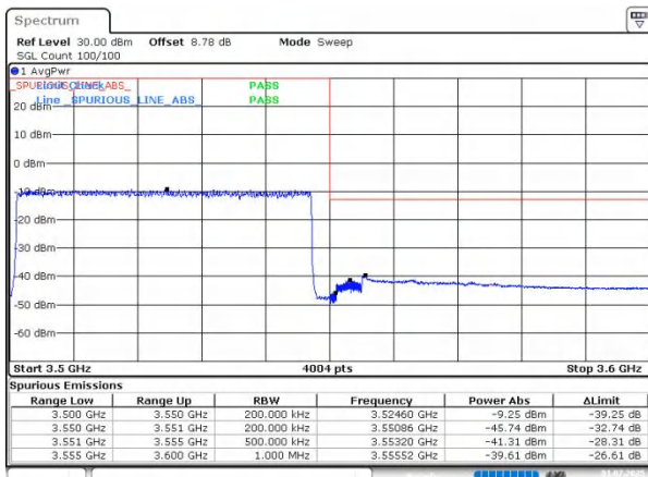
n78(3450-3550) SCS=30kHz DFT_16QAM BW=50MHz HighChannel=635000 RB=128@0
