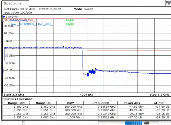
n78(3450-3550) SCS=30kHz DFT_QPSK BW=50MHz HighChannel=635000 RB=128@0
