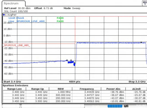
n78(3450-3550) SCS=30kHz DFT_256QAM BW=50MHz LowChannel=631668 RB=1@0
