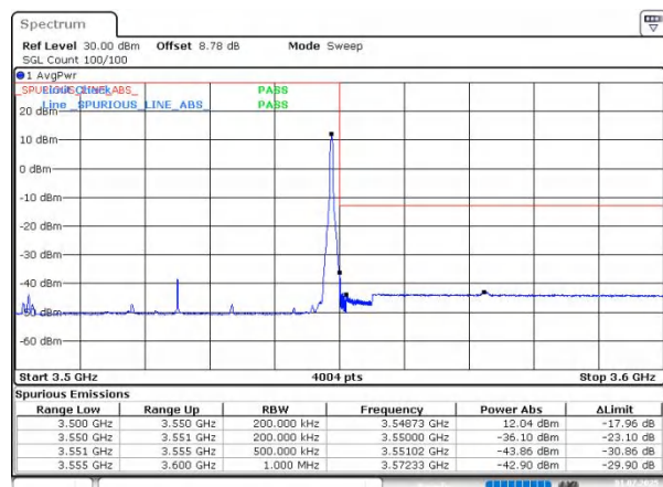
n78(3450-3550) SCS=30kHz DFT_BPSK BW=50MHz HighChannel=635000 RB=1@132
