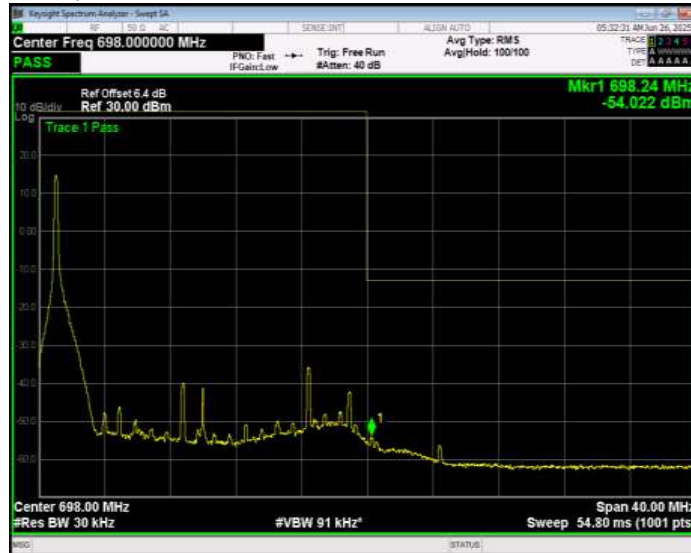
Band71 QPSK BW=20MHz Channel=133372 RB Size=1 Position=#Max Extended
