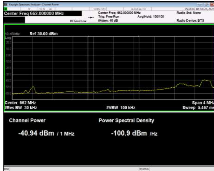
Band71 QPSK BW=5MHz Channel=133147 RB Size=1 Position=#Max Normal
