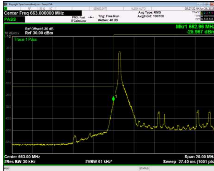
Band71 QPSK BW=10MHz Channel=133172 RB Size=1 Position=#Max Extended
