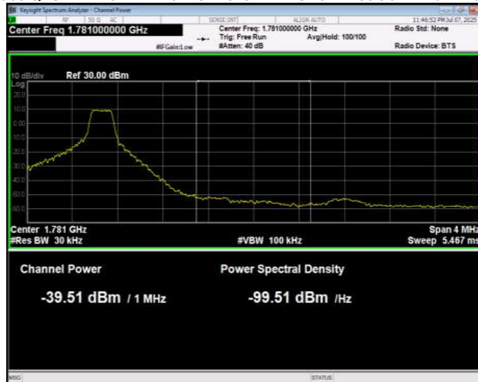
Band66 QPSK BW=5MHz Channel=132647 RB Size=1 Position=#Max Normal
