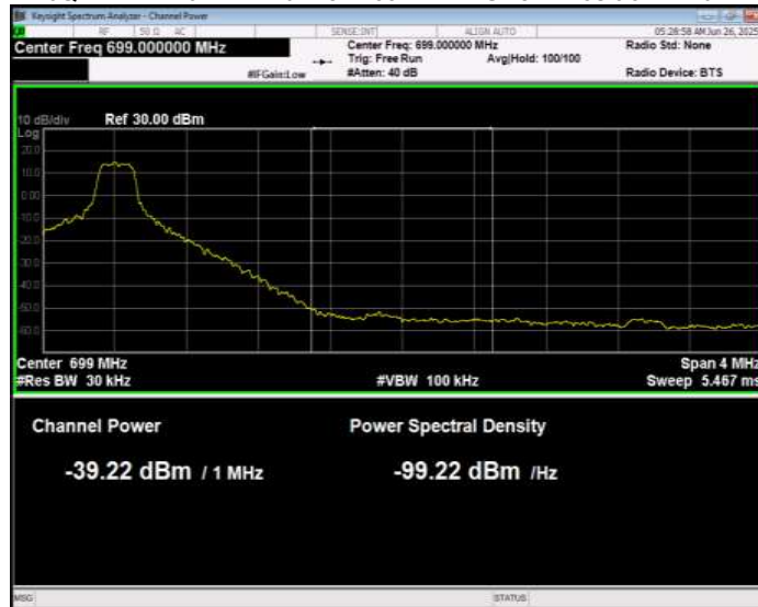
Band71 16QAM BW=10MHz Channel=133422 RB Size=1 Position=#Max Normal
