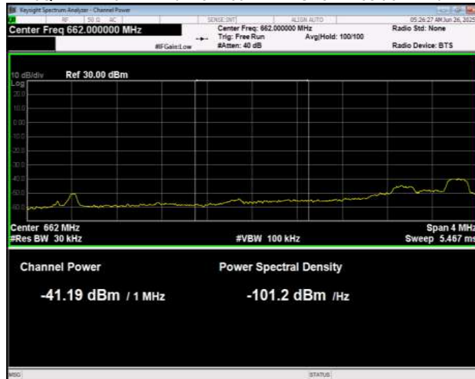
Band71 16QAM BW=5MHz Channel=133147 RB Size=1 Position=#Max Normal
