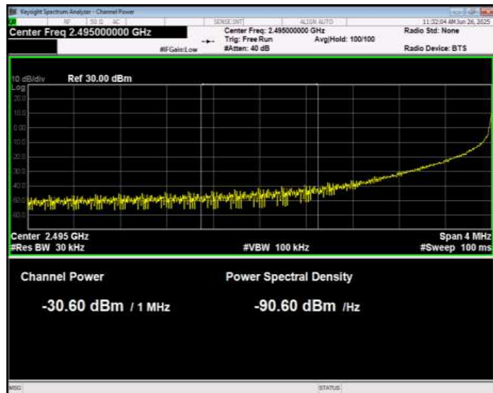
Band41 QPSK BW=20MHz Channel=39750 RB Size=1 Position=#0 Normal
