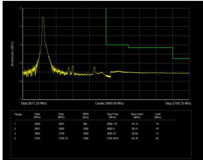
Band41 QPSK BW=15MHz Channel=41515 RB Size=1 Position=#Max Extended
