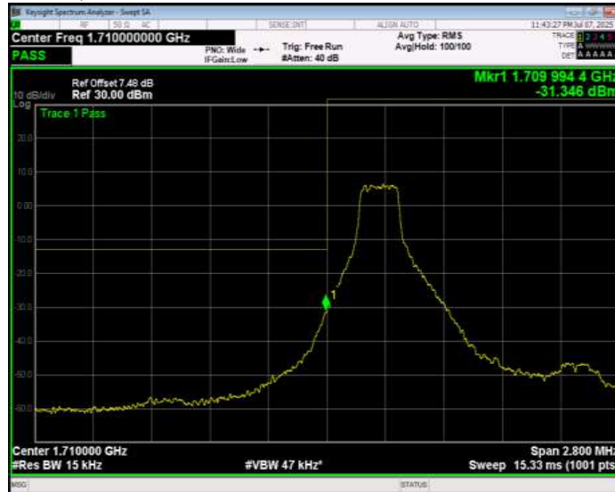
Band66 16QAM BW=1.4MHz Channel=131979 RB Size=1 Position=#Max Extended
