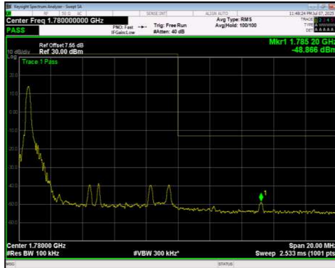
Band66 16QAM BW=10MHz Channel=132622 RB Size=1 Position=#Max Extended
