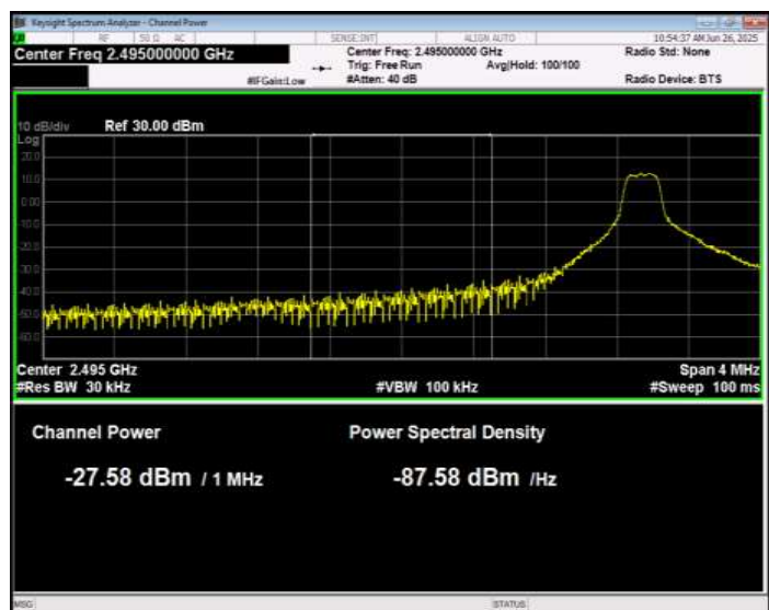
Band41 QPSK BW=5MHz Channel=39675 RB Size=1 Position=#0 Normal
