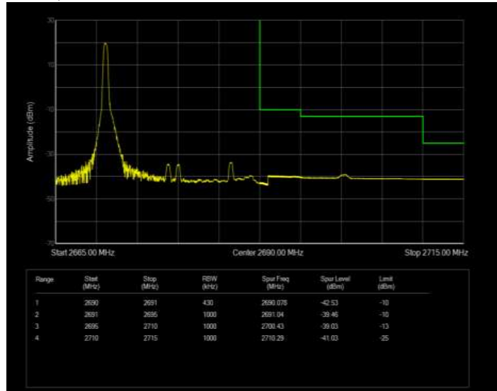
Band41 QPSK BW=20MHz Channel=41490 RB Size=1 Position=#Max Extended
