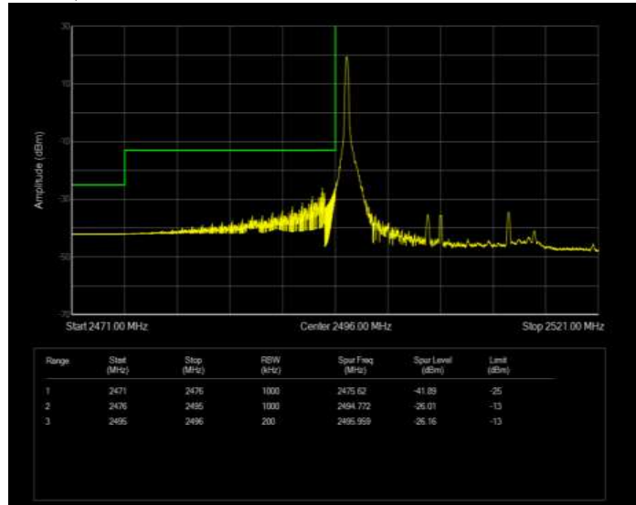
Band41 QPSK BW=20MHz Channel=39750 RB Size=1 Position=#Max Extended
