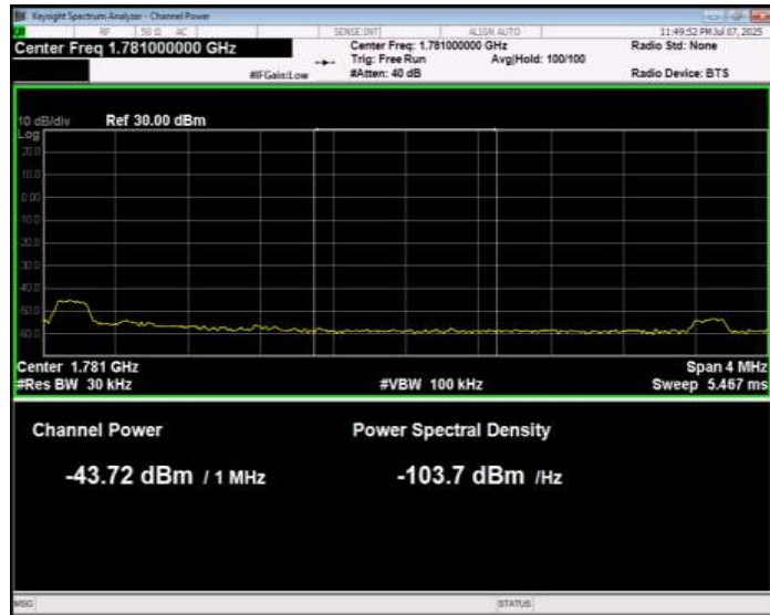
Band66 QPSK BW=15MHz Channel=132597 RB Size=1 Position=#0 Normal
