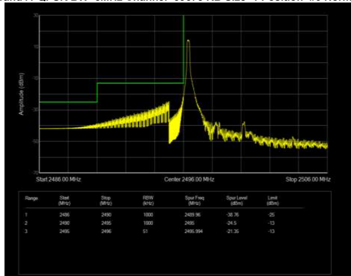
Band41 QPSK BW=5MHz Channel=39675 RB Size=1 Position=#Max Extended
