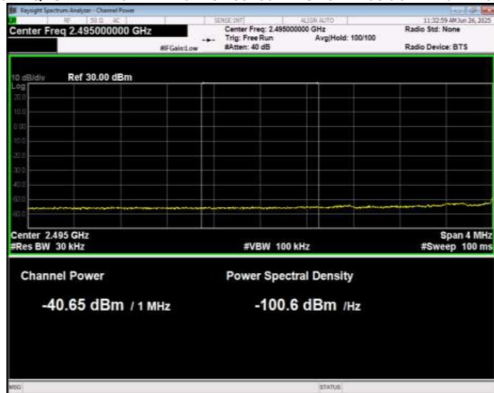
Band41 QPSK BW=20MHz Channel=39750 RB Size=1 Position=#Max Normal
