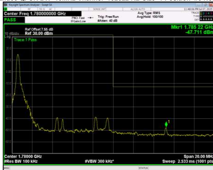
Band66 QPSK BW=10MHz Channel=132622 RB Size=1 Position=#Max Extended
