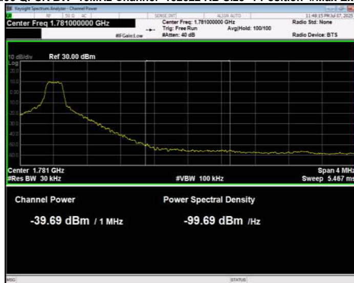
Band66 QPSK BW=10MHz Channel=132622 RB Size=1 Position=#Max Normal
