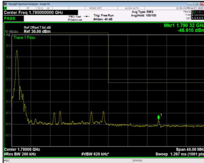
Band66 QPSK BW=20MHz Channel=132572 RB Size=1 Position=#Max Extended
