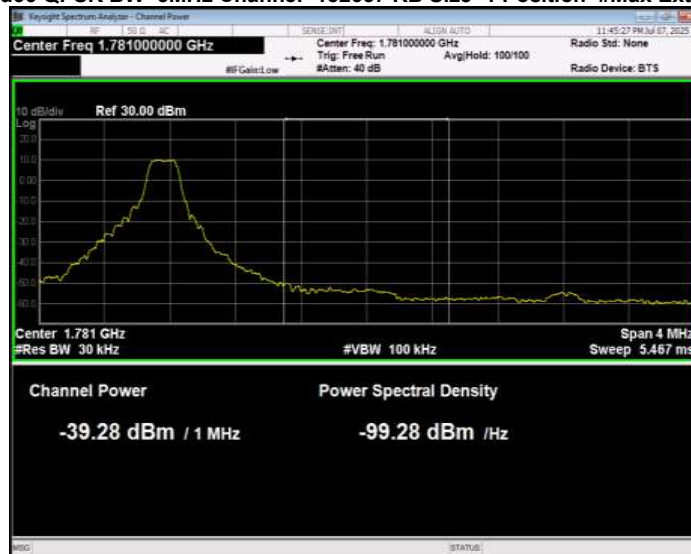
Band66 QPSK BW=3MHz Channel=132657 RB Size=1 Position=#Max Normal
