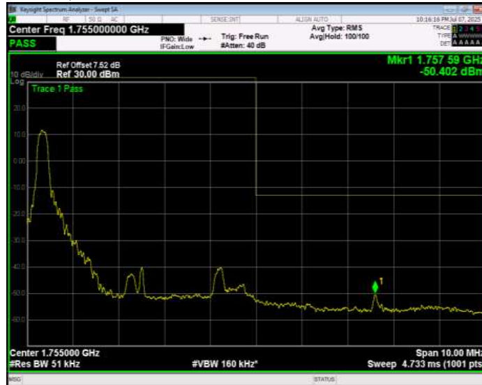
Band4 16QAM BW=5MHz Channel=20375 RB Size=1 Position=#Max Extended
