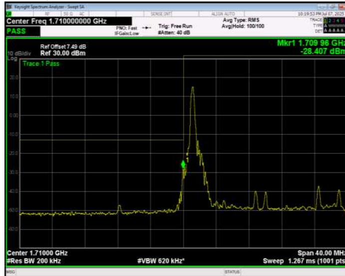
Band4 16QAM BW=20MHz Channel=20050 RB Size=1 Position=#Max Extended
