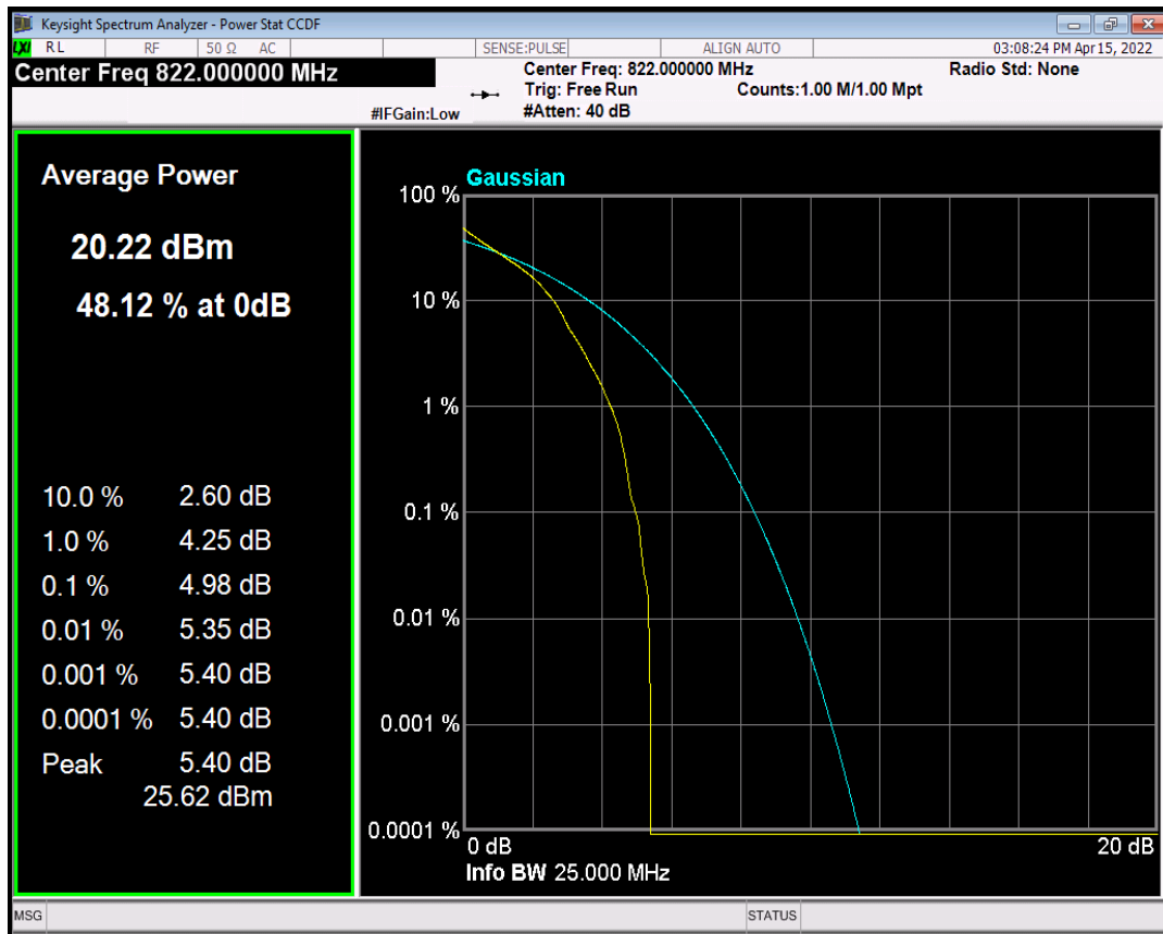
Band26(820-824) QPSK BW=3MHz Channel=26770 RB Size=1 Position=#0
