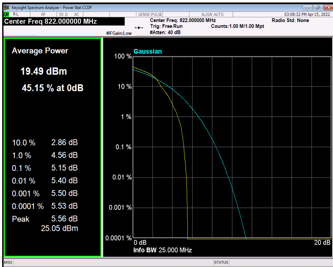
Band26(820-824) QPSK BW=1.4MHz Channel=26770 RB Size=1 Position=#0
