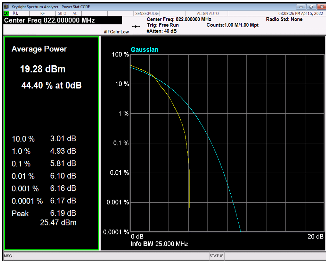
Band26(820-824) QAM16 BW=3MHz Channel=26770 RB Size=1 Position=#0
