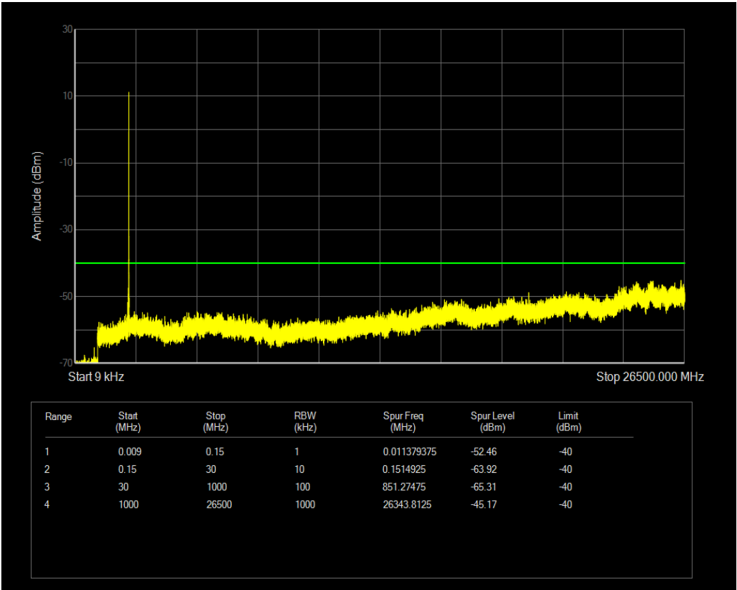
Band40(2350-2360) QAM16 BW=5MHz Channel=39225 RB Size=25 Position=#0
