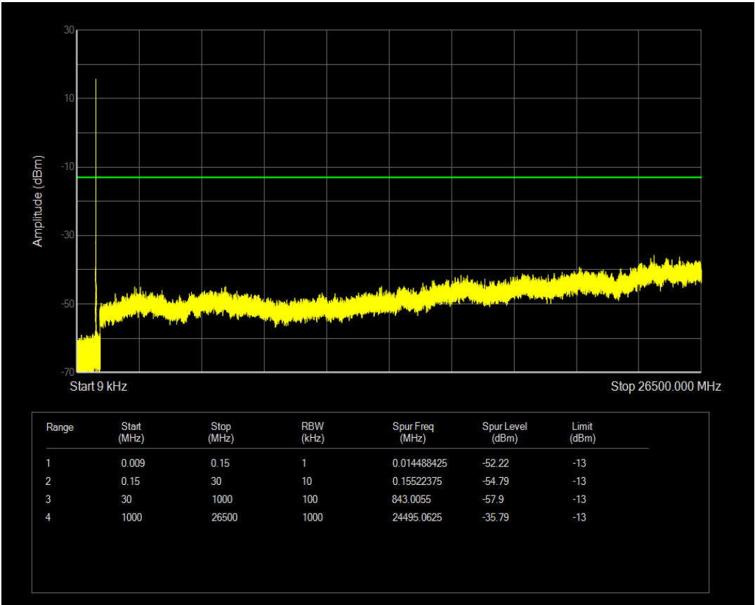
Band26(820-824) QAM16 BW=3MHz Channel=26765 RB Size=15 Position=#0
