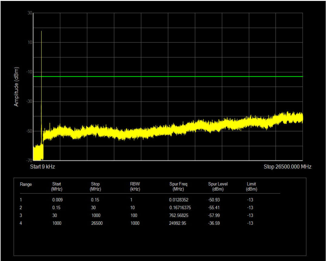
Band26(820-824) QPSK BW=3MHz Channel=26765 RB Size=15 Position=#0
