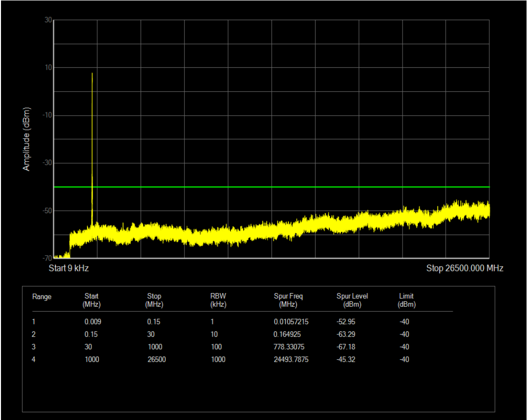
Band40(2350-2360) QAM16 BW=5MHz Channel=39175 RB Size=25 Position=#0
