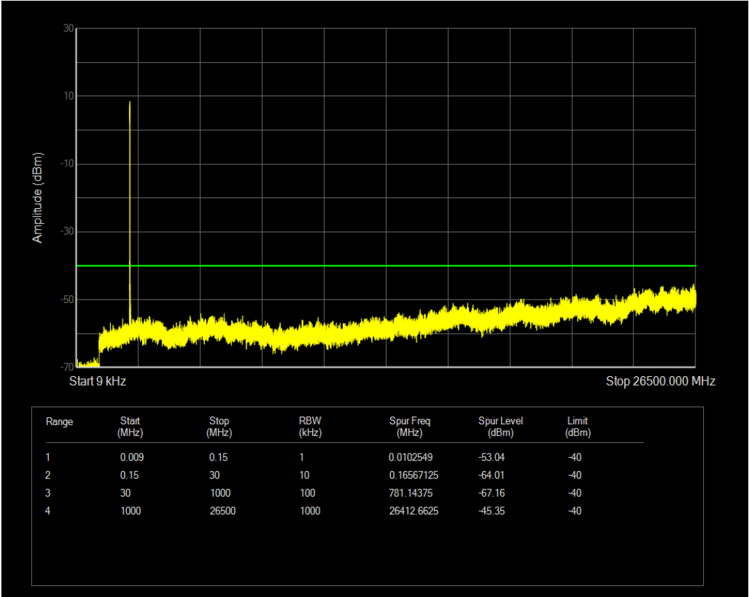
Band40(2305-2315) QAM16 BW=5MHz Channel=38725 RB Size=25 Position=#0
