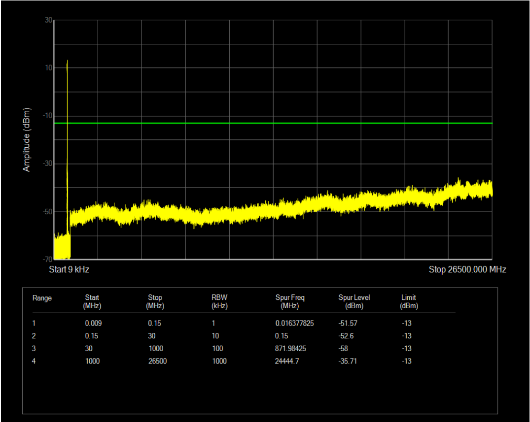
Band26(820-824) QPSK BW=3MHz Channel=26775 RB Size=15 Position=#0
