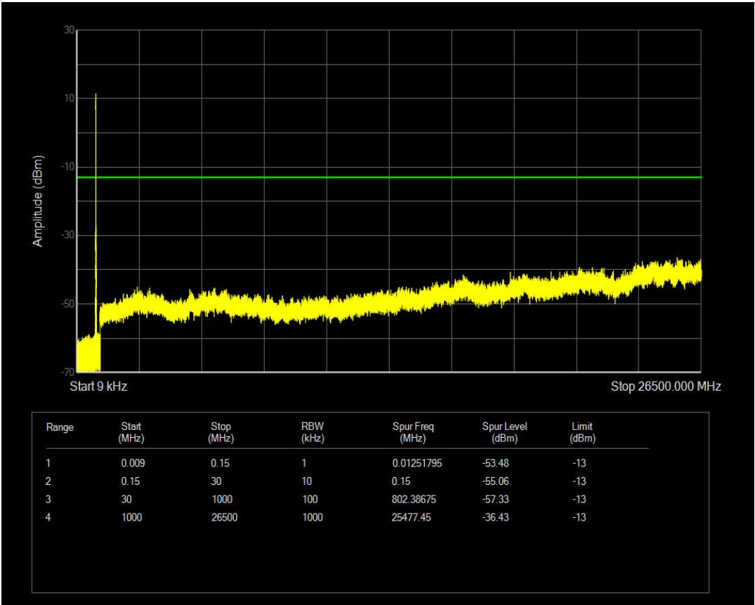
Band26(820-824) QPSK BW=1.4MHz Channel=26757 RB Size=6 Position=#0
