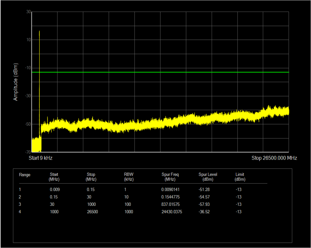
Band26(820-824) QPSK BW=1.4MHz Channel=26783 RB Size=6 Position=#0
