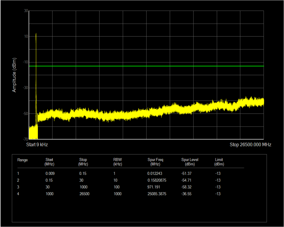
Band26(820-824) QAM16 BW=3MHz Channel=26775 RB Size=15 Position=#0
