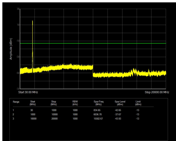
n66 SCS=15kHz DFT_BPSK BW=40MHz Channel=346000 RB=216@0 NVNT
