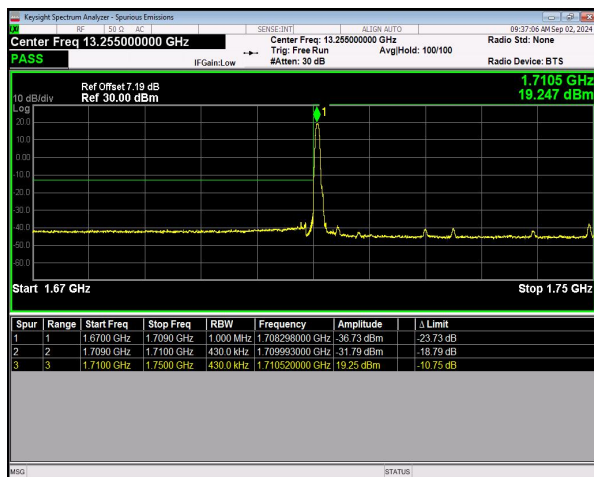
n66 SCS=15kHz DFT_256QAM BW=40MHz LowChannel=346000 RB=1@0 NVNT
