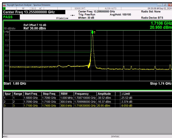
n66 SCS=15kHz DFT_64QAM BW=30MHz LowChannel=345000 RB=1@0 NVNT
