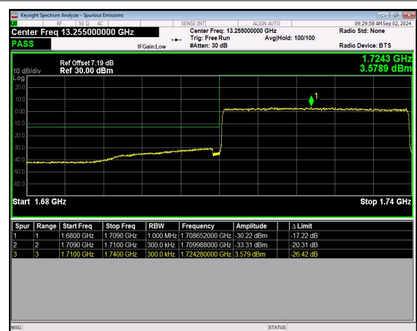
n66 SCS=15kHz DFT_QPSK BW=30MHz LowChannel=345000 RB=160@0 NVNT
