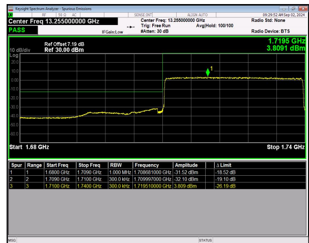
n66 SCS=15kHz DFT_BPSK BW=30MHz LowChannel=345000 RB=160@0 NVNT
