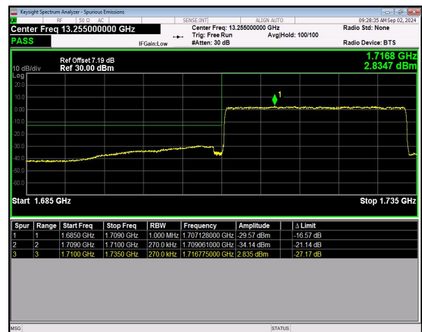
n66 SCS=15kHz DFT_16QAM BW=25MHz LowChannel=344500 RB=128@0 NVNT
