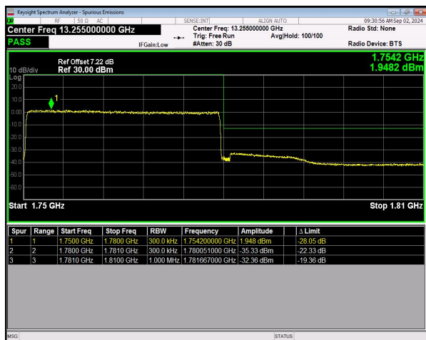
n66 SCS=15kHz DFT_64QAM BW=30MHz HighChannel=353000 RB=160@0 NVNT
