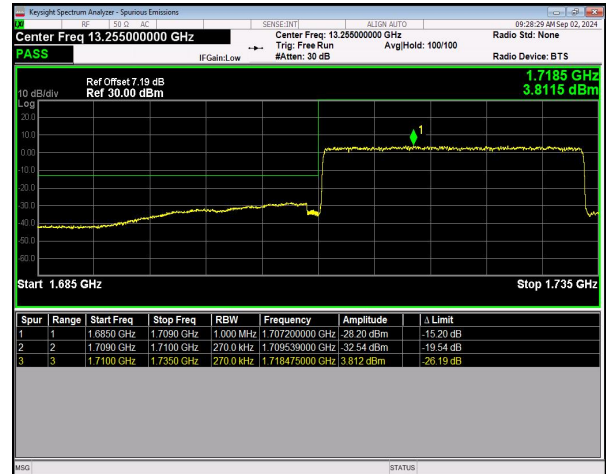
n66 SCS=15kHz DFT_QPSK BW=25MHz LowChannel=344500 RB=128@0 NVNT
