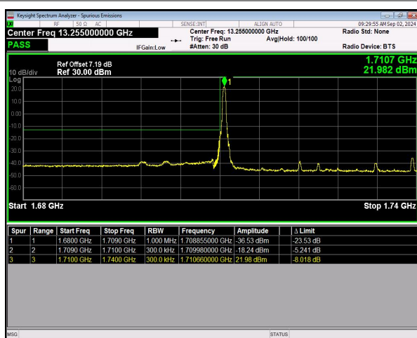
n66 SCS=15kHz DFT_QPSK BW=30MHz LowChannel=345000 RB=1@0 NVNT
