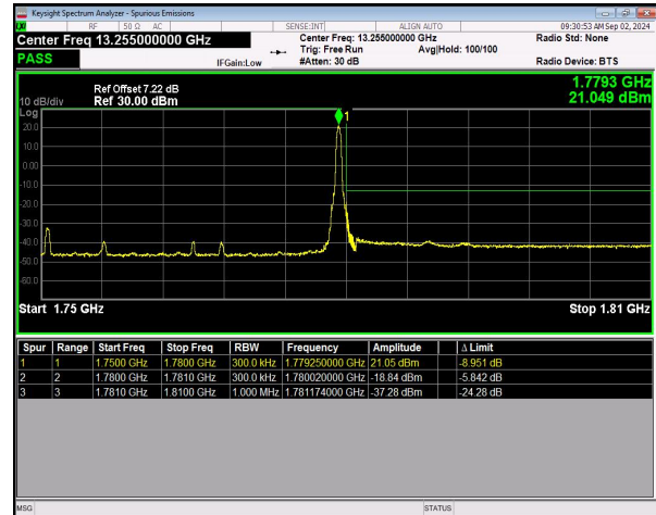
n66 SCS=15kHz DFT_64QAM BW=30MHz HighChannel=353000 RB=1@159 NVNT
