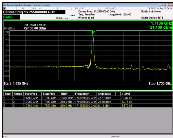
n66 SCS=15kHz DFT_16QAM BW=25MHz LowChannel=344500 RB=1@0 NVNT
