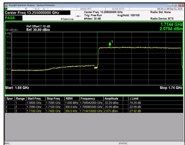
n66 SCS=15kHz DFT_64QAM BW=30MHz LowChannel=345000 RB=160@0 NVNT
