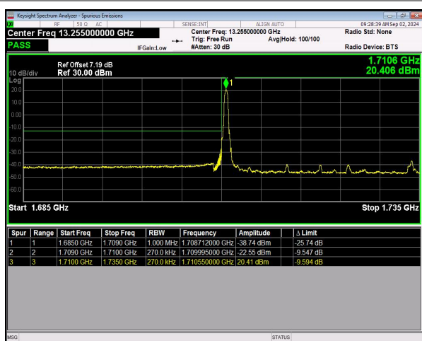
n66 SCS=15kHz DFT_64QAM BW=25MHz LowChannel=344500 RB=1@0 NVNT
