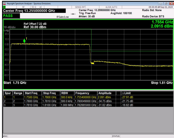
n66 SCS=15kHz DFT_16QAM BW=30MHz HighChannel=353000 RB=160@0 NVNT
