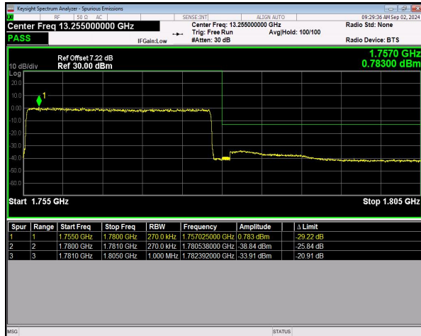
n66 SCS=15kHz DFT_256QAM BW=25MHz HighChannel=353500 RB=128@0 NVNT
