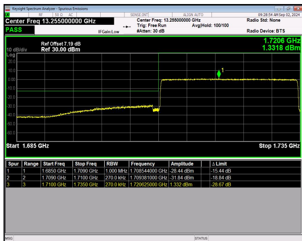
n66 SCS=15kHz CP_QPSK BW=25MHz LowChannel=344500 RB=133@0 NVNT
