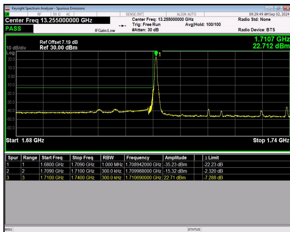
n66 SCS=15kHz DFT_BPSK BW=30MHz LowChannel=345000 RB=1@0 NVNT
