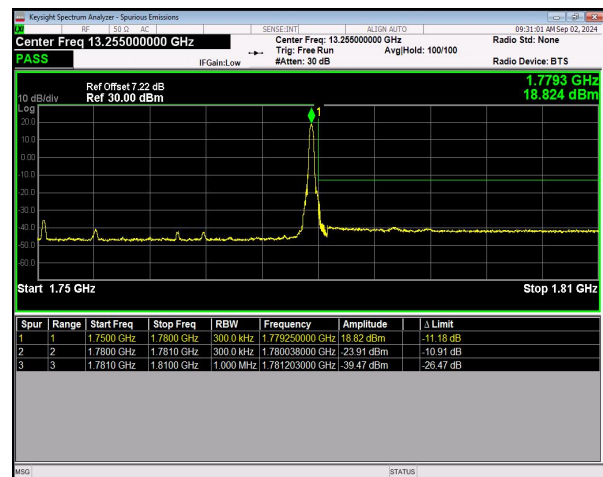
n66 SCS=15kHz DFT_256QAM BW=30MHz HighChannel=353000 RB=1@159 NVNT
