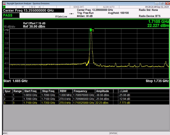
n66 SCS=15kHz DFT_QPSK BW=25MHz LowChannel=344500 RB=1@0 NVNT
