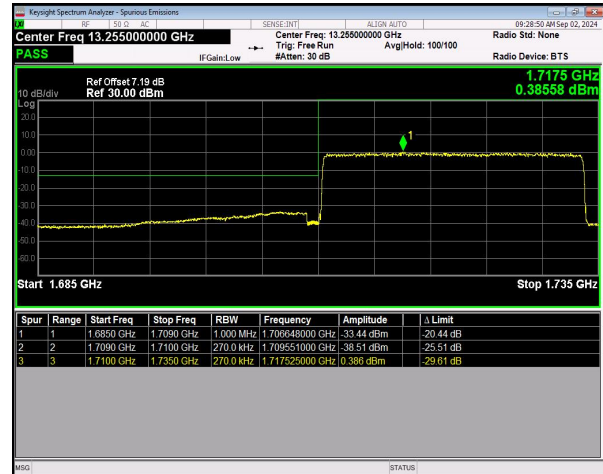
n66 SCS=15kHz DFT_256QAM BW=25MHz LowChannel=344500 RB=128@0 NVNT
