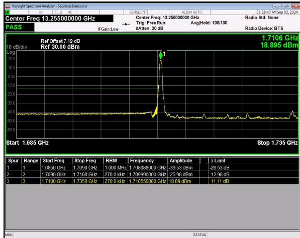
n66 SCS=15kHz DFT_256QAM BW=25MHz LowChannel=344500 RB=1@0 NVNT
