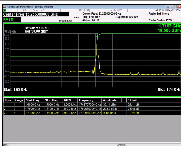
n66 SCS=15kHz DFT_256QAM BW=30MHz LowChannel=345000 RB=1@0 NVNT
