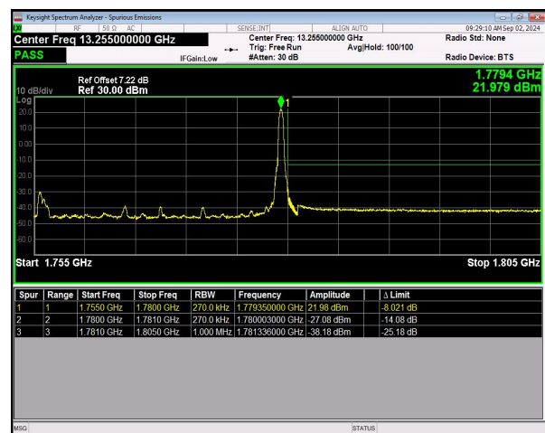
n66 SCS=15kHz DFT_QPSK BW=25MHz HighChannel=353500 RB=1@132 NVNT
