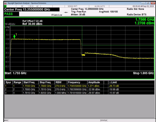
n66 SCS=15kHz CP_QPSK BW=25MHz HighChannel=353500 RB=133@0 NVNT
