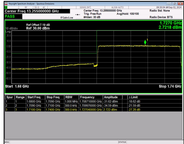
n66 SCS=15kHz DFT_16QAM BW=30MHz LowChannel=345000 RB=160@0 NVNT
