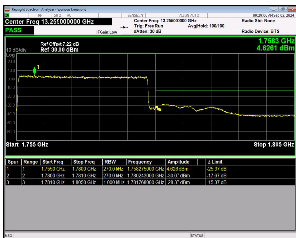
n66 SCS=15kHz DFT_BPSK BW=25MHz HighChannel=353500 RB=128@0 NVNT
