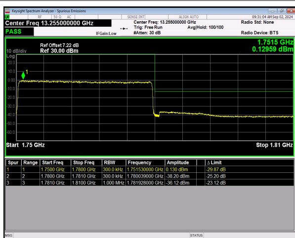
n66 SCS=15kHz DFT_256QAM BW=30MHz HighChannel=353000 RB=160@0 NVNT
