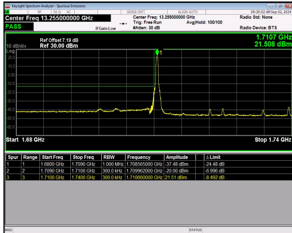
n66 SCS=15kHz DFT_16QAM BW=30MHz LowChannel=345000 RB=1@0 NVNT
