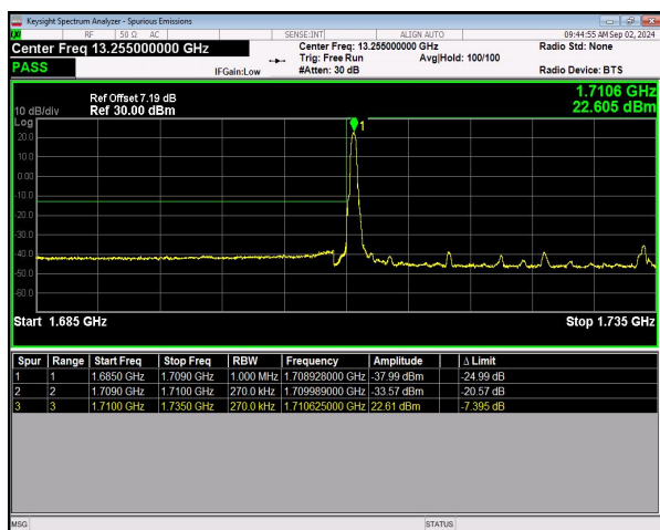
n66 SCS=15kHz DFT_BPSK BW=25MHz LowChannel=344500 RB=1@0 NVNT
