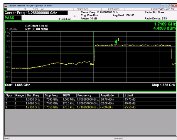
n66 SCS=15kHz DFT_BPSK BW=25MHz LowChannel=344500 RB=128@0 NVNT
