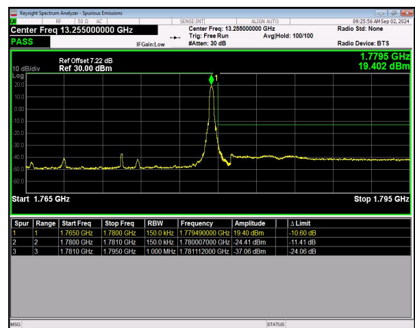
n66 SCS=15kHz DFT_16QAM BW=15MHz HighChannel=354500 RB=1@78 NVNT
