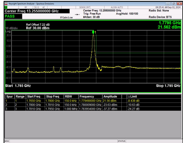
n66 SCS=15kHz DFT_BPSK BW=15MHz HighChannel=354500 RB=1@78 NVNT
