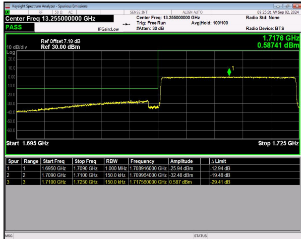
n66 SCS=15kHz CP_QPSK BW=15MHz LowChannel=343500 RB=79@0 NVNT
