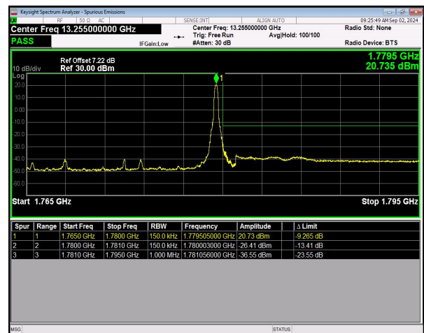
n66 SCS=15kHz DFT_QPSK BW=15MHz HighChannel=354500 RB=1@78 NVNT
