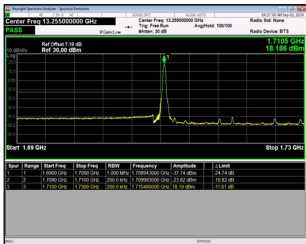
n66 SCS=15kHz DFT_256QAM BW=20MHz LowChannel=344000 RB=1@0 NVNT
