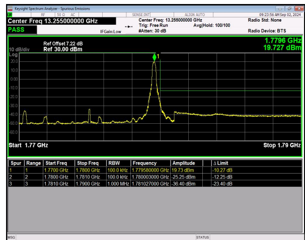
n66 SCS=15kHz DFT_BPSK BW=10MHz HighChannel=355000 RB=1@51 NVNT
