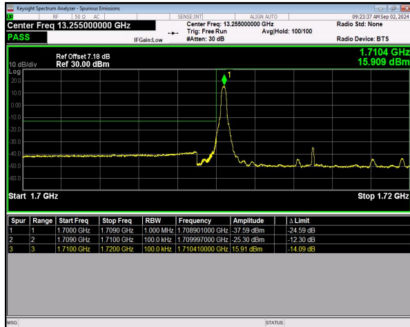
n66 SCS=15kHz DFT_256QAM BW=10MHz LowChannel=343000 RB=1@0 NVNT
