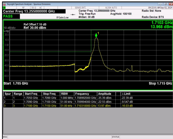
RB=1@0 NVNT
