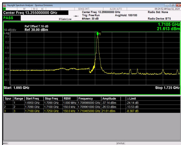
n66 SCS=15kHz DFT_BPSK BW=15MHz LowChannel=343500 RB=1@0 NVNT
