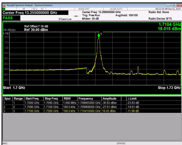
n66 SCS=15kHz DFT_16QAM BW=10MHz LowChannel=343000 RB=1@0 NVNT
