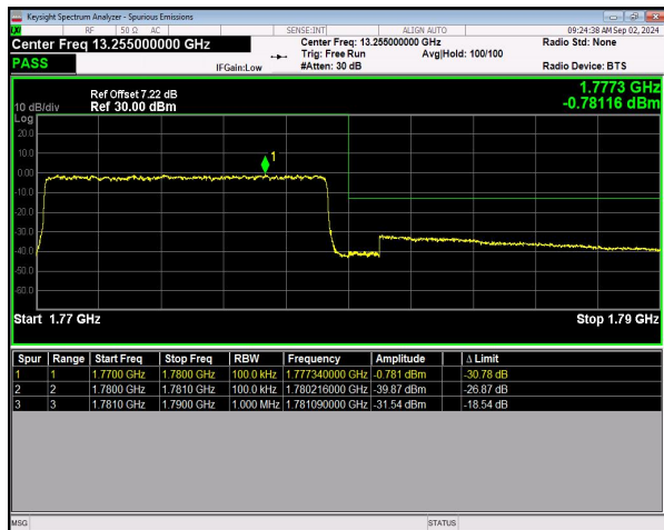
n66 SCS=15kHz DFT_256QAM BW=10MHz HighChannel=355000 RB=50@0 NVNT
