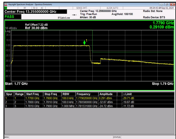
n66 SCS=15kHz CP_QPSK BW=10MHz HighChannel=355000 RB=52@0 NVNT
