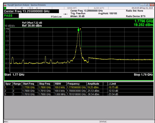
n66 SCS=15kHz DFT_QPSK BW=10MHz HighChannel=355000 RB=1@51 NVNT
