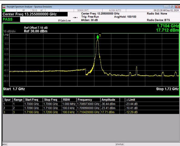
n66 SCS=15kHz DFT_64QAM BW=10MHz LowChannel=343000 RB=1@0 NVNT
