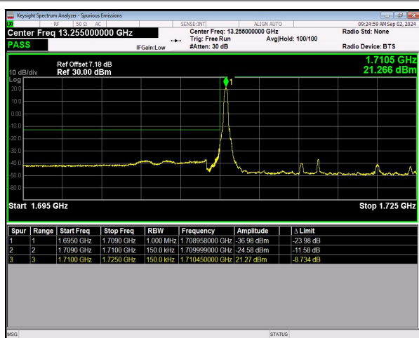
n66 SCS=15kHz DFT_QPSK BW=15MHz LowChannel=343500 RB=1@0 NVNT
