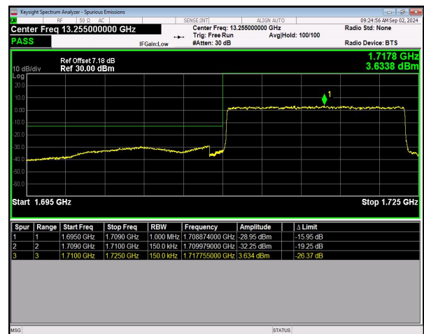
n66 SCS=15kHz DFT_BPSK BW=15MHz LowChannel=343500 RB=75@0 NVNT
