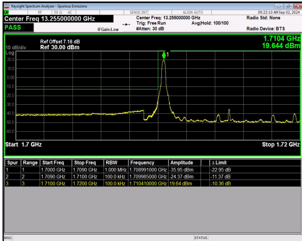
n66 SCS=15kHz DFT_QPSK BW=10MHz LowChannel=343000 RB=1@0 NVNT
