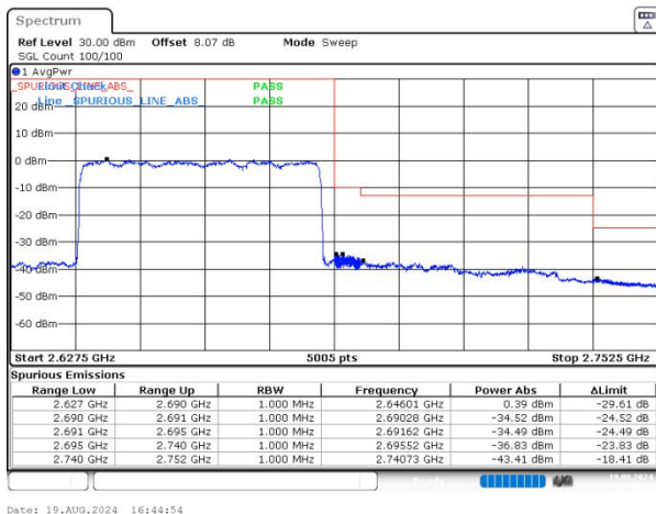
n41 SCS=30kHz DFT_QPSK BW=50MHz HighChannel=532998 RB=128@0 NVNT
