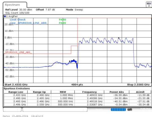
n41 SCS=30kHz DFT_QPSK BW=50MHz LowChannel=504204 RB=128@0 NVNT
