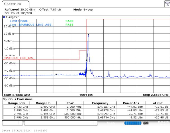
n41 SCS=30kHz DFT_BPSK BW=50MHz LowChannel=504204 RB=1@0 NVNT
