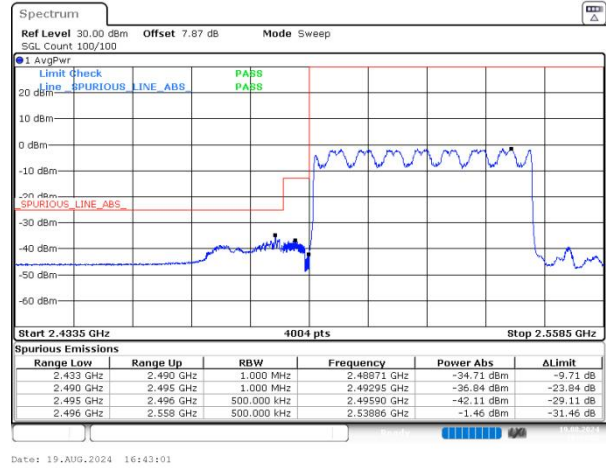
n41 SCS=30kHz DFT_BPSK BW=50MHz LowChannel=504204 RB=128@0 NVNT
