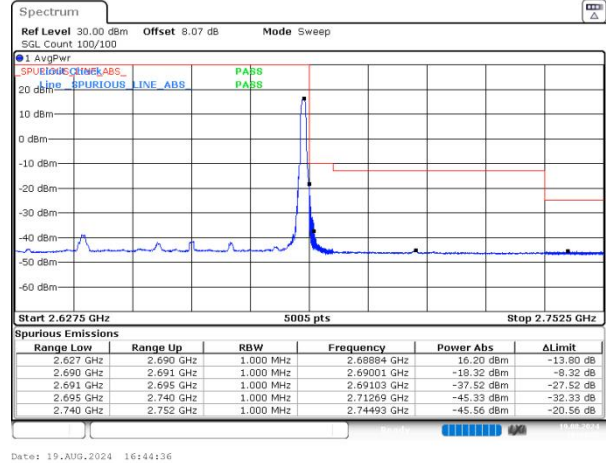
n41 SCS=30kHz DFT_BPSK BW=50MHz HighChannel=532998 RB=1@132 NVNT
