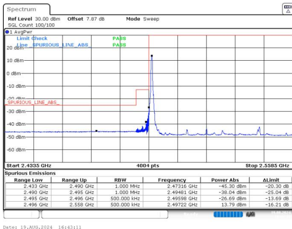
n41 SCS=30kHz DFT_QPSK BW=50MHz LowChannel=504204 RB=1@0 NVNT
