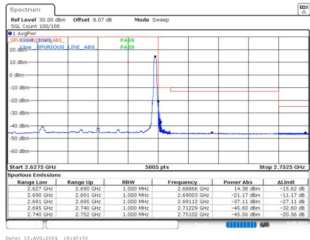
n41 SCS=30kHz DFT_16QAM BW=50MHz HighChannel=532998 RB=1@132 NVNT
