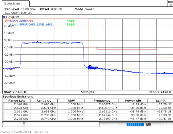
n41 SCS=30kHz DFT_256QAM BW=40MHz HighChannel=534000 RB=100@0 NVNT
