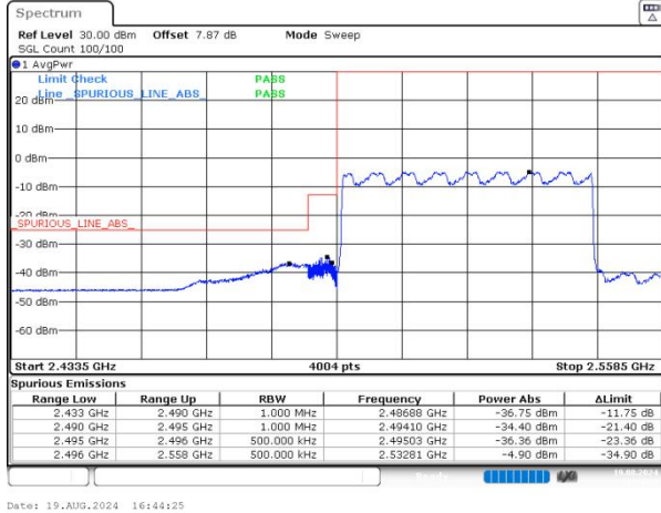
n41 SCS=30kHz CP_QPSK BW=50MHz LowChannel=504204 RB=133@0 NVNT
