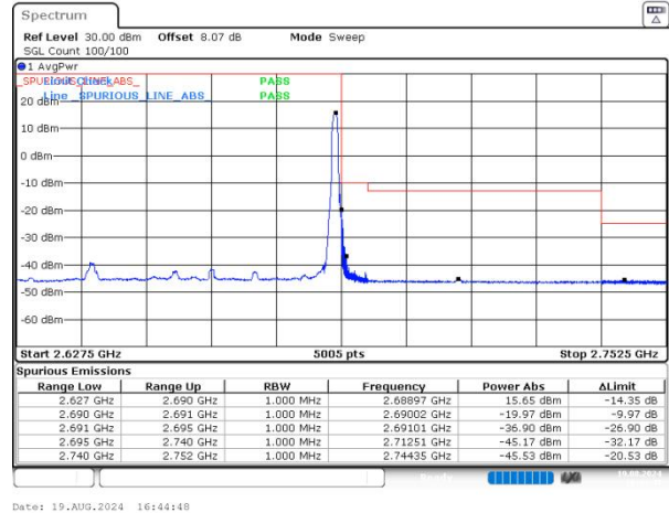
n41 SCS=30kHz DFT_QPSK BW=50MHz HighChannel=532998 RB=1@132 NVNT
