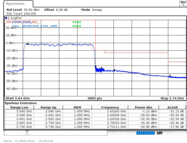
n41 SCS=30kHz CP_QPSK BW=40MHz HighChannel=534000 RB=106@0 NVNT
