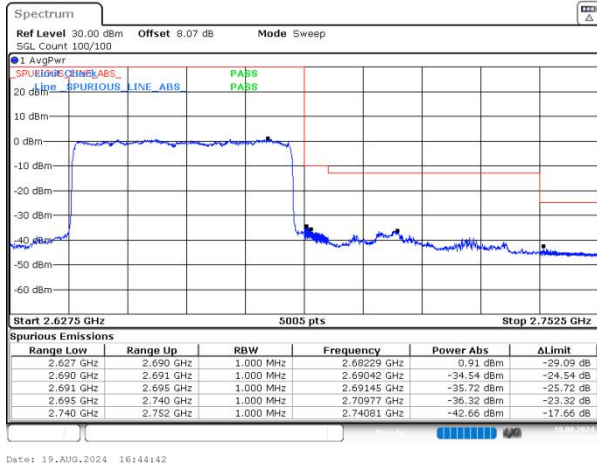
n41 SCS=30kHz DFT_BPSK BW=50MHz HighChannel=532998 RB=128@0 NVNT
