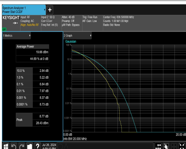
n5 SCS=15kHz DFT_256QAM BW=5MHz Channel=167300
