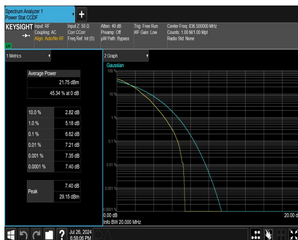
n5 SCS=15kHz DFT_64QAM BW=5MHz Channel=167300
