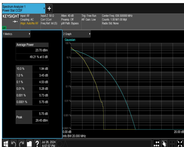
n5 SCS=15kHz DFT_BPSK BW=5MHz Channel=167300
