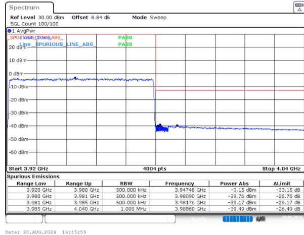
n77(3700-3980) SCS=30kHz DFT_BPSK BW=60MHz HighChannel=663332 RB=1@161 NVNT
