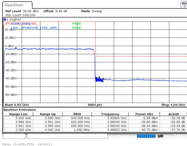
n77(3700-3980) SCS=30kHz DFT_BPSK BW=60MHz HighChannel=663332 RB=162@0 NVNT
