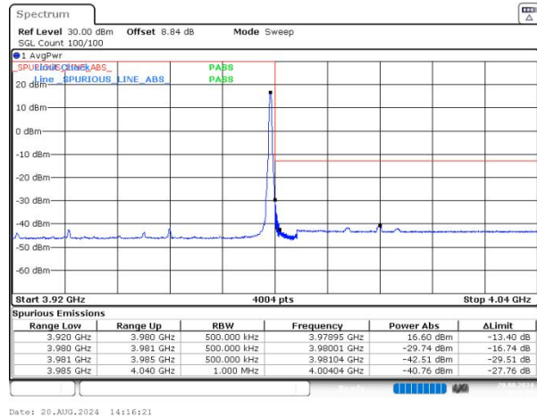
n77(3700-3980) SCS=30kHz DFT_QPSK BW=60MHz HighChannel=663332 RB=1@161 NVNT
