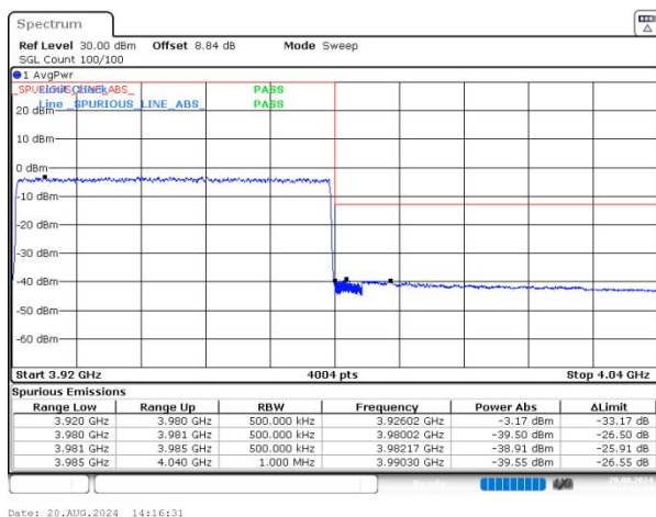
n77(3700-3980) SCS=30kHz DFT_QPSK BW=60MHz HighChannel=663332 RB=162@0 NVNT
