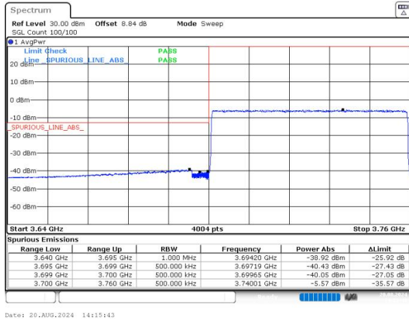
n77(3700-3980) SCS=30kHz CP_QPSK BW=60MHz LowChannel=648668 RB=162@0 NVNT
