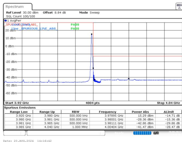
n77(3700-3980) SCS=30kHz DFT_16QAM BW=60MHz HighChannel=663332 RB=1@161 NVNT
