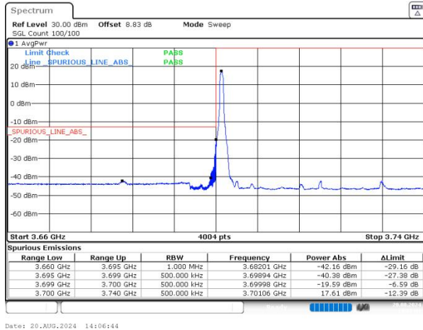
n77(3700-3980) SCS=30kHz DFT_BPSK BW=40MHz LowChannel=648000 RB=1@0 NVNT
