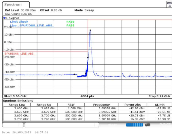
n77(3700-3980) SCS=30kHz DFT_QPSK BW=40MHz LowChannel=648000 RB=1@0 NVNT
