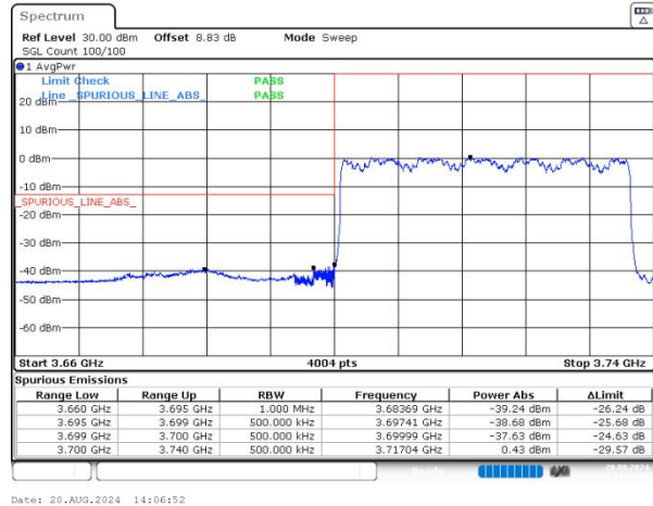
n77(3700-3980) SCS=30kHz DFT_BPSK BW=40MHz LowChannel=648000 RB=100@0 NVNT
