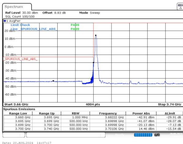
n77(3700-3980) SCS=30kHz DFT_16QAM BW=40MHz LowChannel=648000 RB=1@0 NVNT
