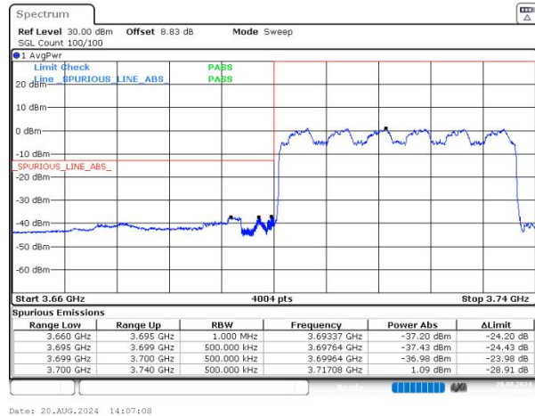
n77(3700-3980) SCS=30kHz DFT_QPSK BW=40MHz LowChannel=648000 RB=100@0 NVNT
