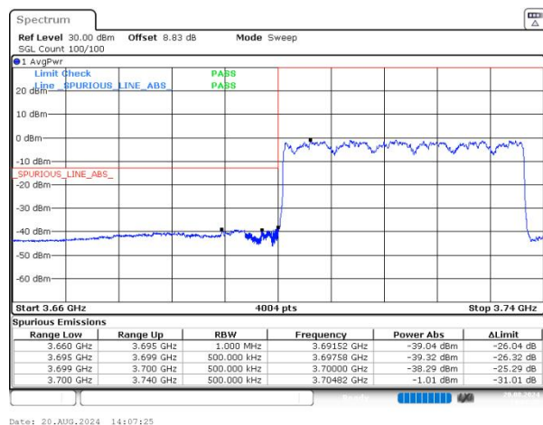
n77(3700-3980) SCS=30kHz DFT_16QAM BW=40MHz LowChannel=648000 RB=100@0 NVNT
