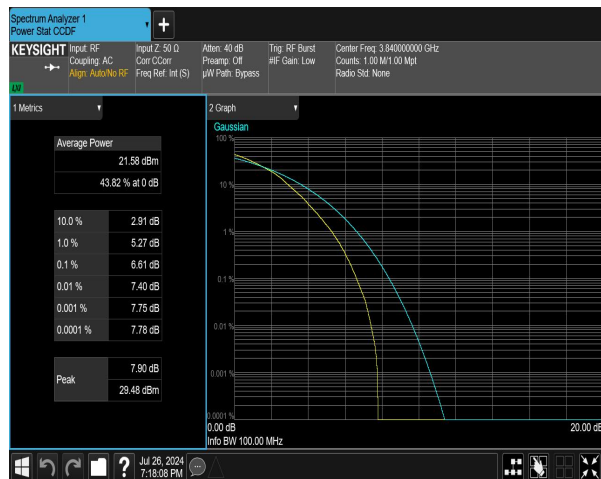
n77(3700-3980) SCS=30kHz DFT_64QAM BW=20MHz Channel=656000 RB=50@0 NVNT
