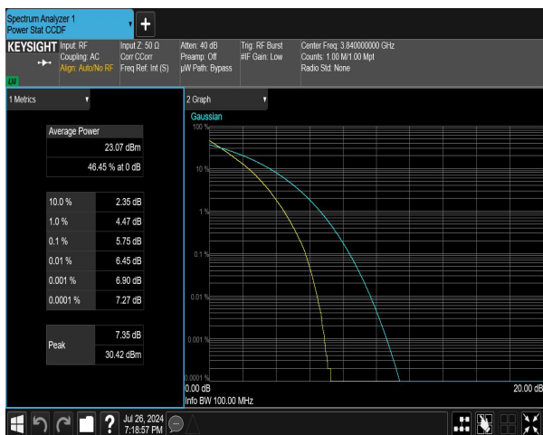
n77(3700-3980) SCS=30kHz DFT_QPSK BW=60MHz Channel=656000 RB=162@0 NVNT
