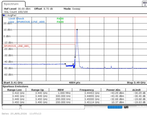
n77(3450-3550) SCS=30kHz DFT_256QAM BW=40MHz LowChannel=631334 RB=1@0 NVNT
