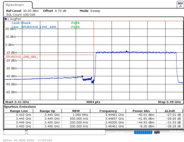
n77(3450-3550) SCS=30kHz DFT_256QAM BW=40MHz LowChannel=631334 RB=100@0 NVNT
