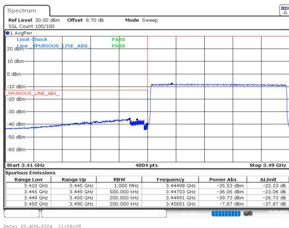
n77(3450-3550) SCS=30kHz CP_QPSK BW=40MHz LowChannel=631334 RB=106@0 NVNT
