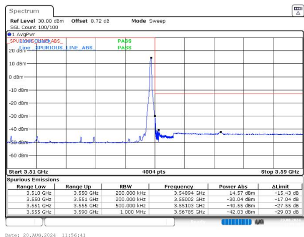
n77(3450-3550) SCS=30kHz DFT_BPSK BW=40MHz HighChannel=635332 RB=1@105 NVNT
