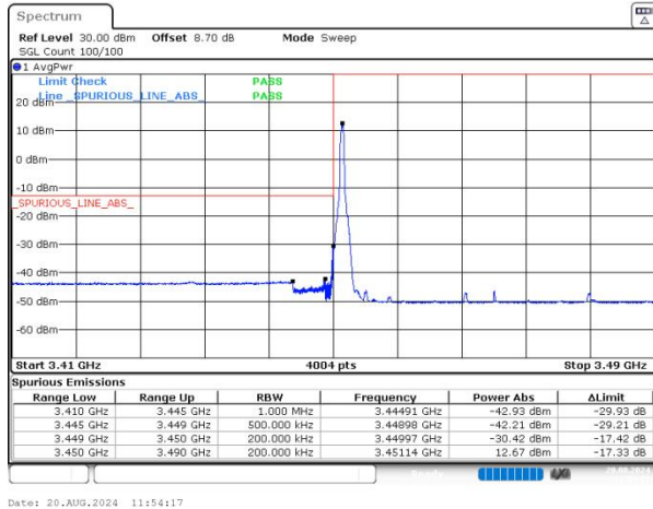
n77(3450-3550) SCS=30kHz DFT_64QAM BW=40MHz LowChannel=631334 RB=1@0 NVNT
