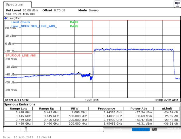
n77(3450-3550) SCS=30kHz DFT_64QAM BW=40MHz LowChannel=631334 RB=100@0 NVNT
