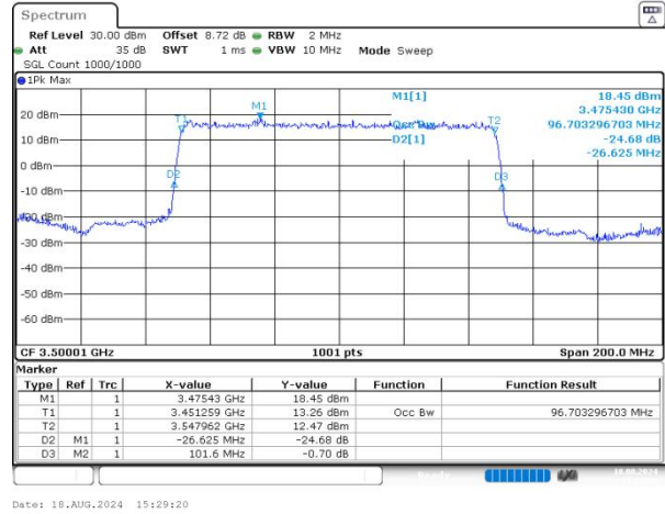
n77(3450-3550) SCS=30kHz DFT_BPSK BW=100MHz Channel=633334 RB=270@0 NVNT
