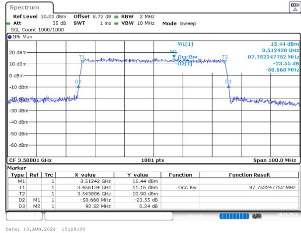
n77(3450-3550) SCS=30kHz CP_64QAM BW=90MHz Channel=633334 RB=245@0 NVNT
