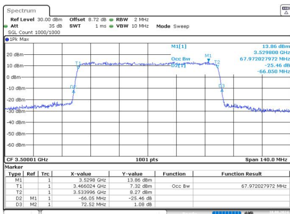
n77(3450-3550) SCS=30kHz CP_16QAM BW=70MHz Channel=633334 RB=189@0 NVNT
