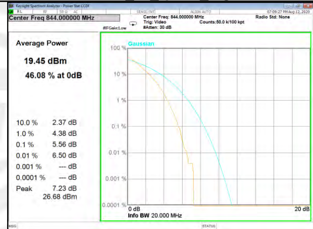
Band5_50_Q16_High
