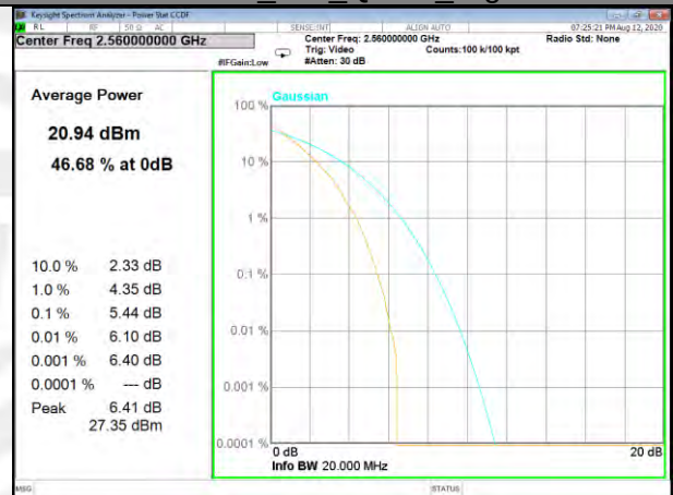
Band7_100_Q16_High
