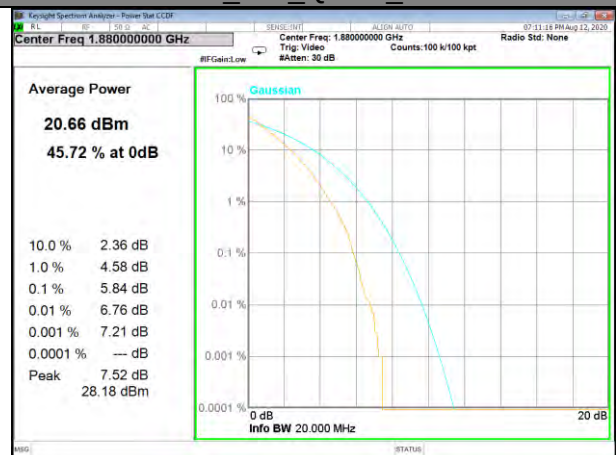
Band2_100_QPSK_Middle
