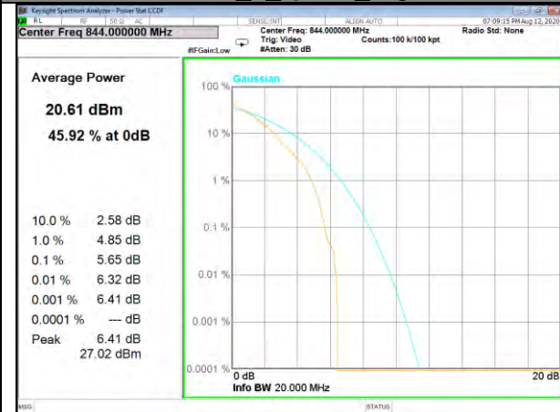
Band5_1_Q16_High
