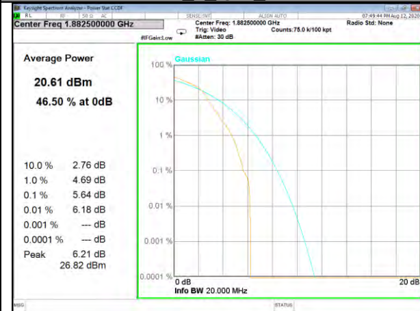
Band25_1_QPSK_High
