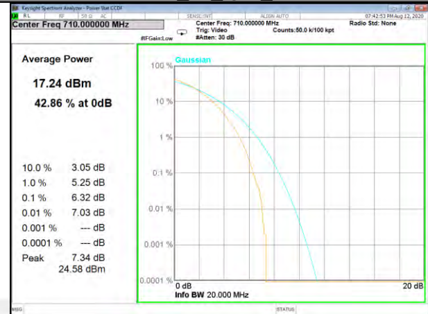
Band17_50_QPSK_High
