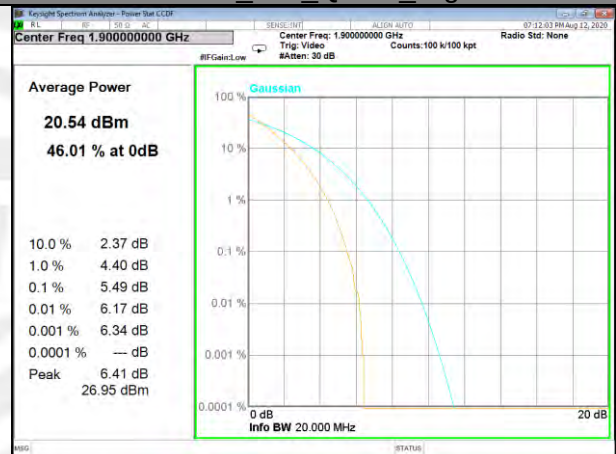
Band2_100_Q16_High
