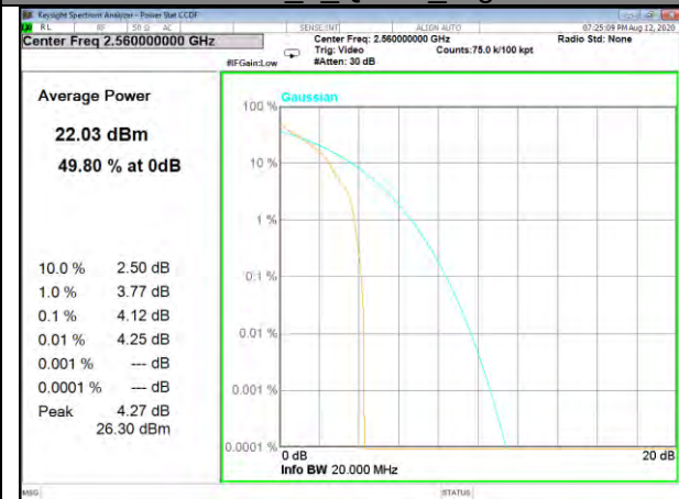
Band7_1_Q16_High
