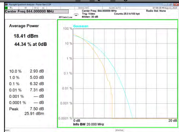
Band5_50_Q16_High
