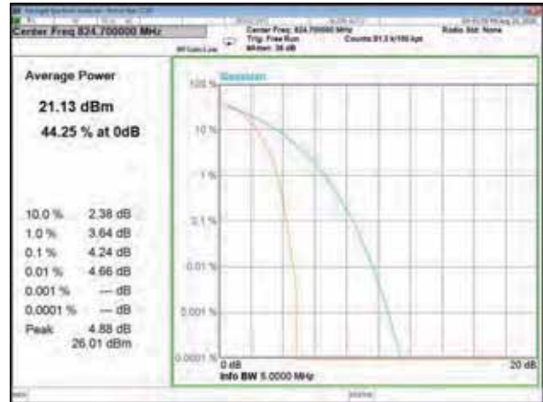
EVDO BC0Low Channel
