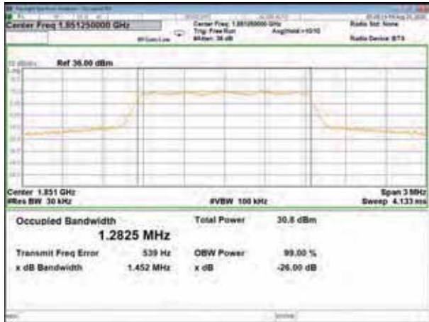
BC1 CDMA Lower 26BW and 99%
