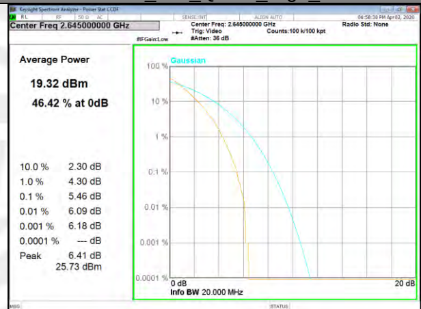
B41_100_Q16_High_
