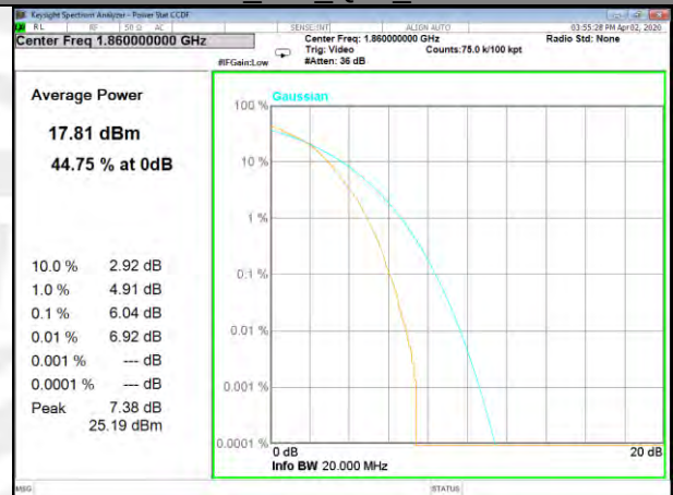
B25_100_QPSK_Middle
