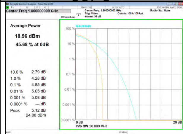
B25_1_QPSK_Middle
