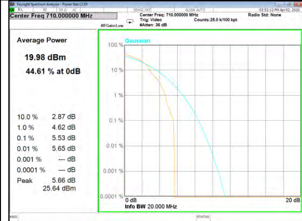
B17_1_QPSK_High
