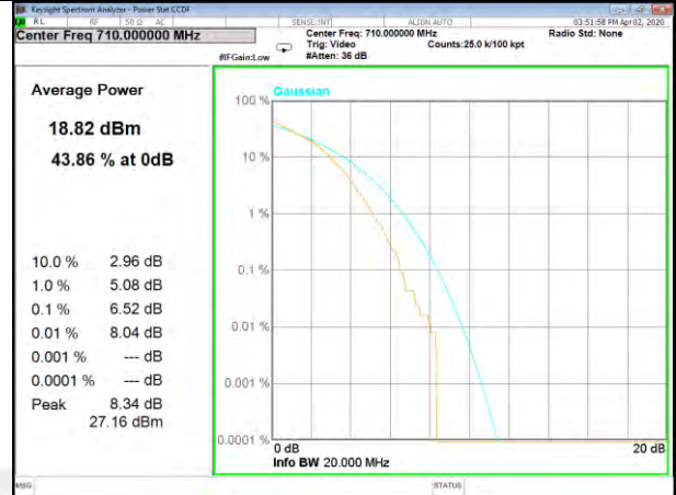
B17_50_QPSK_High
