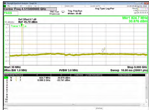
GPRS_850_Lower_Conducted_Spurious
