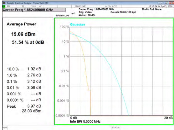
HSPA B2_Lower
