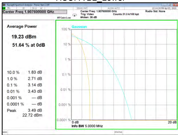
HSPA B2_Higher
