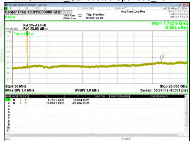
HSDPA B4_Conducted Spurious_High
