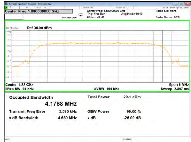
WCDMA B2 26BW and 99% Middle
