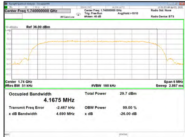
WCDMA B4 26BW and 99% Middle
