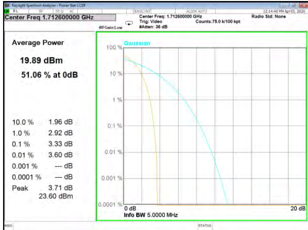
HSUPA B4_Lower
