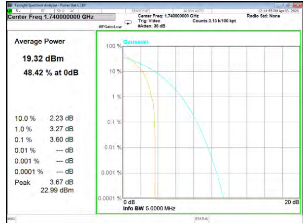
HSUPA B4_Middle
