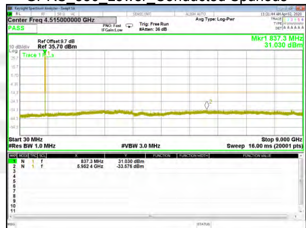
GPRS_850_Middle_Conducted_Spurious
