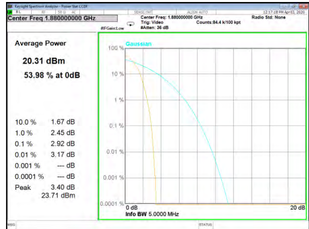
WCDMA B2_Middle
