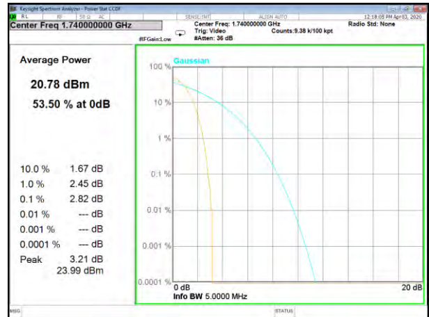
WCDMA B4_Middle
