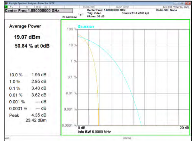
HSPA B2_Middle
