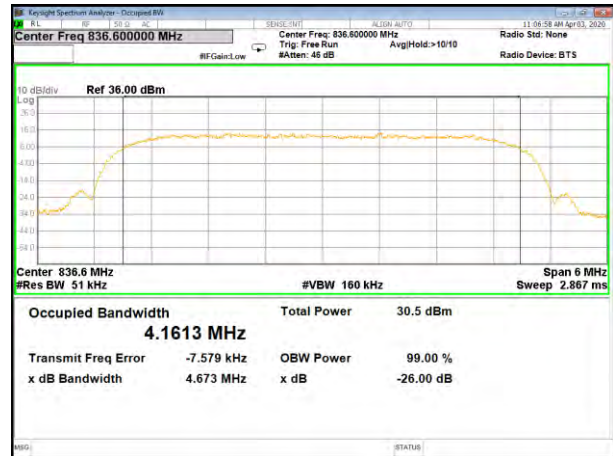
WCDMA B5 26BW and 99% Middle
