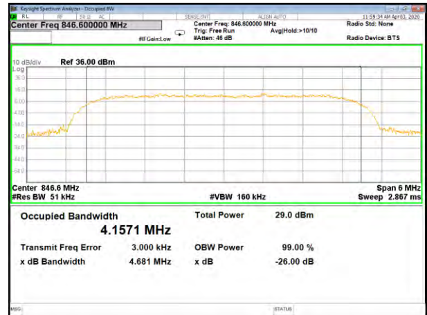
HSUPA B5_26BW and 99%_High
