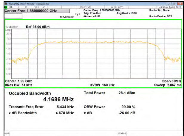
HSUPA B2_26BW and 99%_Middle
