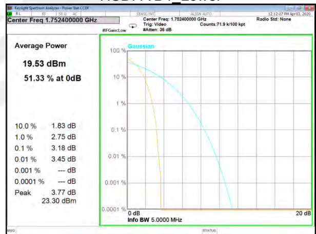
HSDPA B4_Higher
