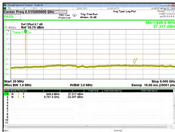
EGPRS 850_Higher_Conducted_Spurious
