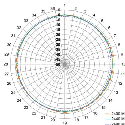
XY-Plane Gain
