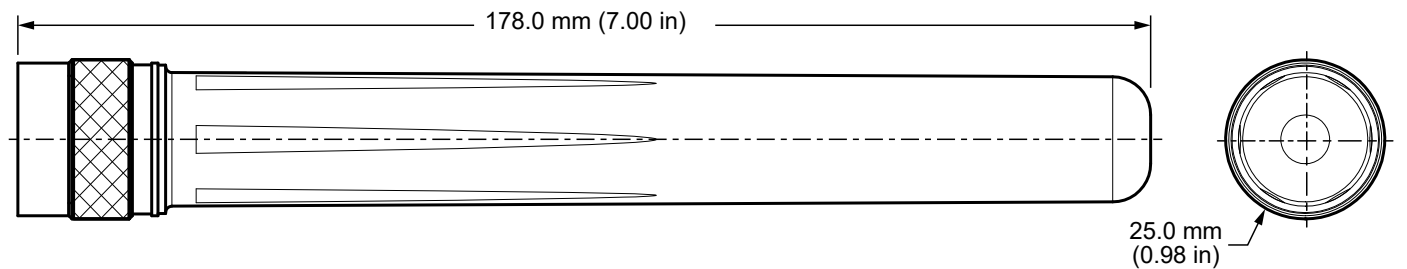
Figure 1. ANT-W63-IPW1-NP Antenna Dimensions
