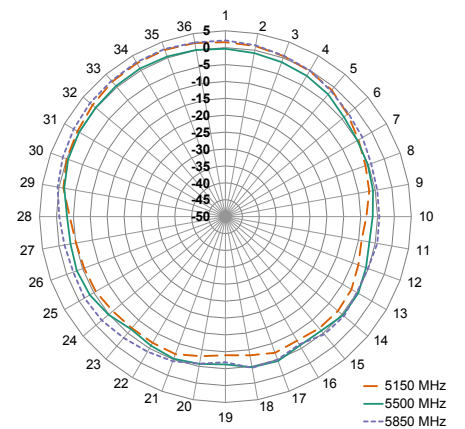
XY-Plane Gain
