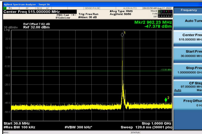
Band12-10MHz-QPSK-23060-1RB#0-30~1000MHz
