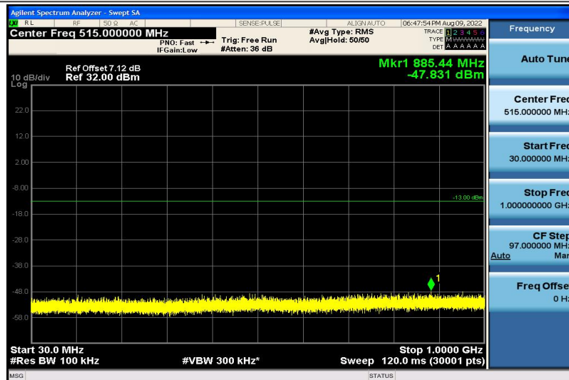
Band2-15MHz-QPSK-18675-1RB#0-30~1000MHz
