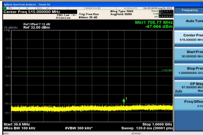
Band2-10MHz-QPSK-18650-1RB#0-30~1000MHz
