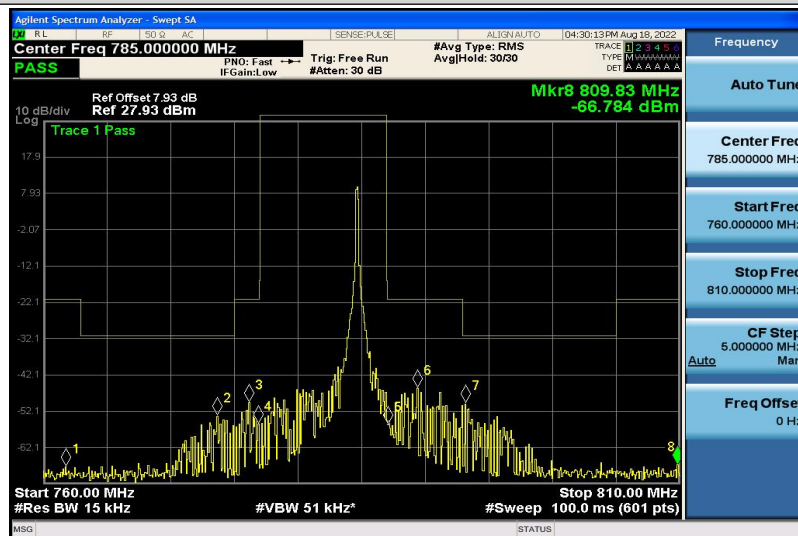
Band13-5MHz-16QAM-23255-1RB#5
