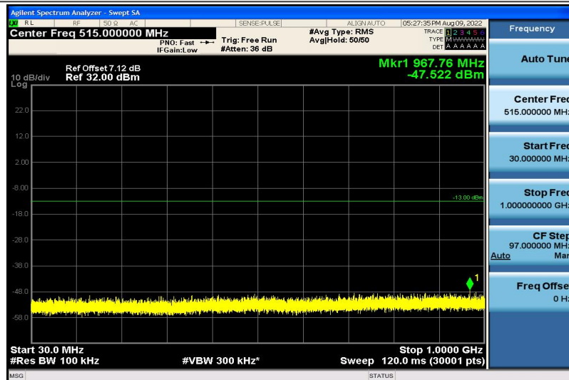
Band2-1.4MHz-16QAM-18607-1RB#0-30~1000MHz
