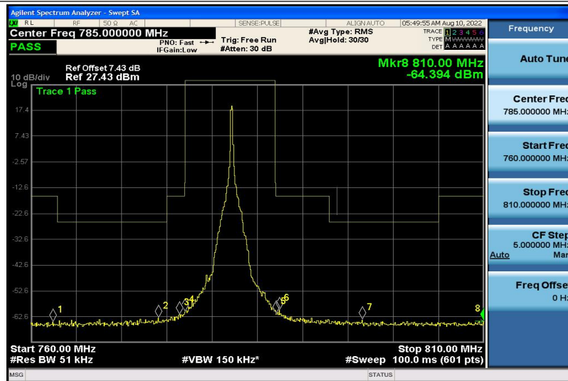
Band13-5MHz-16QAM-23230-1RB#5
