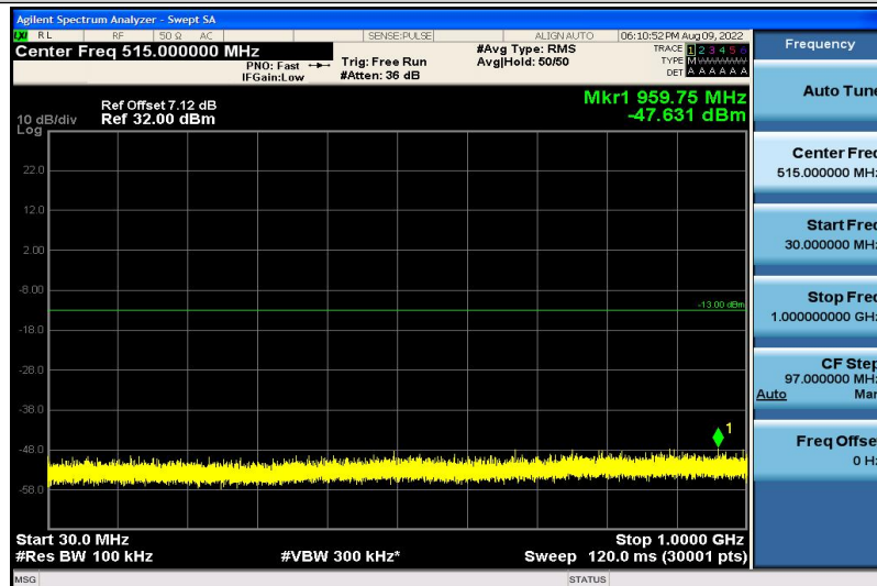
Band2-5MHz-16QAM-18625-1RB#0-30~1000MHz
