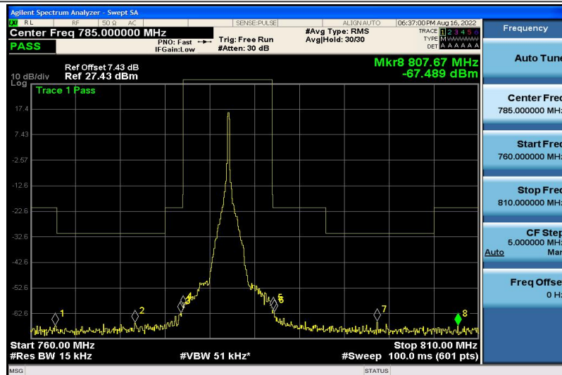
Band13-10MHz-QPSK-23230-1RB#5
