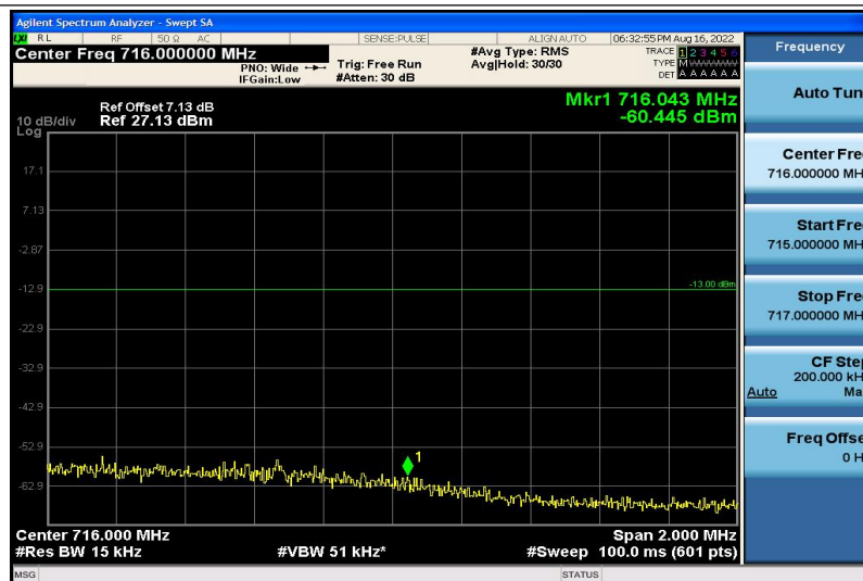
Band12-10MHz-16QAM-23130-1RB#5
