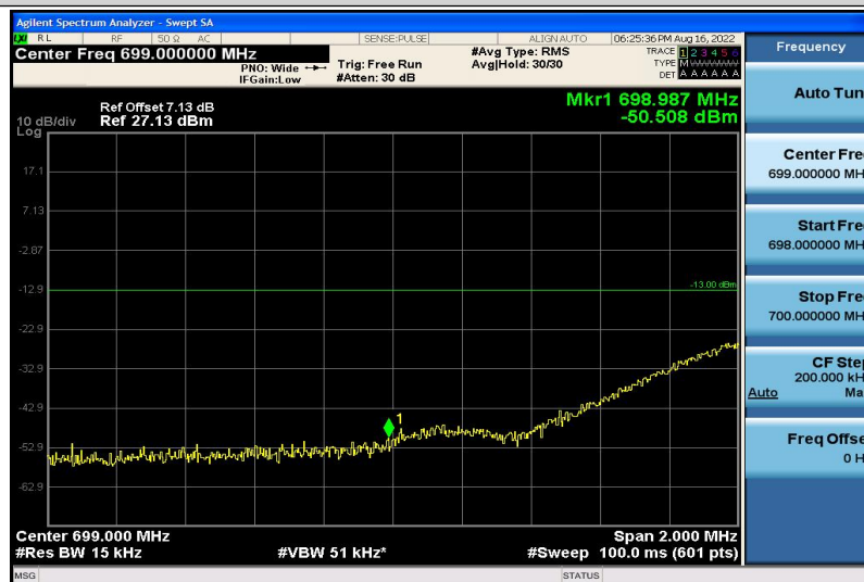
Band12-3MHz-QPSK-23025-1RB#5
