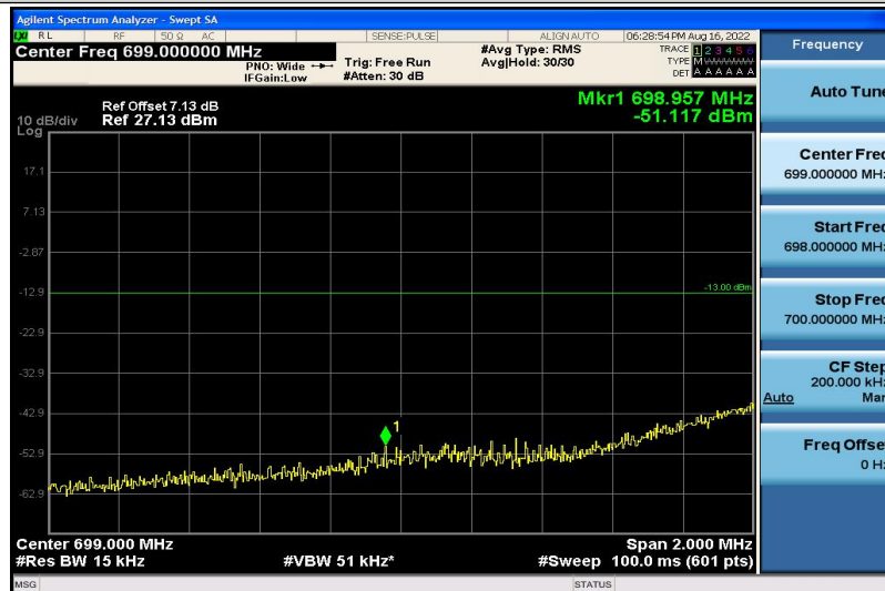
Band12-5MHz-16QAM-23035-1RB#5
