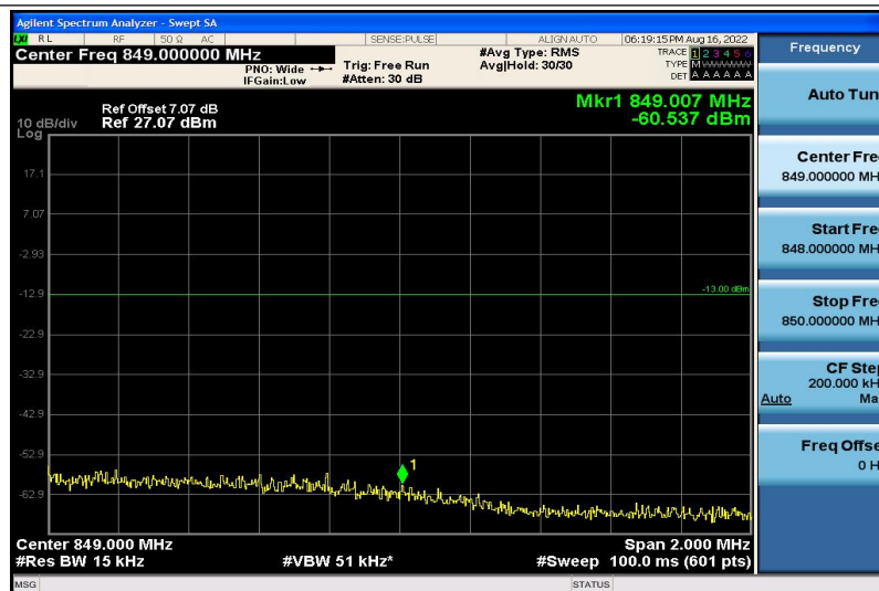
Band5-10MHz-QPSK-20600-1RB#5
