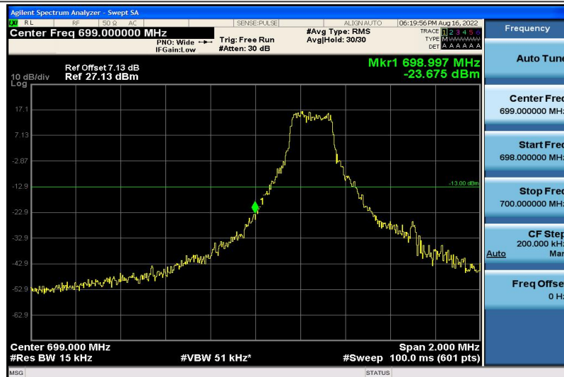
Band12-1.4MHz-QPSK-23017-1RB#0
