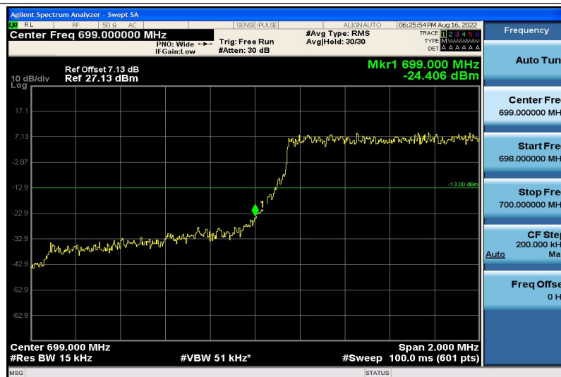
Band12-3MHz-QPSK-23025-6RB#0
