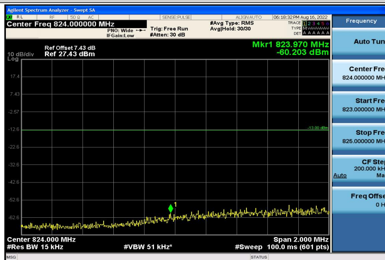
Band5-10MHz-16QAM-20450-1RB#5
