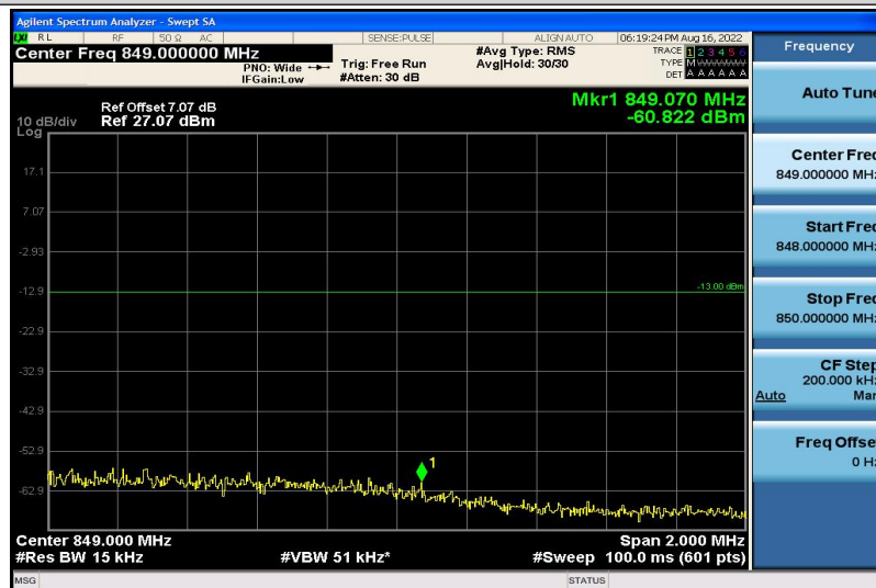
Band5-10MHz-16QAM-20600-1RB#5
