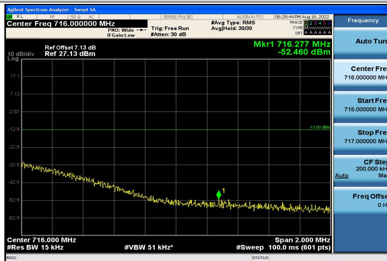
Band12-5MHz-16QAM-23155-1RB#5
