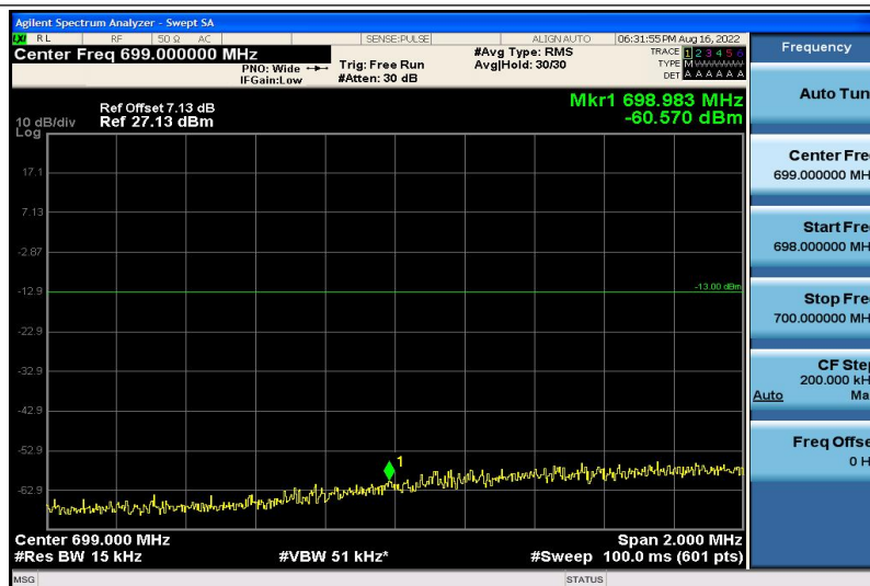
Band12-10MHz-QPSK-23060-1RB#5
