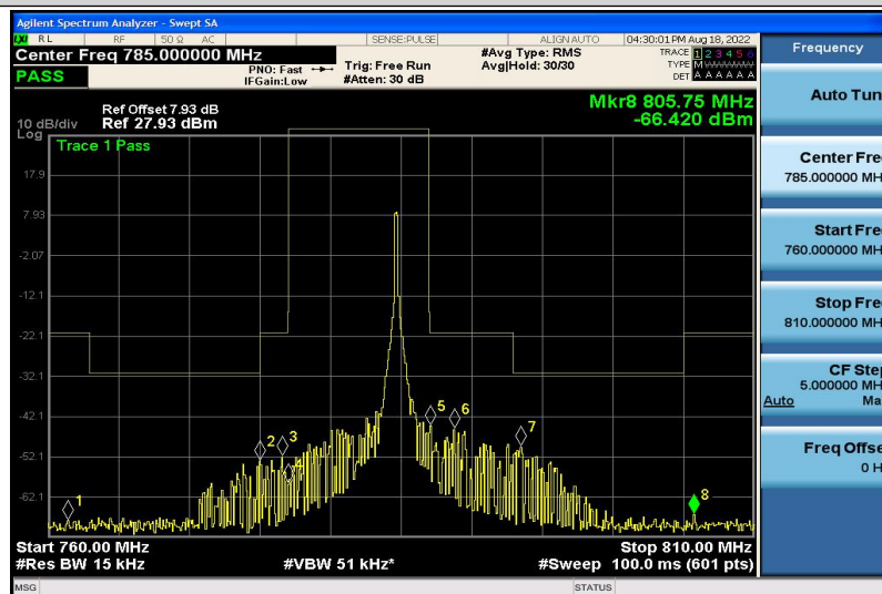
Band13-5MHz-QPSK-23255-1RB#5
