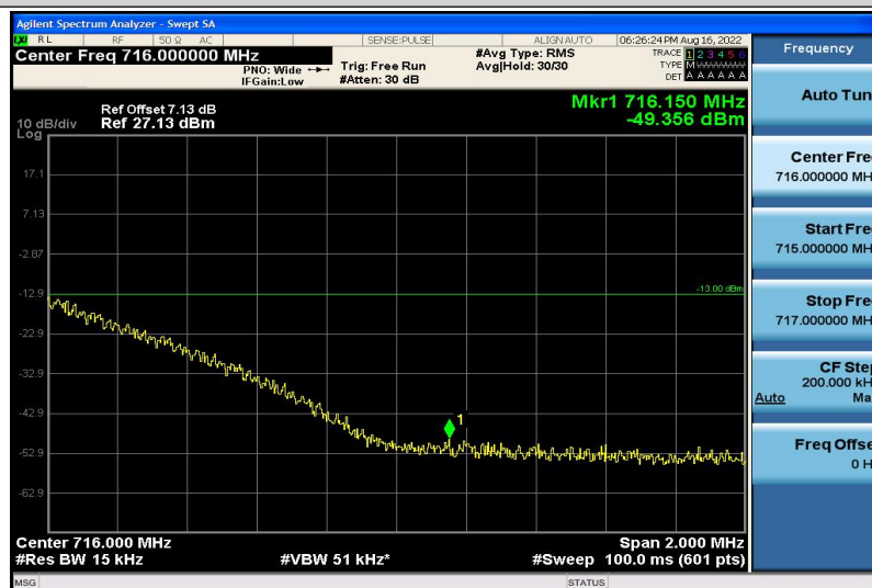
Band12-3MHz-QPSK-23165-1RB#5
