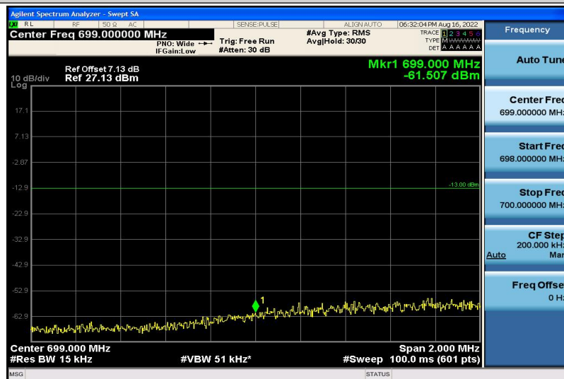
Band12-10MHz-16QAM-23060-1RB#5
