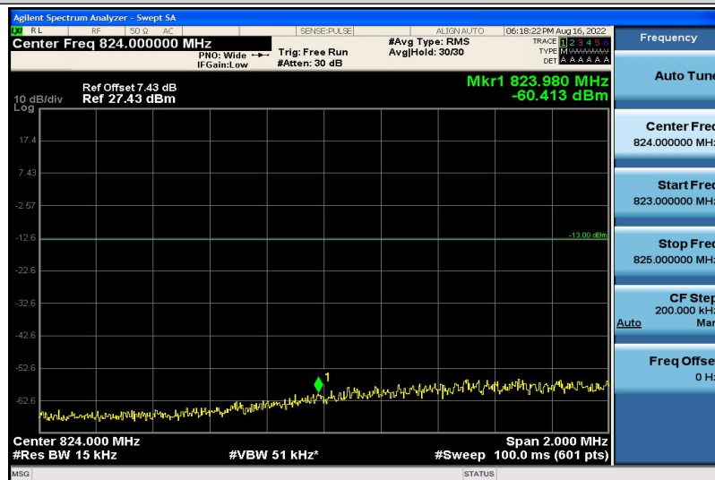
Band5-10MHz-QPSK-20450-1RB#5
