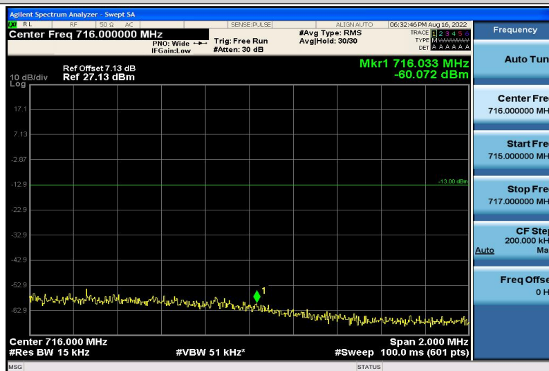
Band12-10MHz-QPSK-23130-1RB#5
