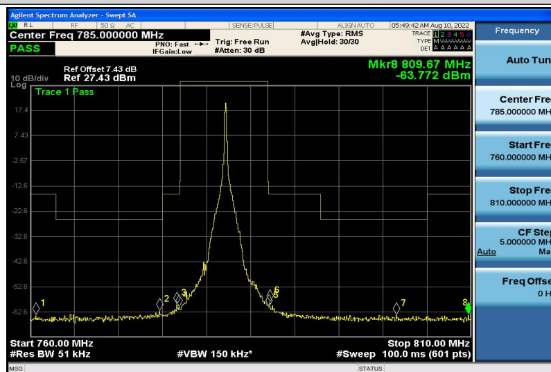
Band13-5MHz-QPSK-23230-1RB#5
