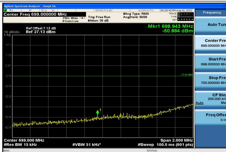
Band12-5MHz-QPSK-23035-1RB#5
