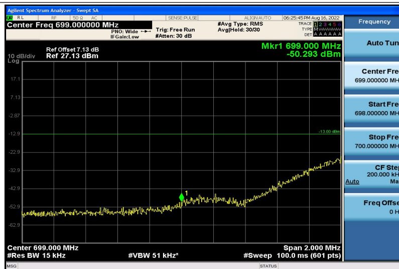
Band12-3MHz-16QAM-23025-1RB#5
