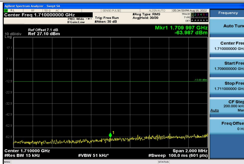
Band4-15MHz-16QAM-20025-1RB#5
