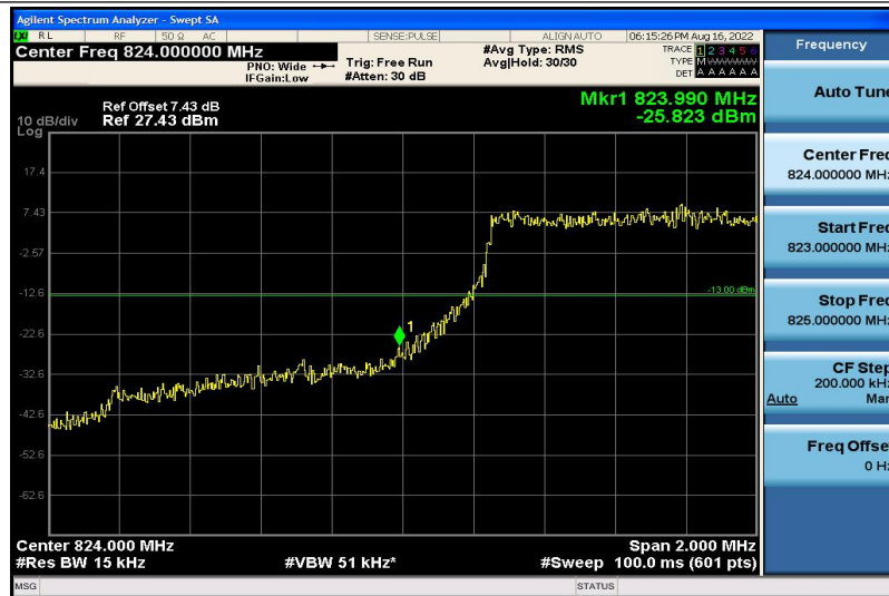
Band5-5MHz-QPSK-20425-6RB#0
