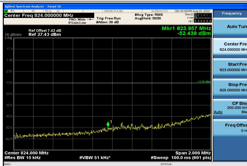
Band5-5MHz-QPSK-20425-1RB#5
