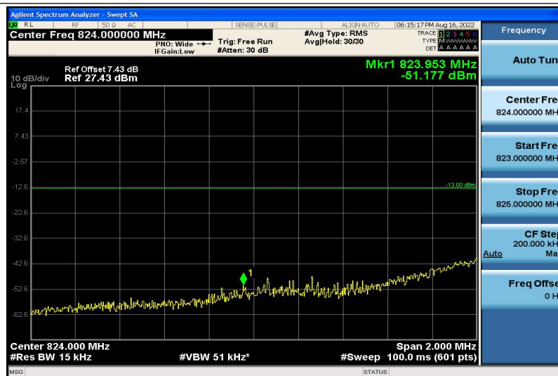
Band5-5MHz-16QAM-20425-1RB#5
