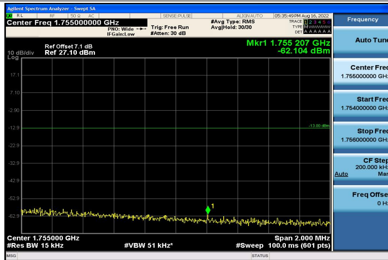
Band4-15MHz-16QAM-20325-1RB#5
