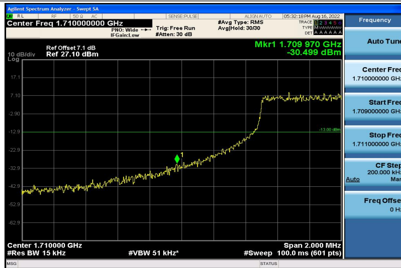
Band4-10MHz-16QAM-20000-6RB#0
