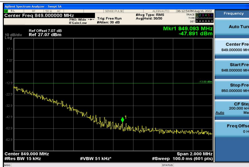
Band5-3MHz-16QAM-20635-1RB#5
