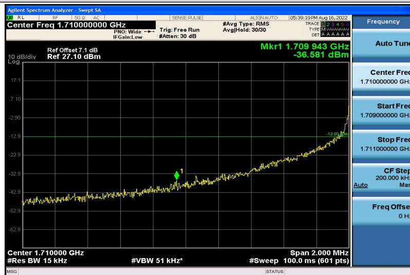
Band4-20MHz-16QAM-20050-6RB#0
