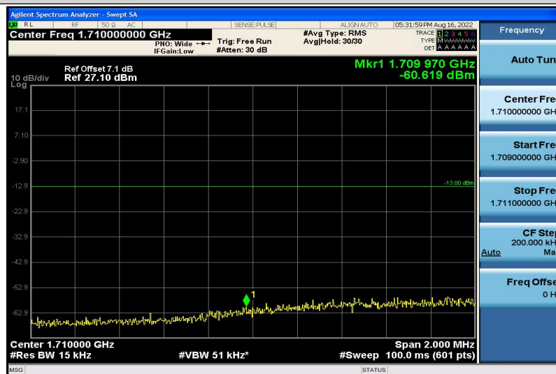
Band4-10MHz-16QAM-20000-1RB#5
