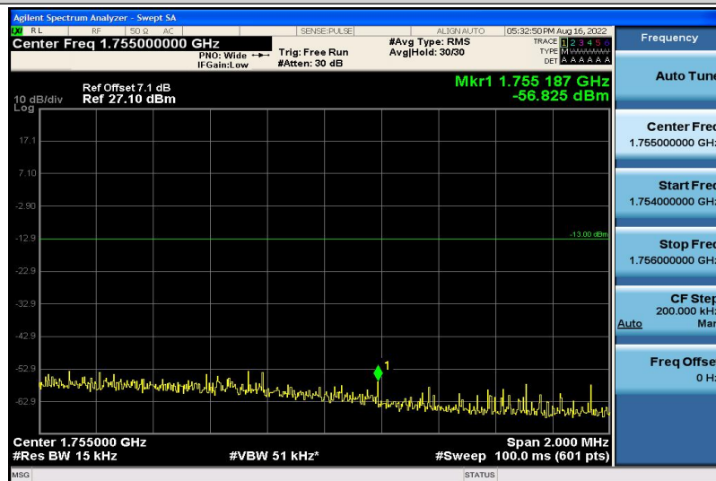
Band4-10MHz-16QAM-20350-1RB#5
