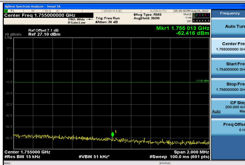
Band4-15MHz-QPSK-20325-1RB#5
