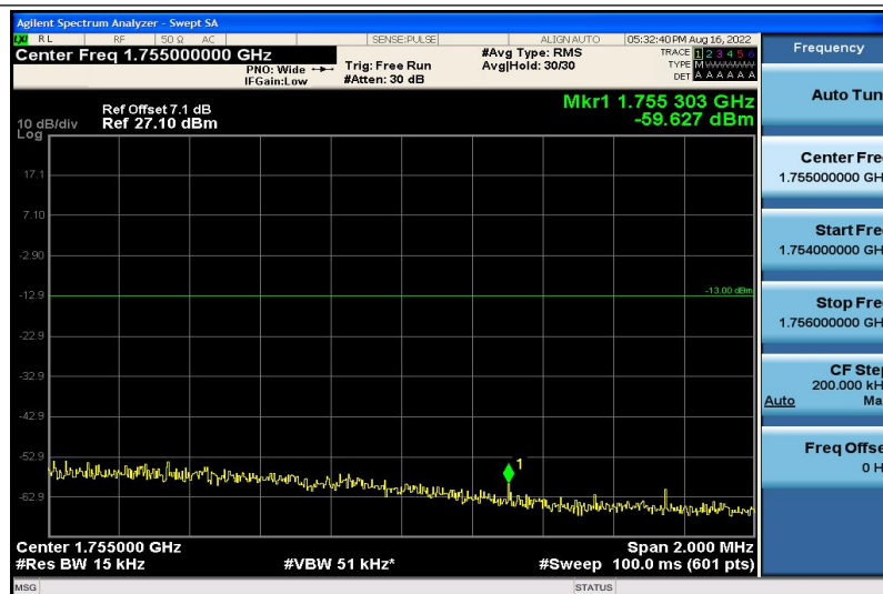
Band4-10MHz-QPSK-20350-1RB#5
