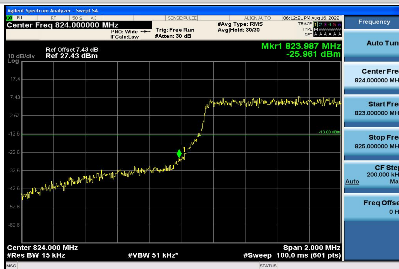
Band5-3MHz-16QAM-20415-6RB#0
