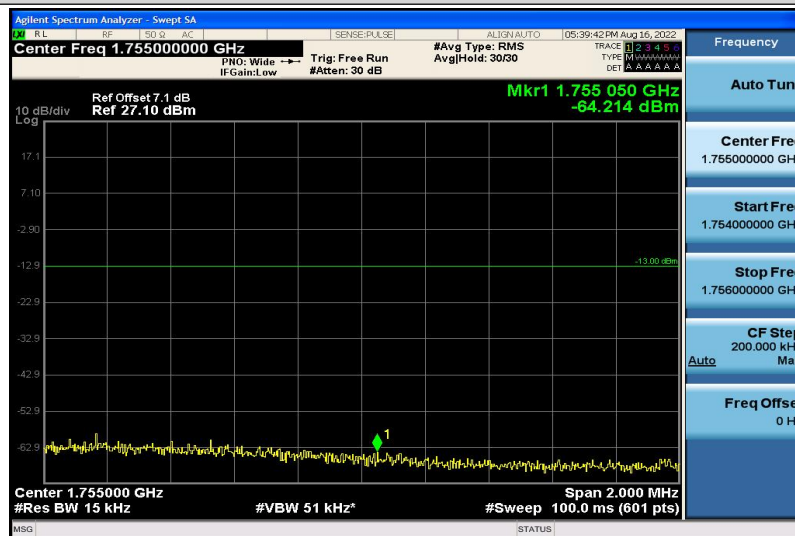
Band4-20MHz-QPSK-20300-1RB#5
