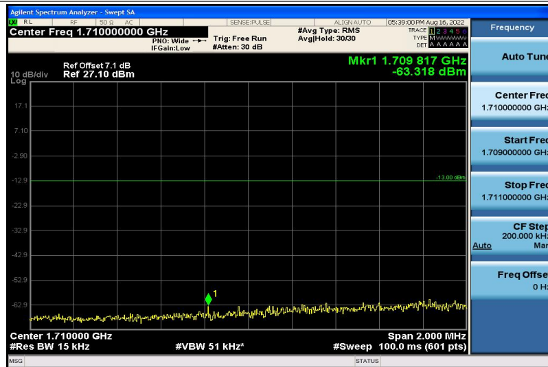
Band4-20MHz-16QAM-20050-1RB#5
