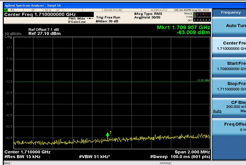
Band4-15MHz-QPSK-20025-1RB#5
