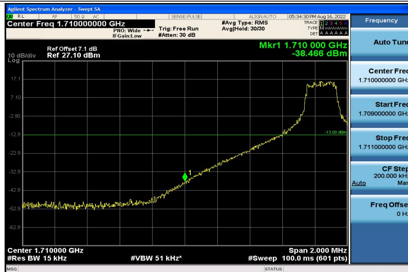
Band4-15MHz-QPSK-20025-1RB#0
