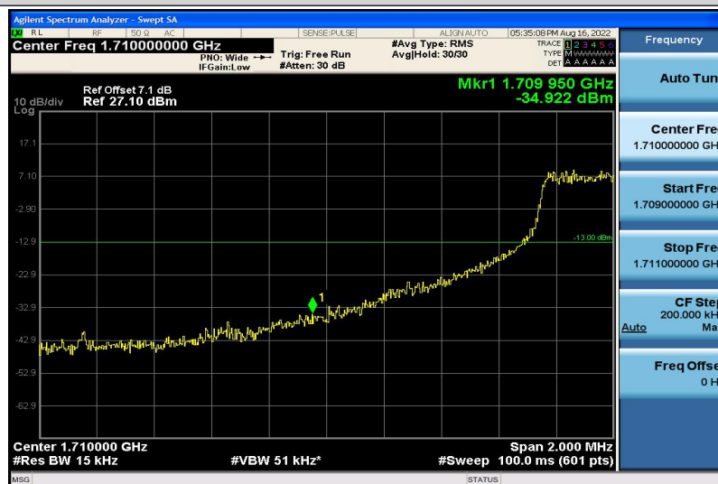
Band4-15MHz-QPSK-20025-6RB#0
