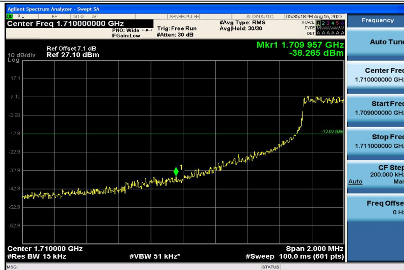
Band4-15MHz-16QAM-20025-6RB#0
