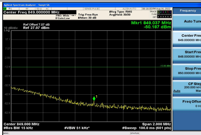
Band5-5MHz-QPSK-20625-1RB#5
