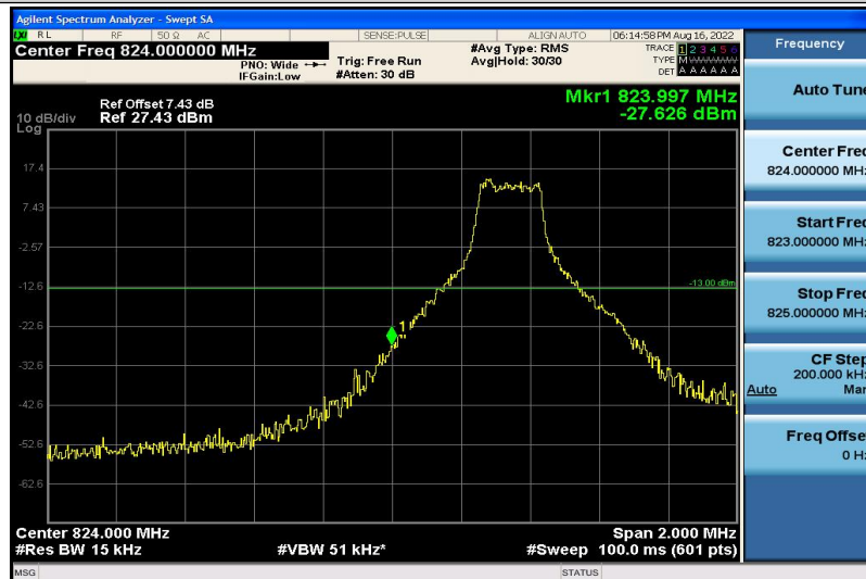
Band5-5MHz-16QAM-20425-1RB#0
