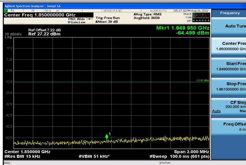
Band2-15MHz-16QAM-18675-1RB#5
