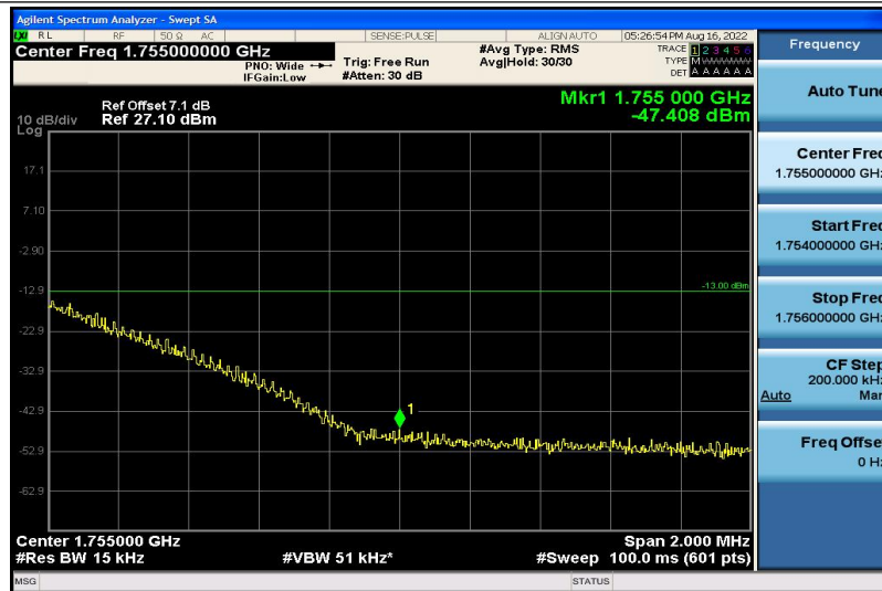
Band4-3MHz-16QAM-20385-1RB#5
