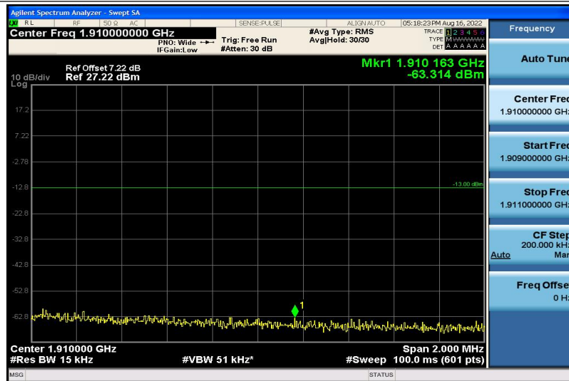
Band2-15MHz-16QAM-19125-1RB#5
