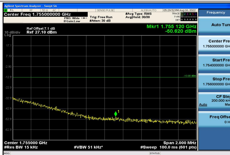
Band4-5MHz-16QAM-20375-1RB#5
