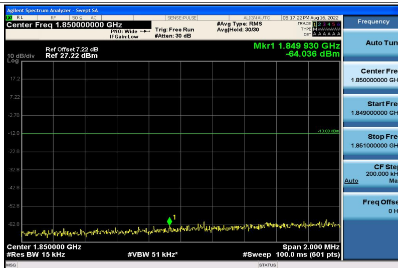
Band2-15MHz-QPSK-18675-1RB#5
