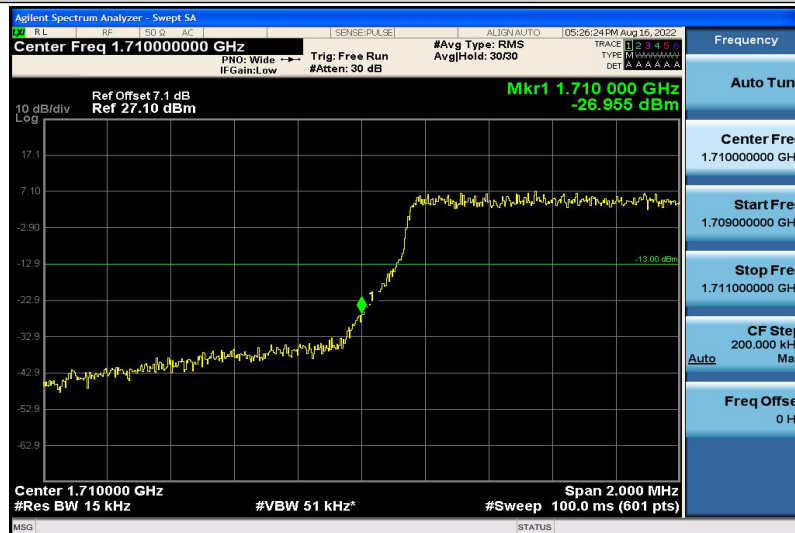
Band4-3MHz-16QAM-19965-6RB#0
