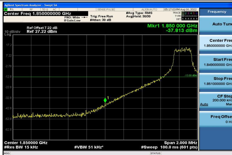
Band2-15MHz-QPSK-18675-1RB#0
