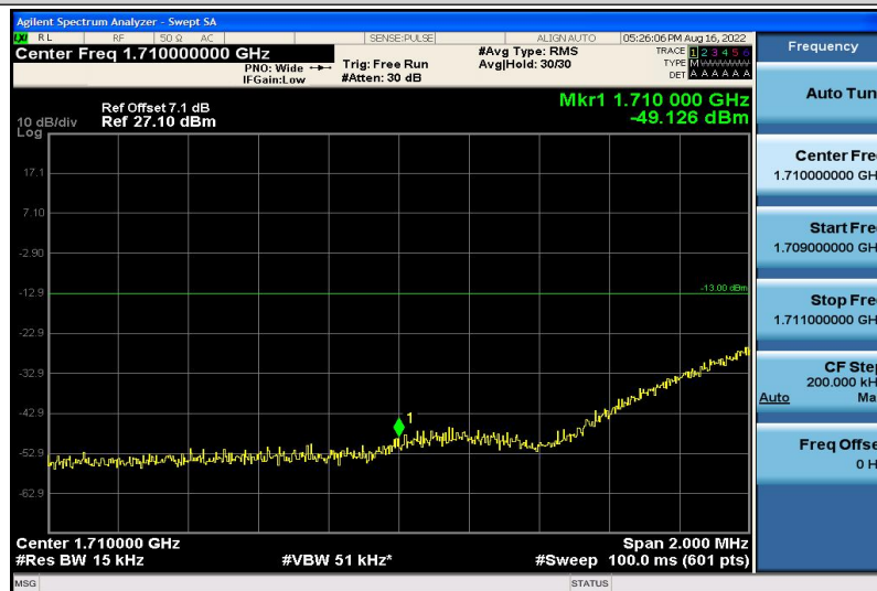
Band4-3MHz-16QAM-19965-1RB#5
