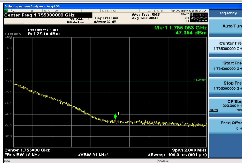
Band4-3MHz-QPSK-20385-1RB#5
