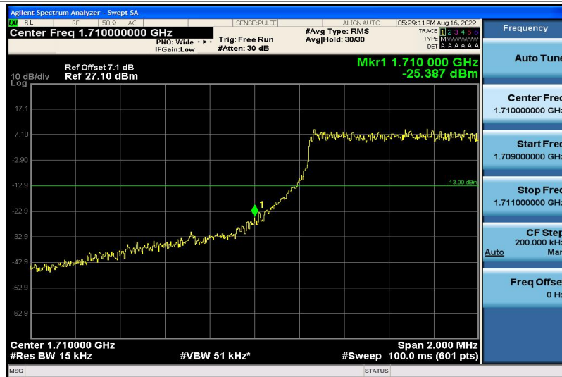
Band4-5MHz-QPSK-19975-6RB#0
