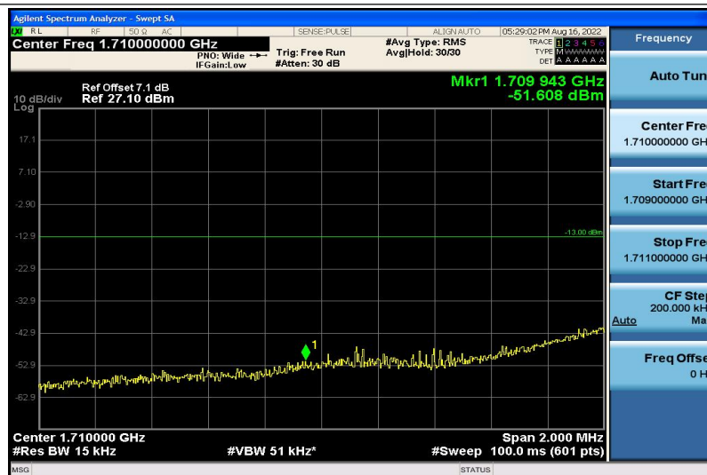
Band4-5MHz-16QAM-19975-1RB#5
