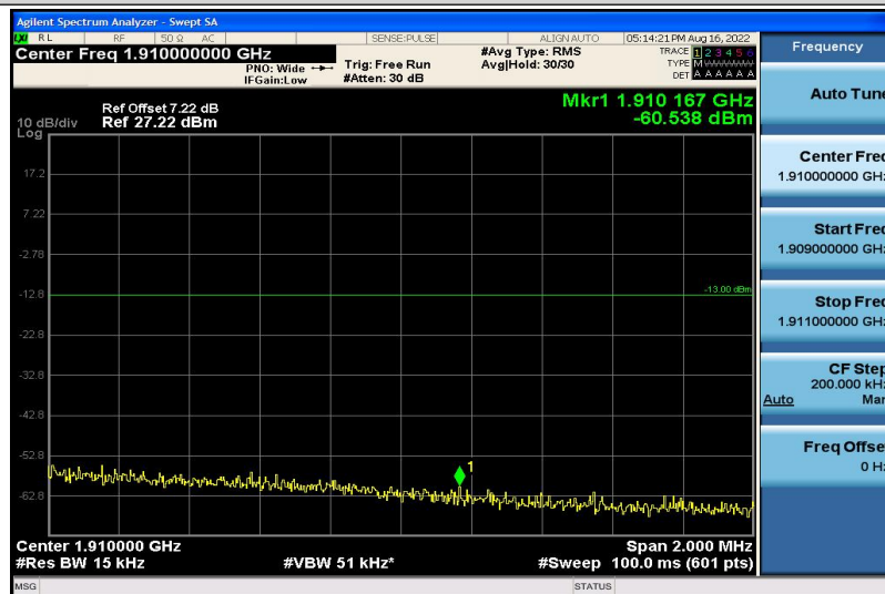
Band2-10MHz-16QAM-19150-1RB#5
