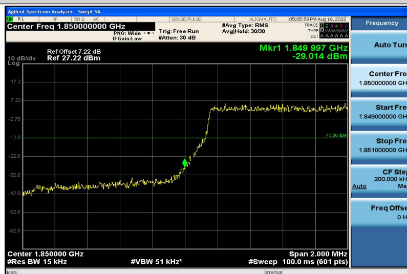
Band2-3MHz-16QAM-18615-6RB#0
