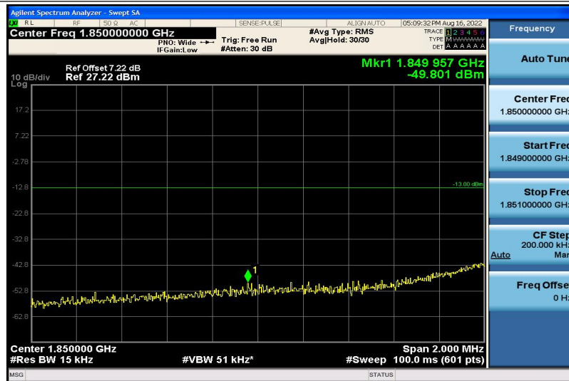
Band2-5MHz-16QAM-18625-1RB#5
