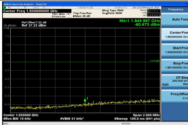
Band2-10MHz-16QAM-18650-1RB#5
