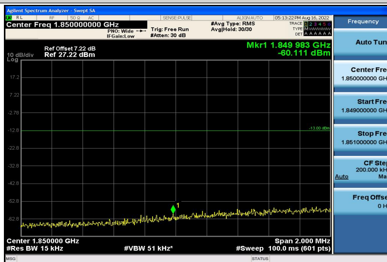
Band2-10MHz-QPSK-18650-1RB#5
