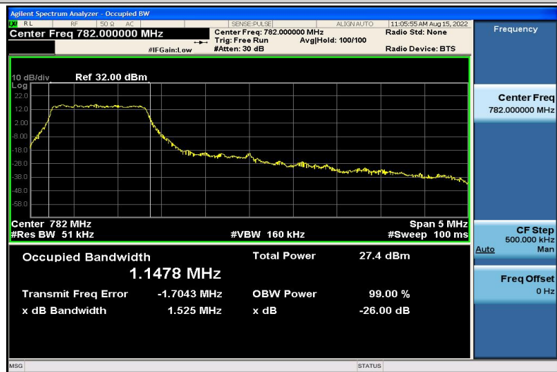
Band13-5MHz-16QAM-23230-6RB#0-1.1478
