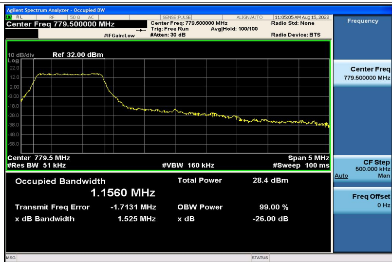
Band13-5MHz-QPSK-23205-6RB#0-1.1560
