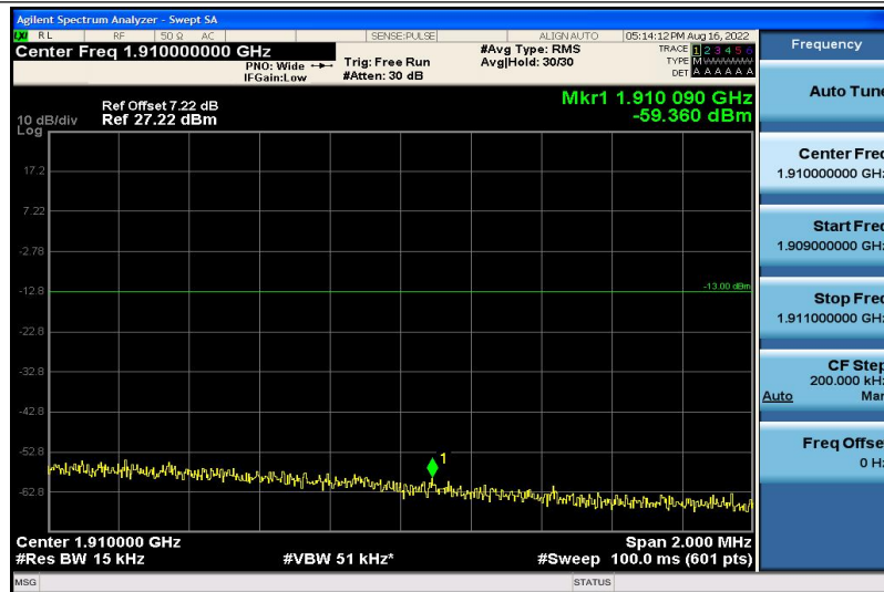
Band2-10MHz-QPSK-19150-1RB#5
