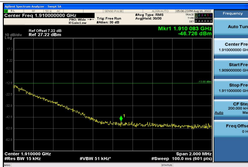
Band2-3MHz-16QAM-19185-1RB#5
