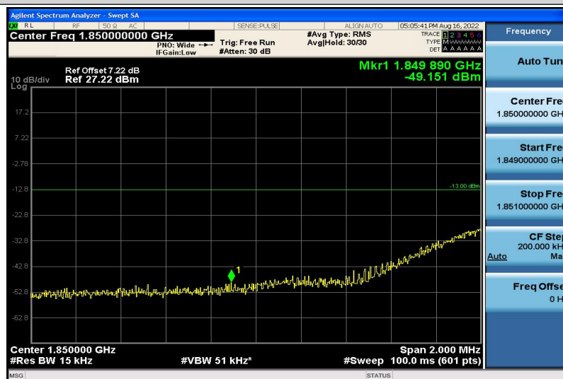
Band2-3MHz-16QAM-18615-1RB#5
