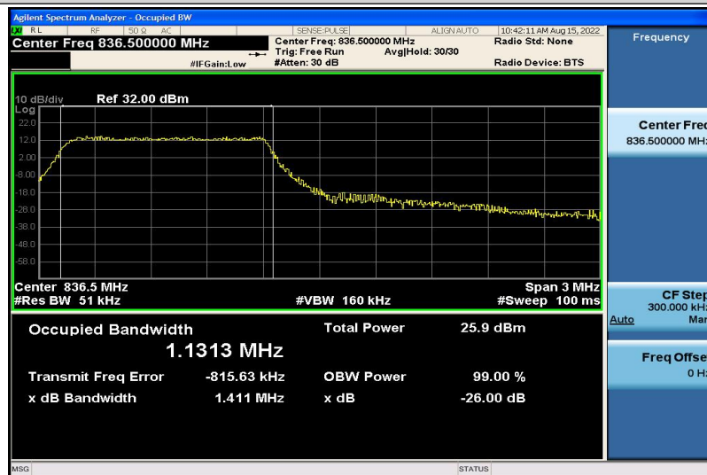
Band5-3MHz-16QAM-20525-6RB#0-1.1313
