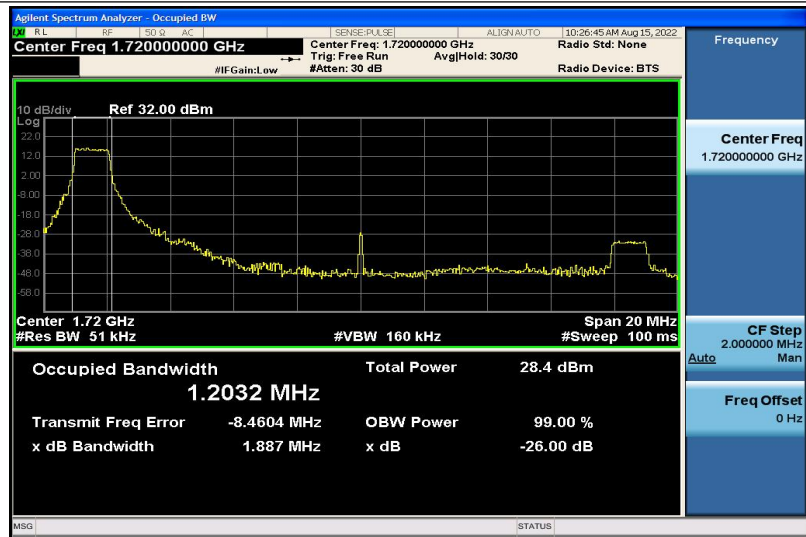
Band4-20MHz-16QAM-20050-6RB#0-1.2032
