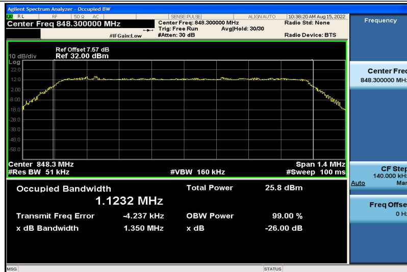
Band5-1.4MHz-16QAM-20643-6RB#0-1.1232
