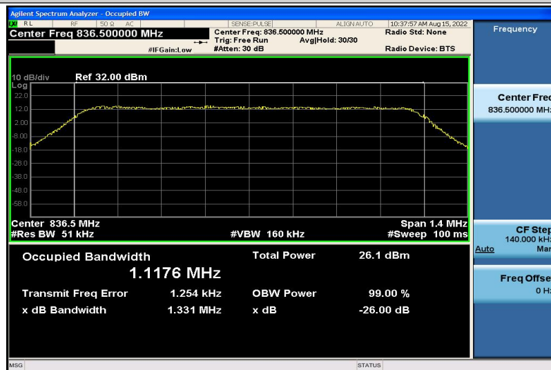
Band5-1.4MHz-16QAM-20525-6RB#0-1.1176
