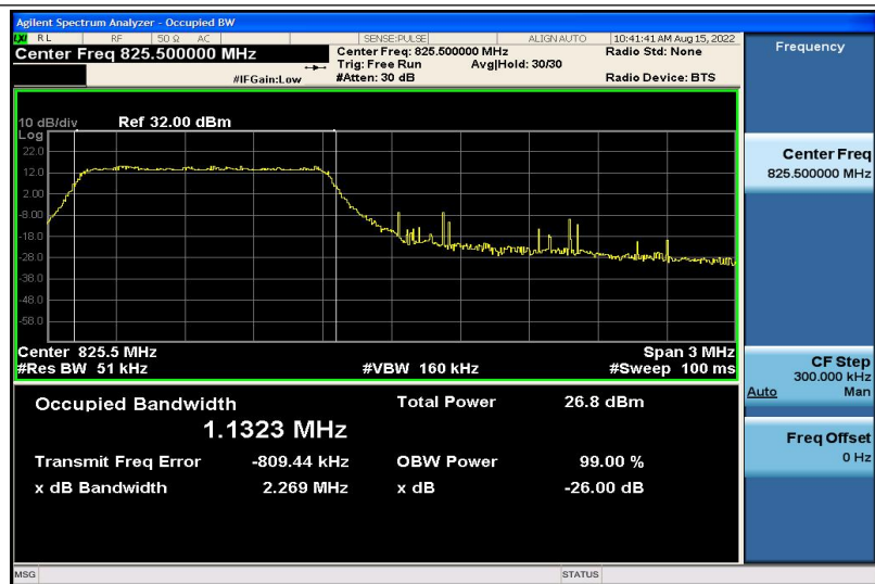
Band5-3MHz-QPSK-20415-6RB#0-1.1323
