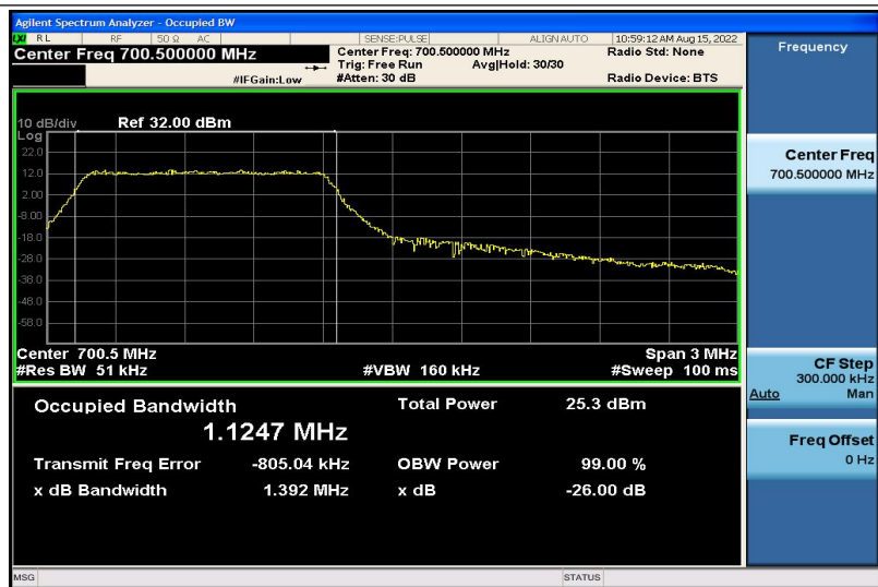
Band12-3MHz-16QAM-23025-6RB#0-1.1247
