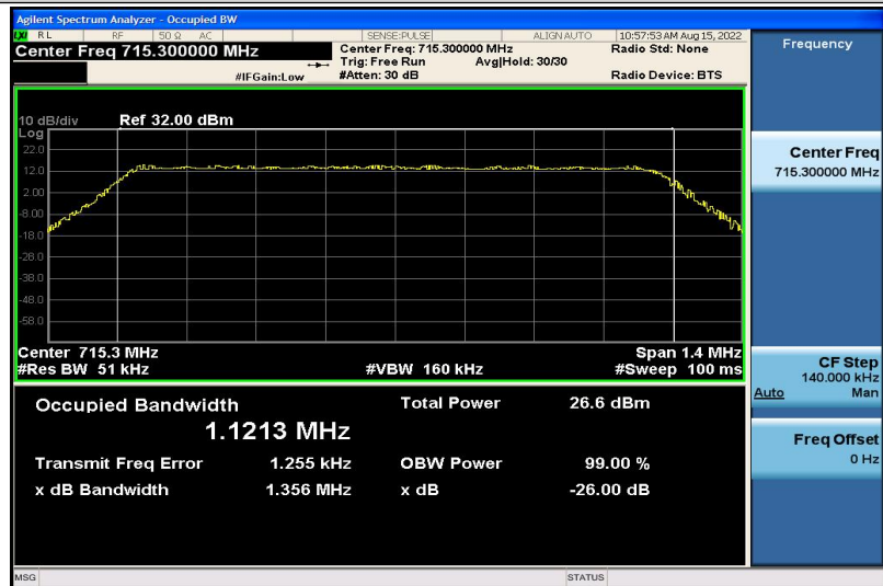
Band12-1.4MHz-QPSK-23173-6RB#0-1.1213
