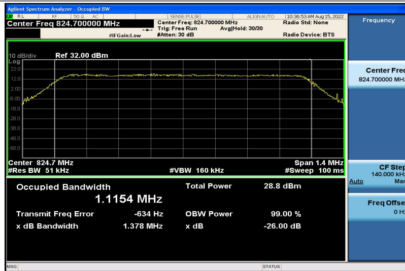
Band5-1.4MHz-16QAM-20407-6RB#0-1.1154
