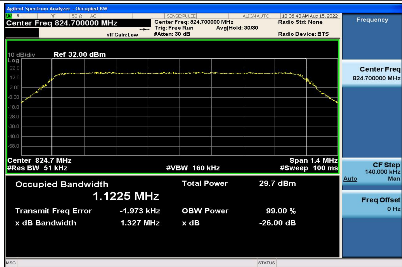
Band5-1.4MHz-QPSK-20407-6RB#0-1.1225
