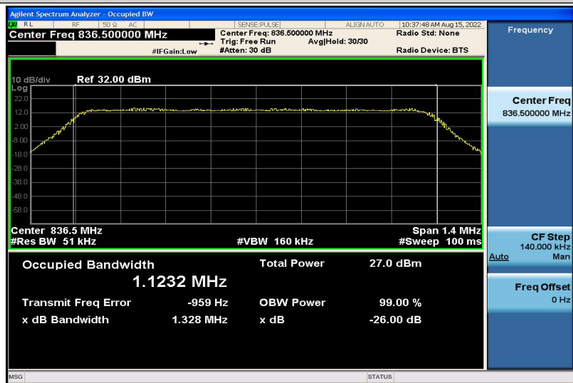
Band5-1.4MHz-QPSK-20525-6RB#0-1.1232
