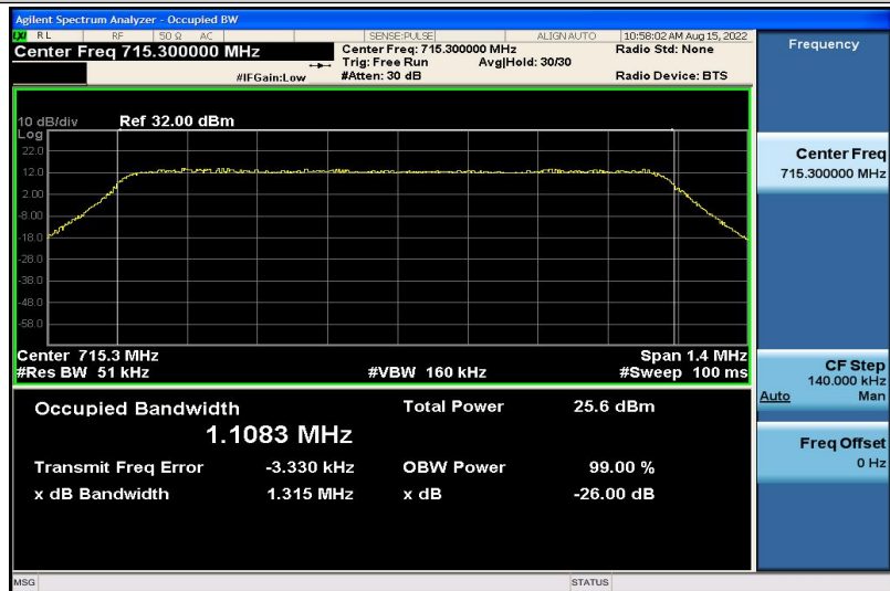
Band12-1.4MHz-16QAM-23173-6RB#0-1.1083
