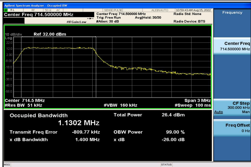
Band12-3MHz-QPSK-23165-6RB#0-1.1302
