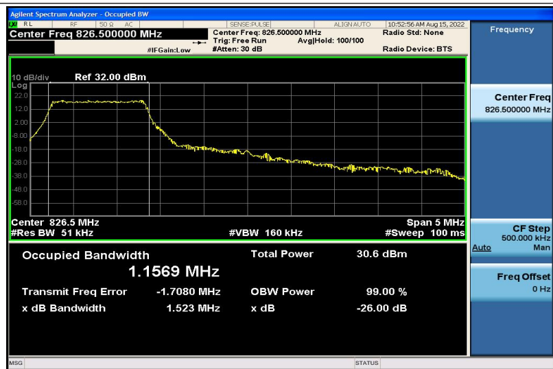
Band5-5MHz-QPSK-20425-6RB#0-1.1569
