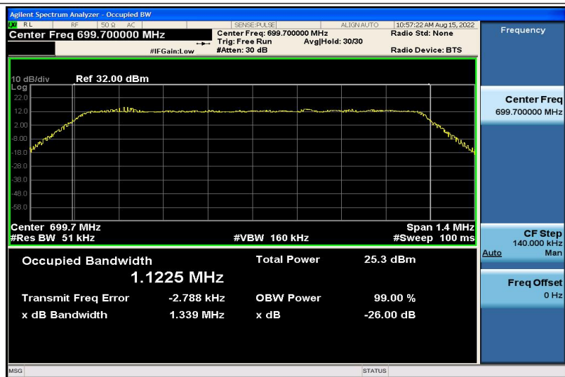
Band12-1.4MHz-16QAM-23017-6RB#0-1.1225
