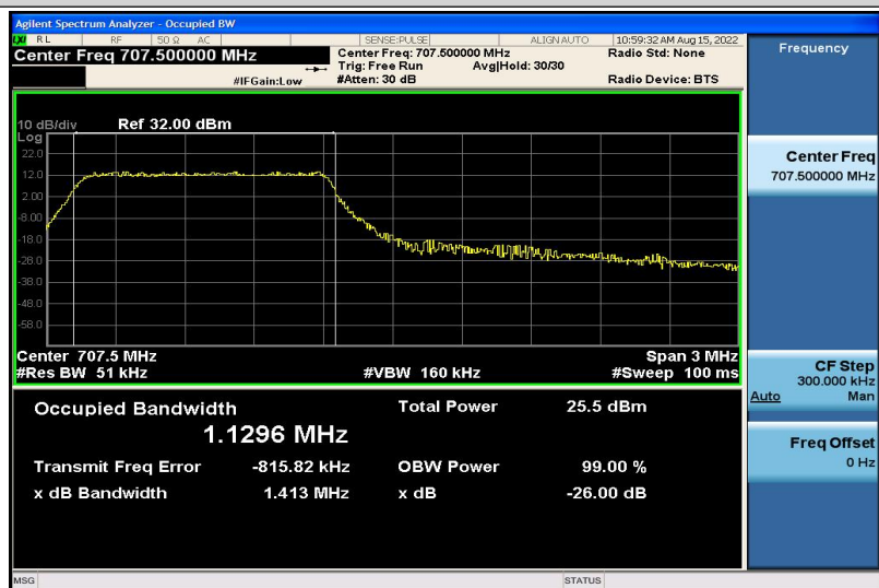
Band12-3MHz-16QAM-23095-6RB#0-1.1296
