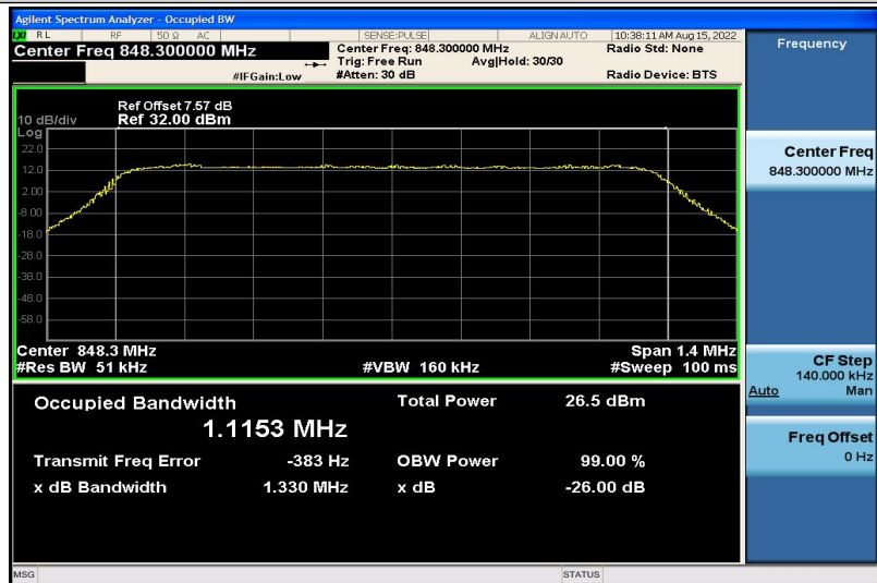
Band5-1.4MHz-QPSK-20643-6RB#0-1.1153
