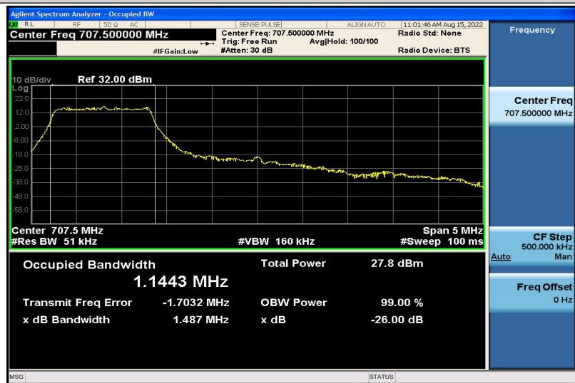
Band12-5MHz-QPSK-23095-6RB#0-1.1443
