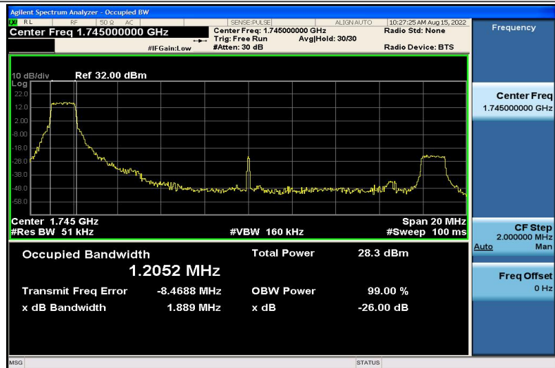
Band4-20MHz-16QAM-20300-6RB#0-1.2052
