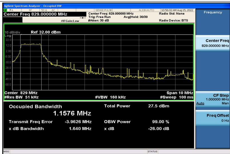
Band5-10MHz-QPSK-20450-6RB#0-1.1576
