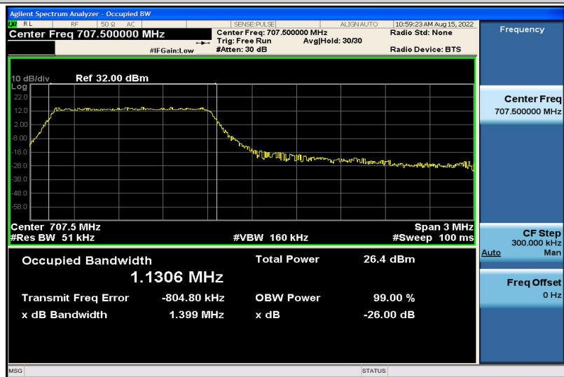
Band12-3MHz-QPSK-23095-6RB#0-1.1306
