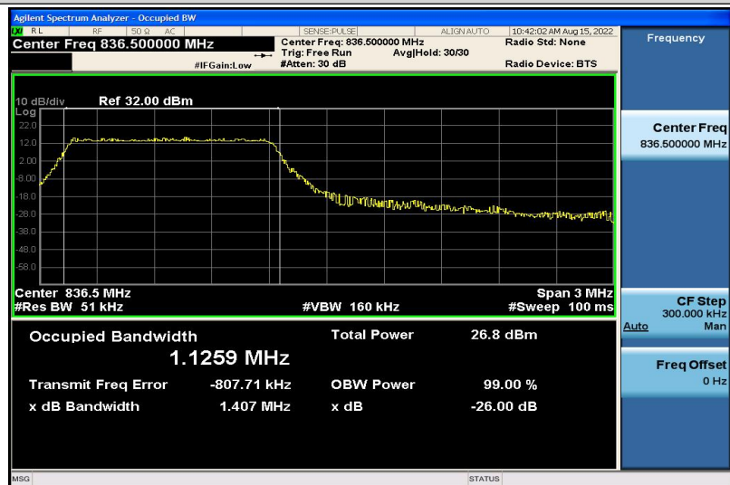
Band5-3MHz-QPSK-20525-6RB#0-1.1259
