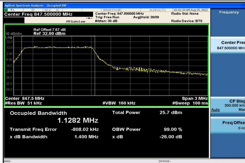
Band5-3MHz-16QAM-20635-6RB#0-1.1282
