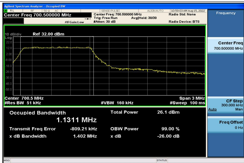
Band12-3MHz-QPSK-23025-6RB#0-1.1311
