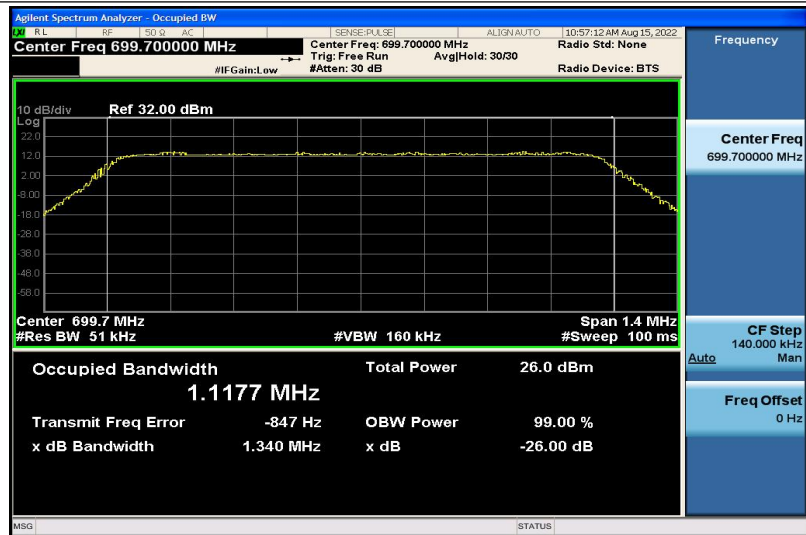
Band12-1.4MHz-QPSK-23017-6RB#0-1.1177
