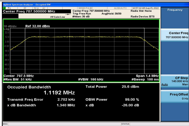
Band12-1.4MHz-16QAM-23095-6RB#0-1.1192
