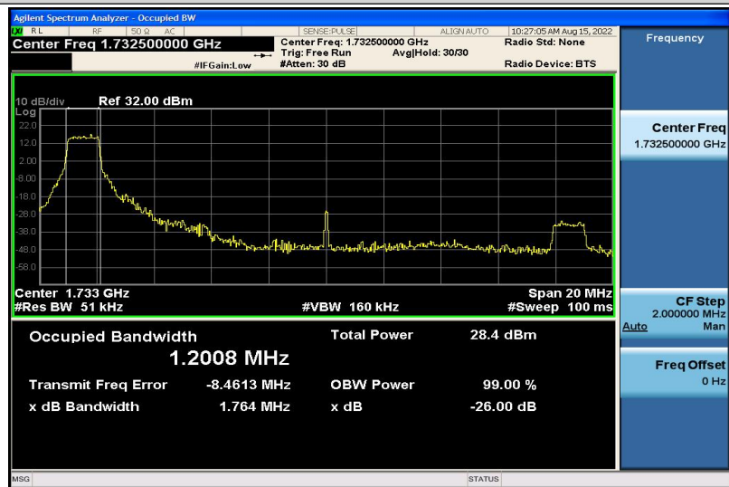
Band4-20MHz-16QAM-20175-6RB#0-1.2008
