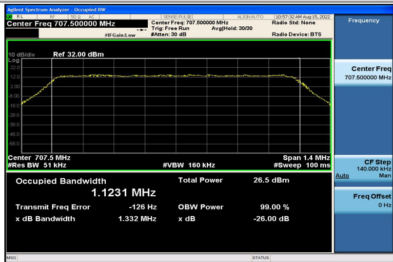
Band12-1.4MHz-QPSK-23095-6RB#0-1.1231
