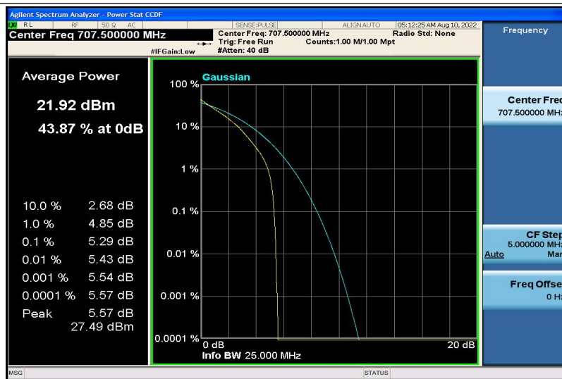
Band12-3MHz-QPSK-23095-6RB#0
