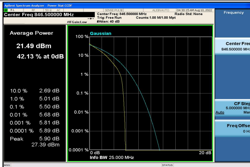
Band5-5MHz-QPSK-20625-6RB#0
