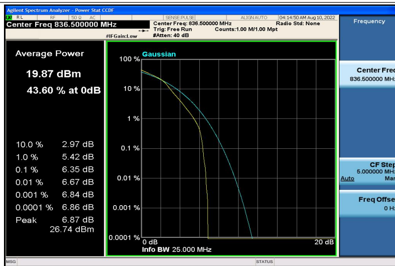
Band5-3MHz-16QAM-20525-6RB#0
