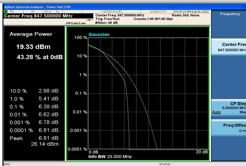
Band5-3MHz-16QAM-20635-6RB#0
