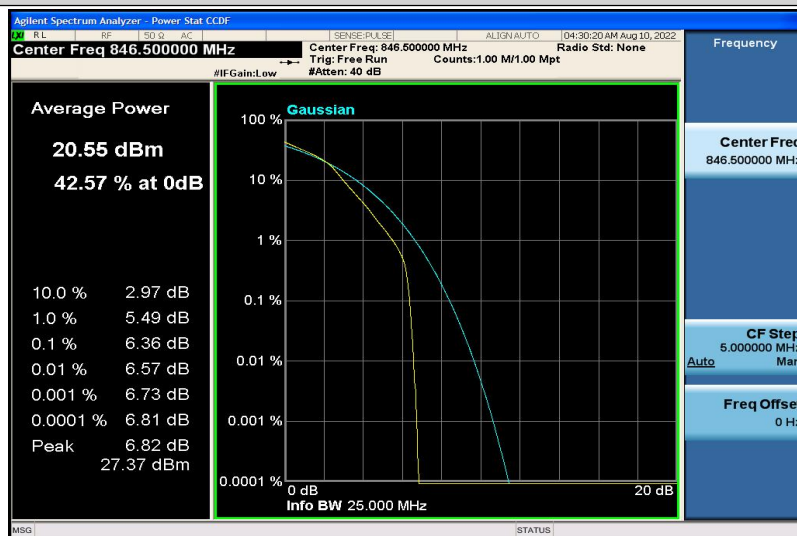
Band5-5MHz-16QAM-20625-6RB#0
