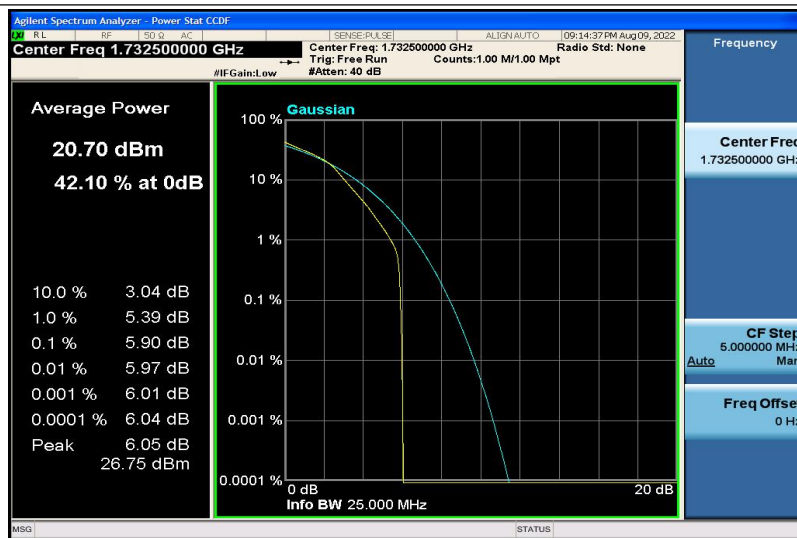
Band4-20MHz-16QAM-20175-6RB#0
