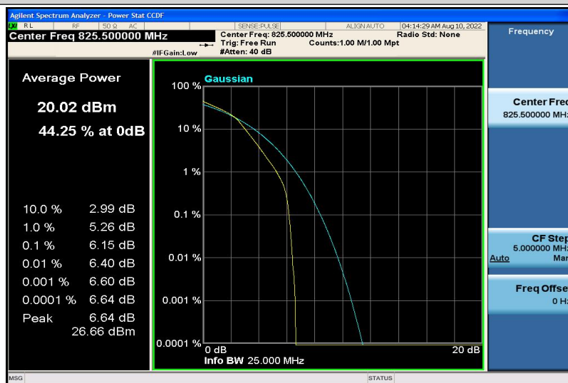
Band5-3MHz-16QAM-20415-6RB#0
