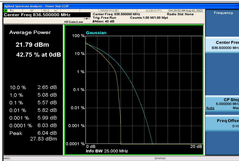
Band5-5MHz-QPSK-20525-6RB#0
