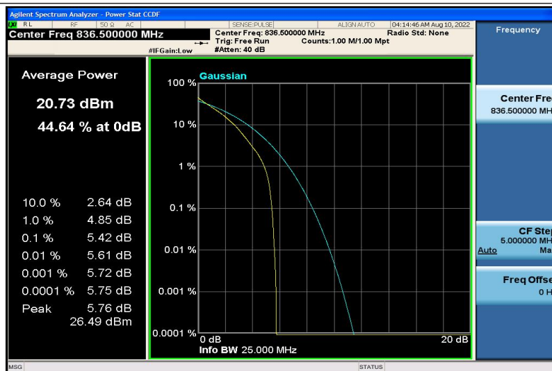
Band5-3MHz-QPSK-20525-6RB#0
