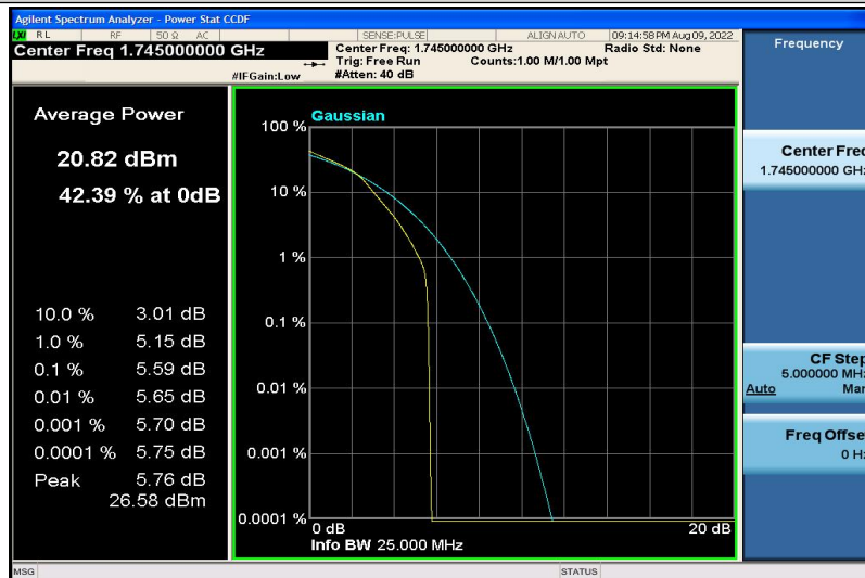
Band4-20MHz-16QAM-20300-6RB#0
