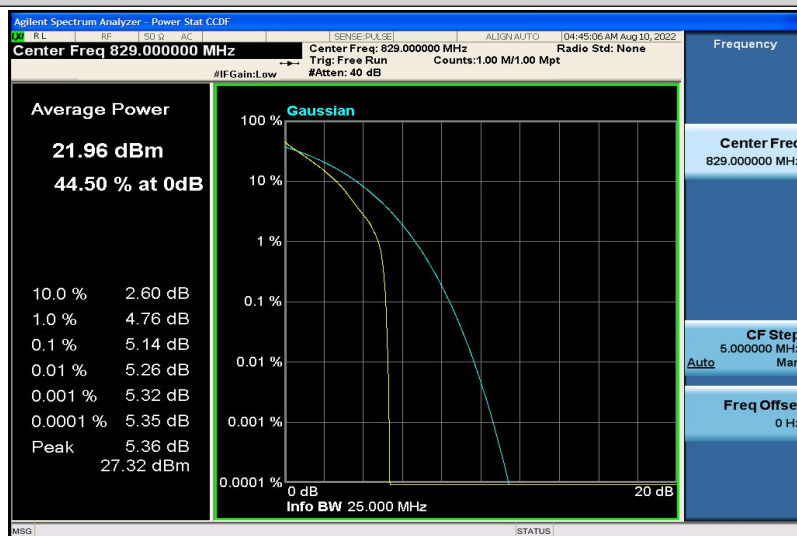
Band5-10MHz-QPSK-20450-6RB#0
