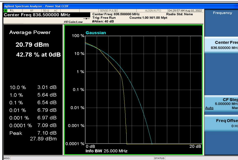
Band5-5MHz-16QAM-20525-6RB#0
