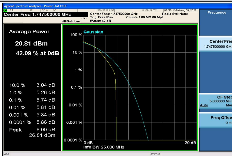
Band4-15MHz-16QAM-20325-6RB#0
