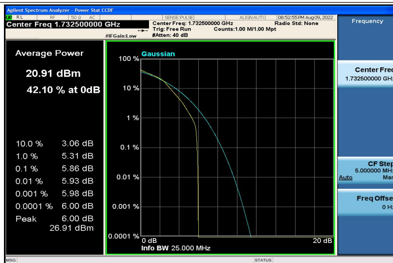
Band4-15MHz-16QAM-20175-6RB#0
