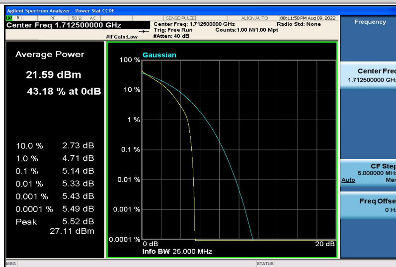
Band4-5MHz-QPSK-19975-6RB#0
