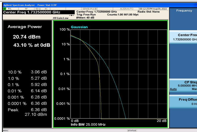
Band4-5MHz-16QAM-20175-6RB#0
