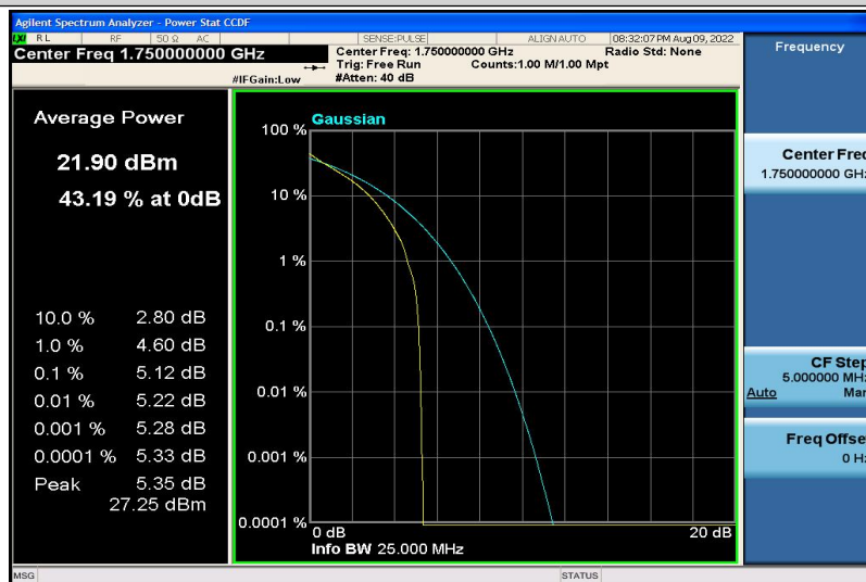
Band4-10MHz-QPSK-20350-6RB#0
