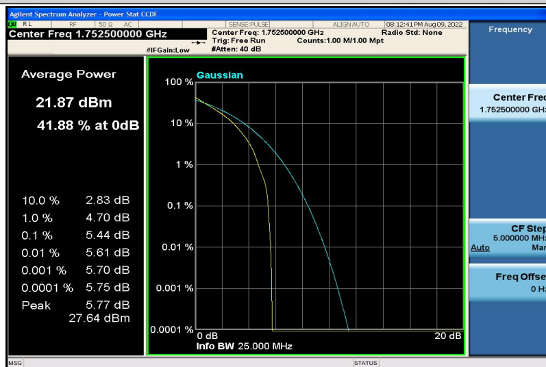
Band4-5MHz-QPSK-20375-6RB#0
