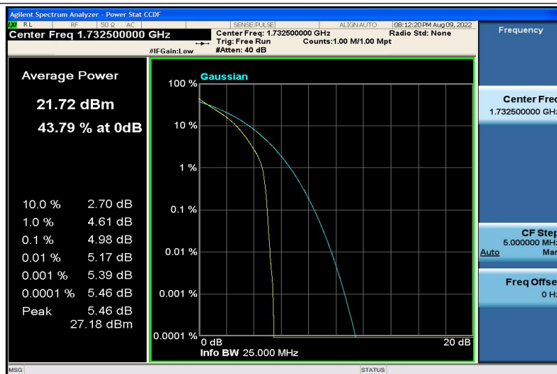
Band4-5MHz-QPSK-20175-6RB#0
