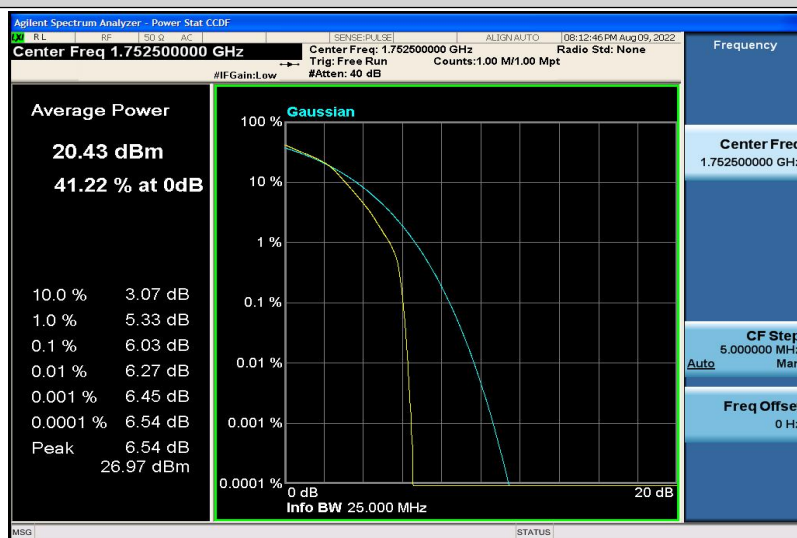
Band4-5MHz-16QAM-20375-6RB#0
