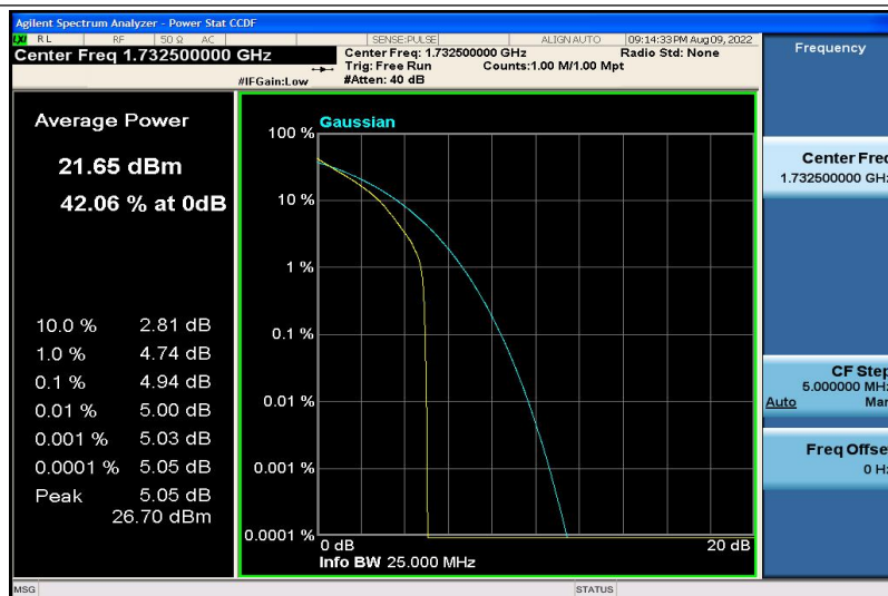
Band4-20MHz-QPSK-20175-6RB#0
