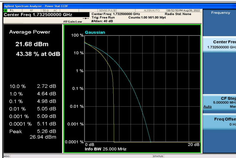
Band4-15MHz-QPSK-20175-6RB#0
