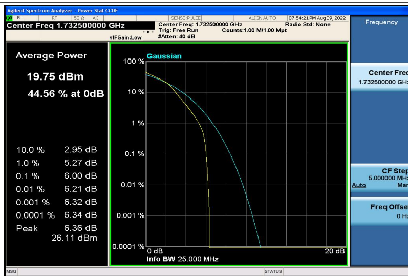
Band4-3MHz-16QAM-20175-6RB#0
