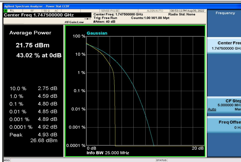
Band4-15MHz-QPSK-20325-6RB#0
