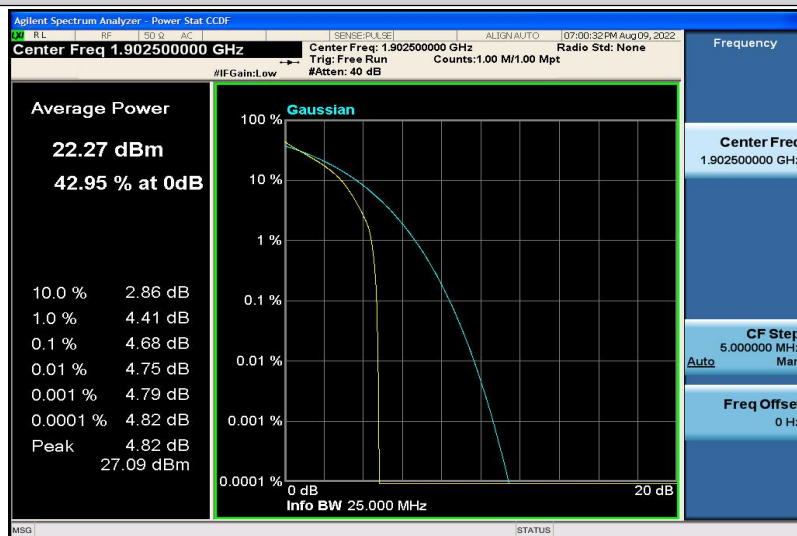
Band2-15MHz-QPSK-19125-6RB#0
