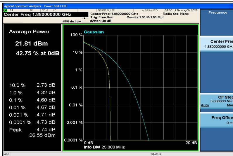
Band2-15MHz-QPSK-18900-6RB#0
