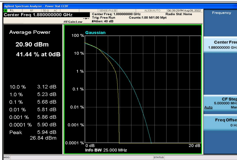
Band2-10MHz-16QAM-18900-6RB#0
