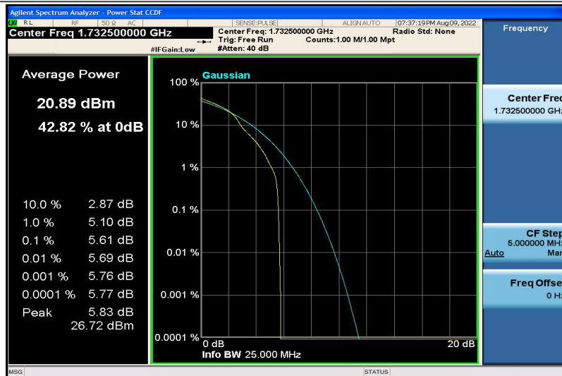
Band4-1.4MHz-16QAM-20175-1RB#0
