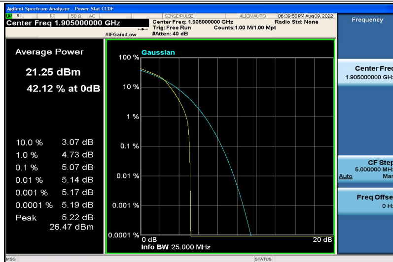
Band2-10MHz-16QAM-19150-6RB#0
