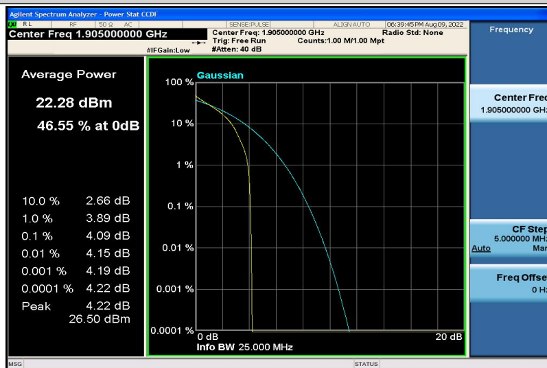
Band2-10MHz-QPSK-19150-6RB#0
