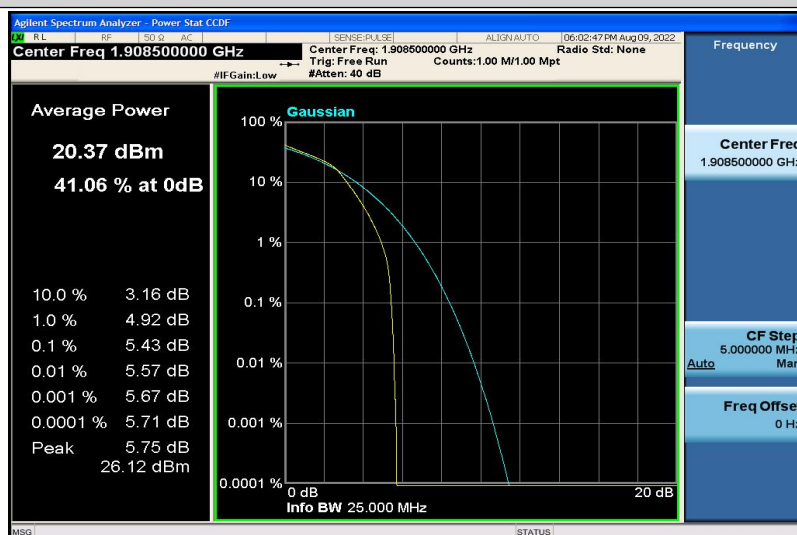
Band2-3MHz-16QAM-19185-6RB#0
