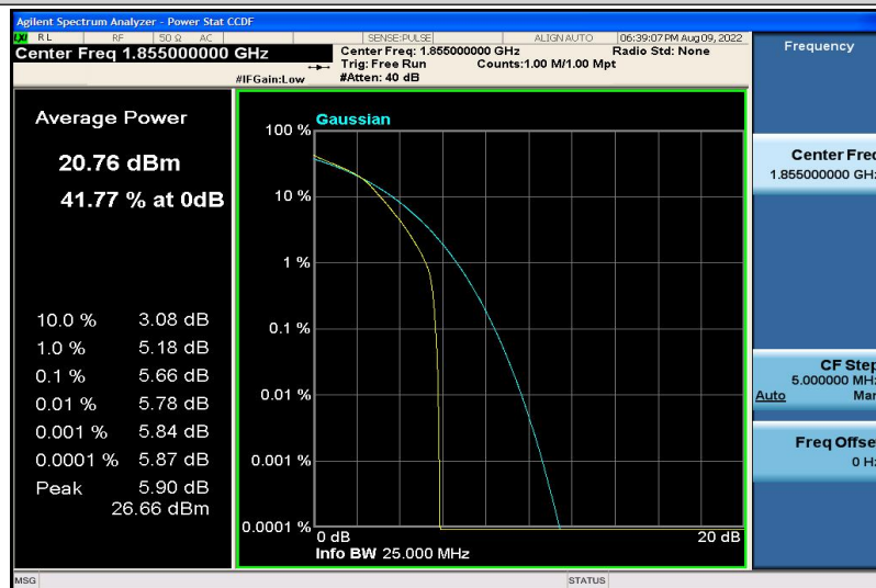
Band2-10MHz-16QAM-18650-6RB#0
