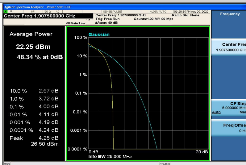
Band2-5MHz-QPSK-19175-6RB#0
