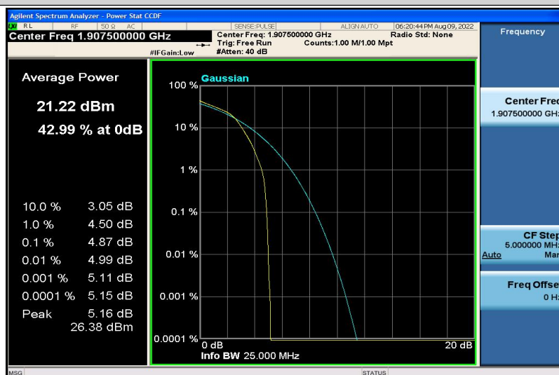
Band2-5MHz-16QAM-19175-6RB#0
