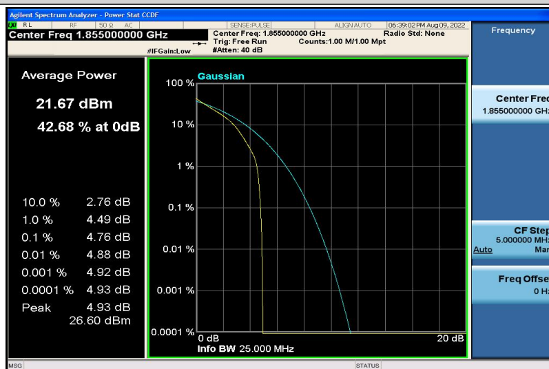
Band2-10MHz-QPSK-18650-6RB#0
