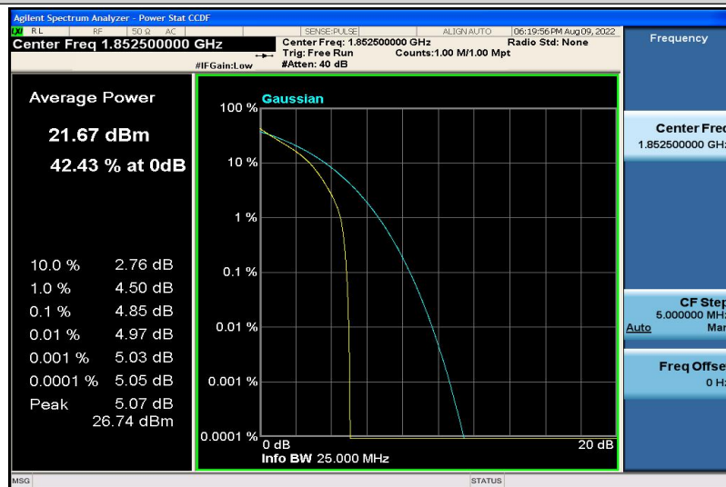
Band2-5MHz-QPSK-18625-6RB#0
